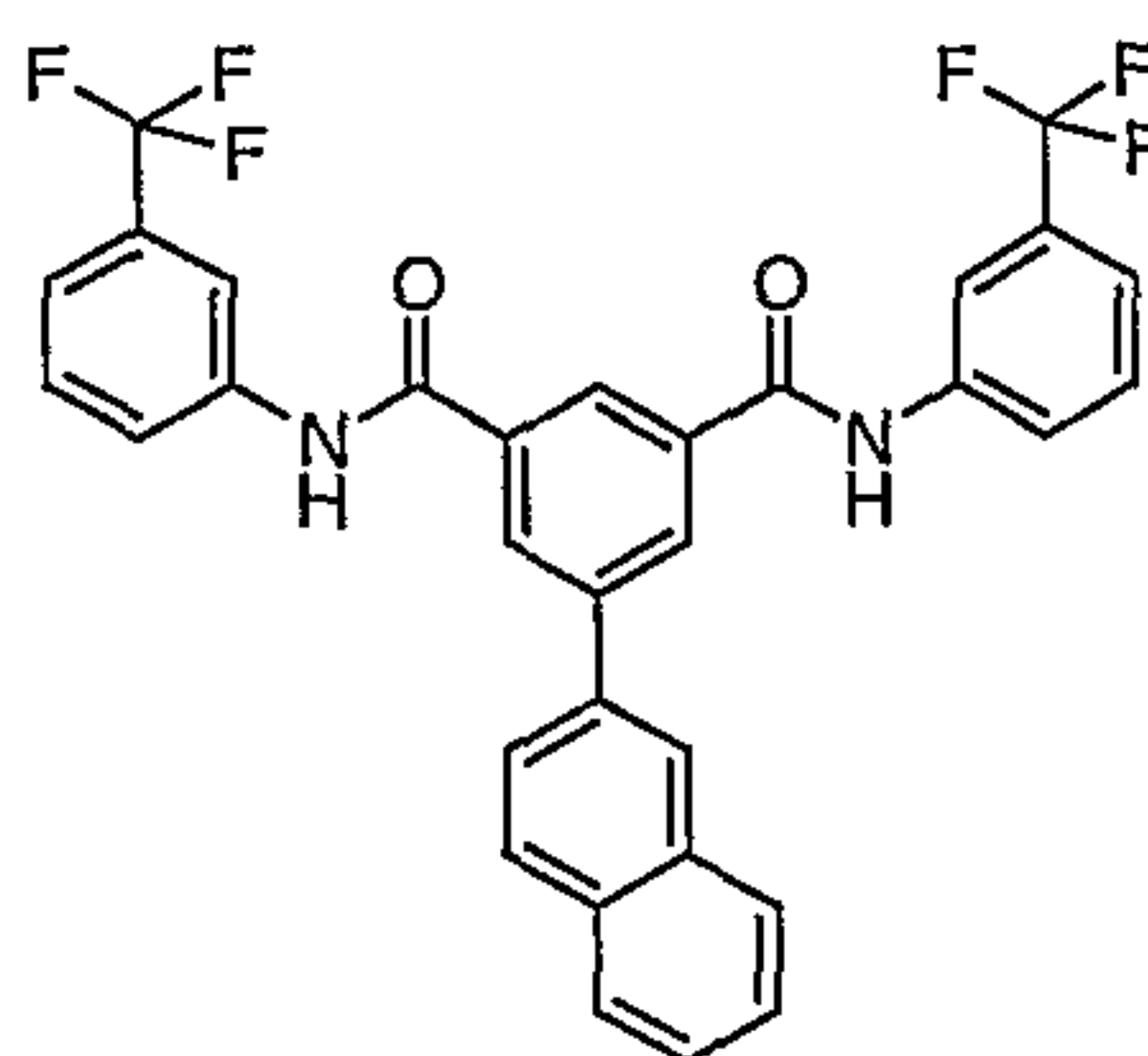
Compound # 18
