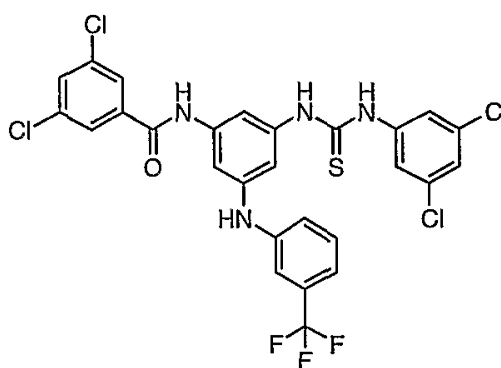
Compound # 10
