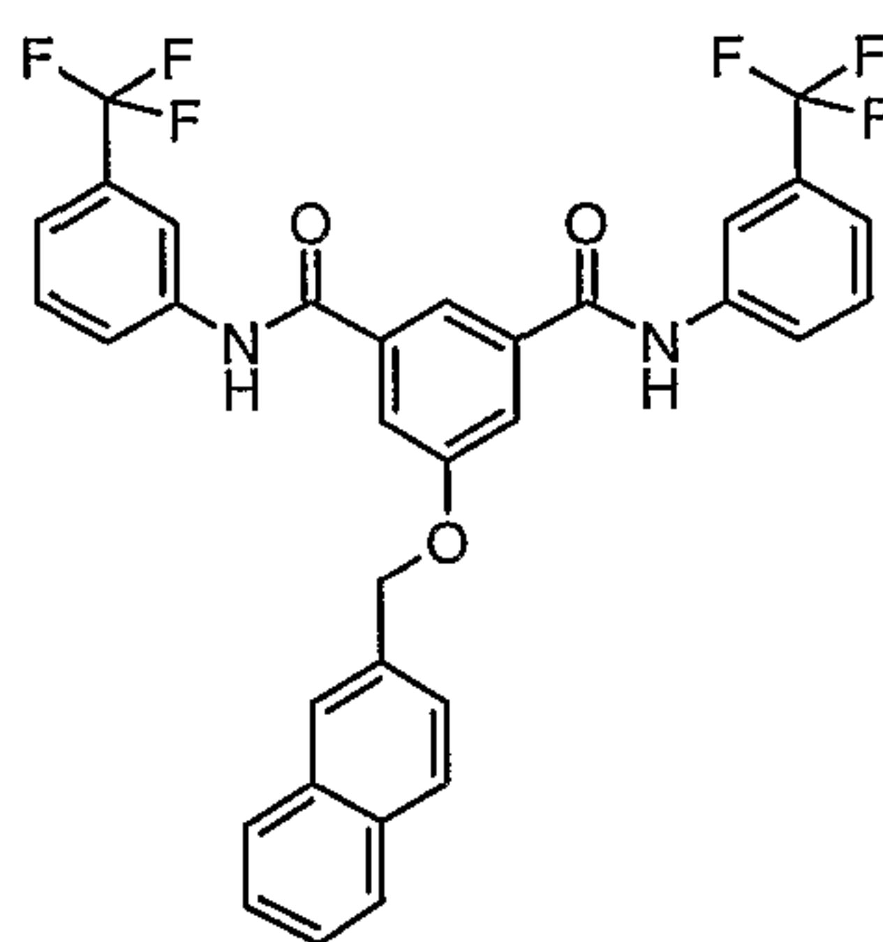
Compound # 42
