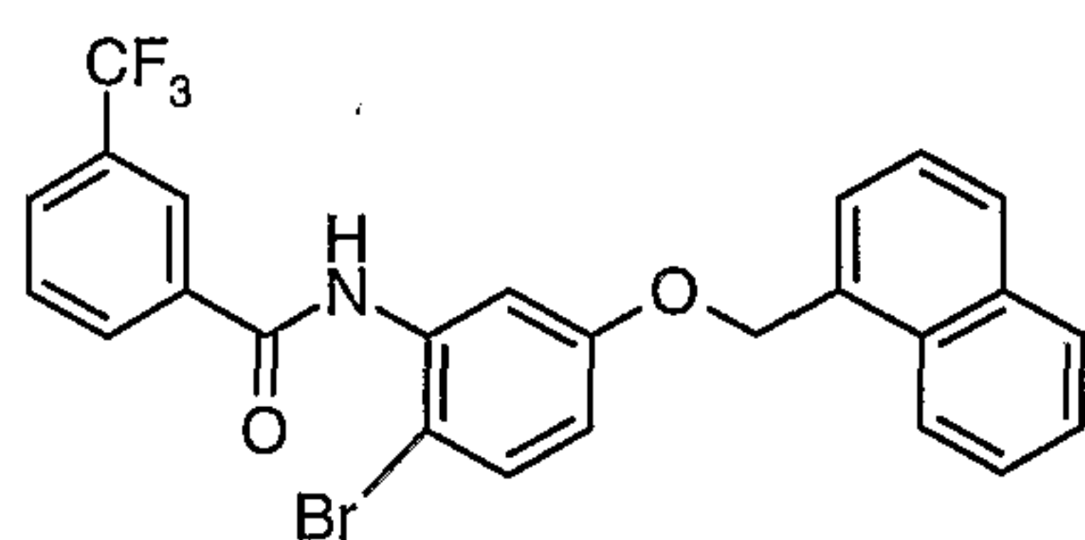
Compound # 34
