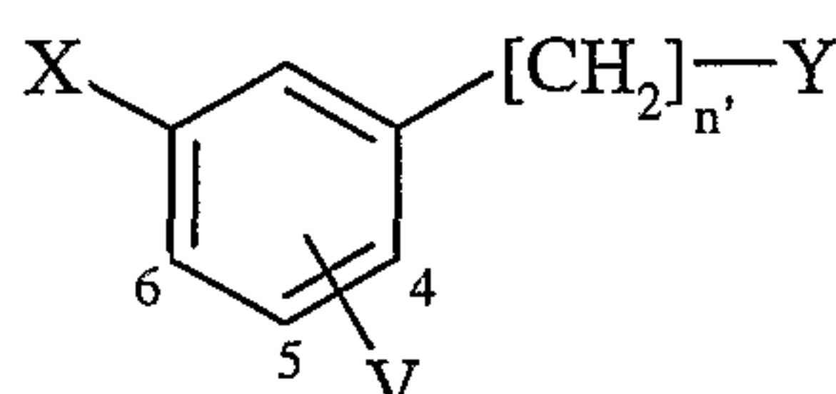
Formula 1
