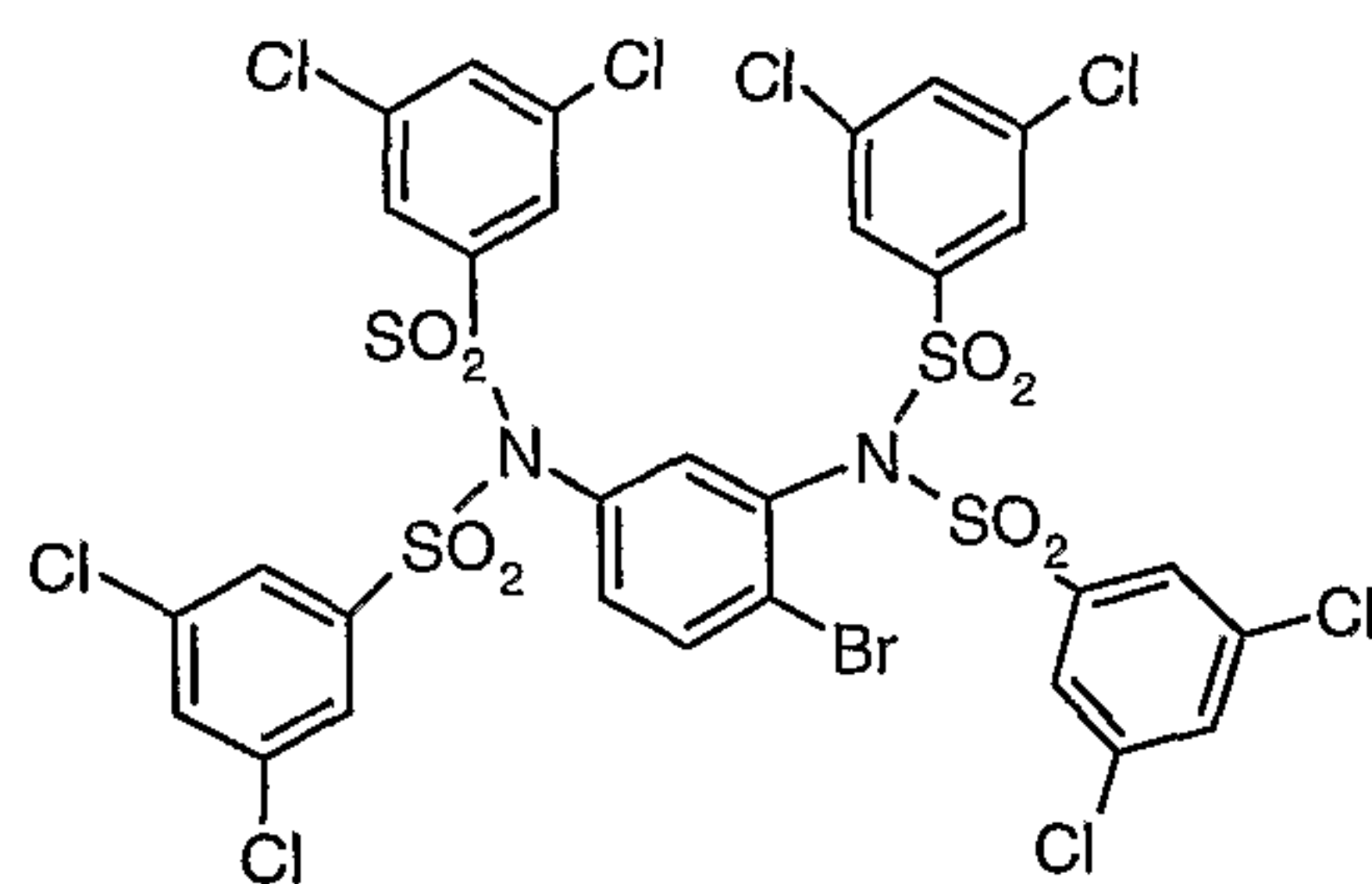
Compound # 30
