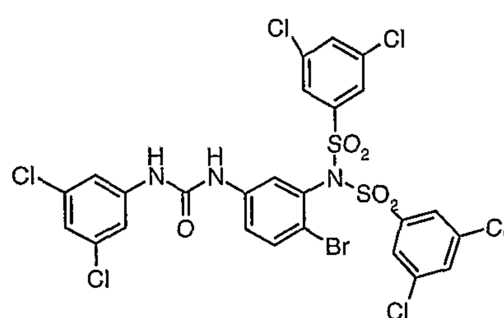
Compound # 29
