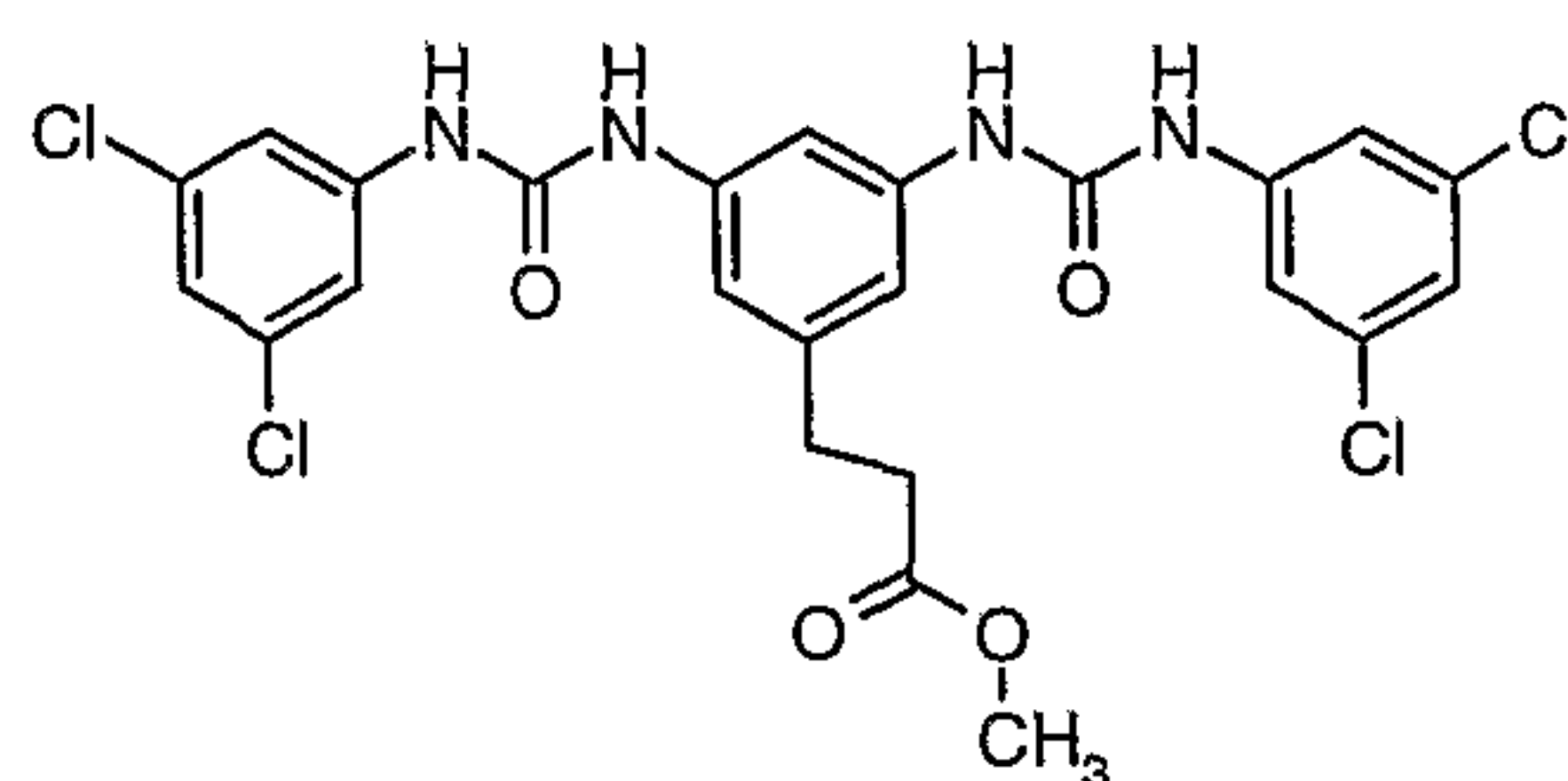
Compound # 1
