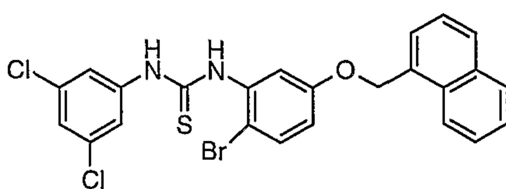
Compound # 33
