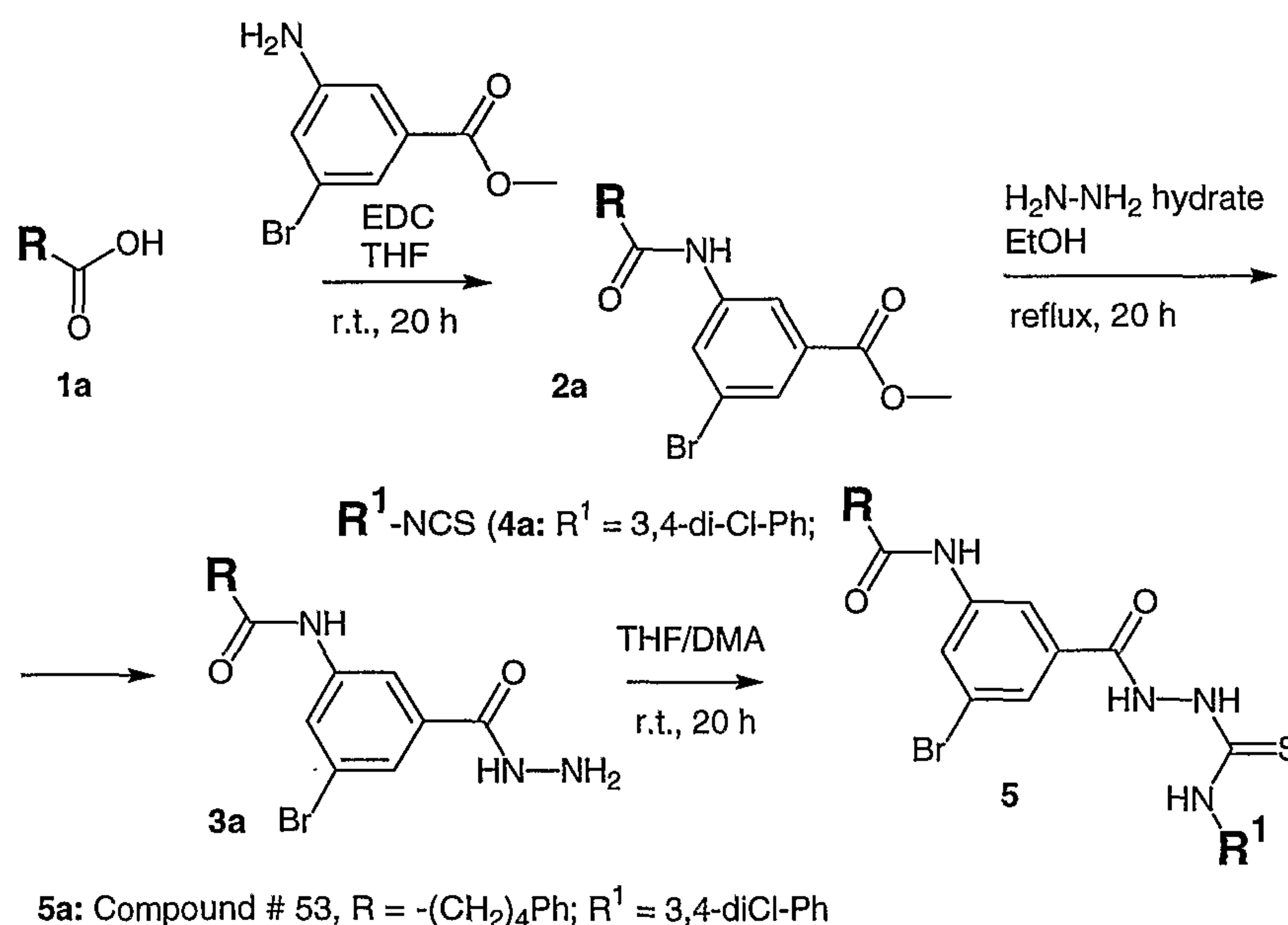
Scheme XIV
