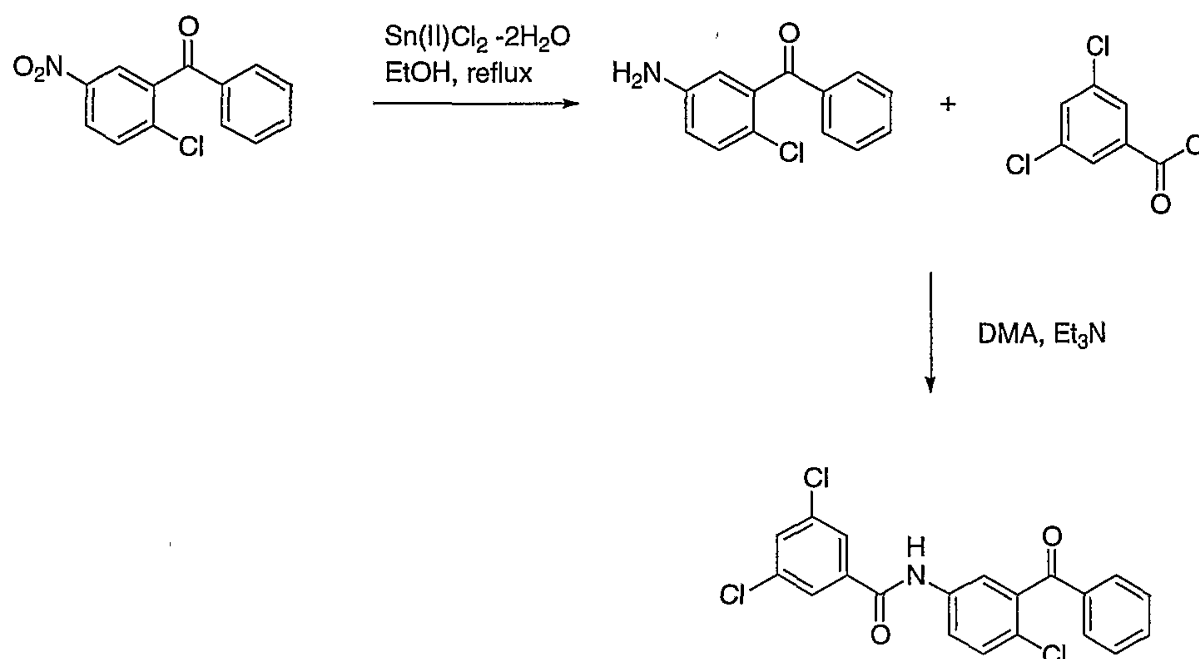
Scheme XI
