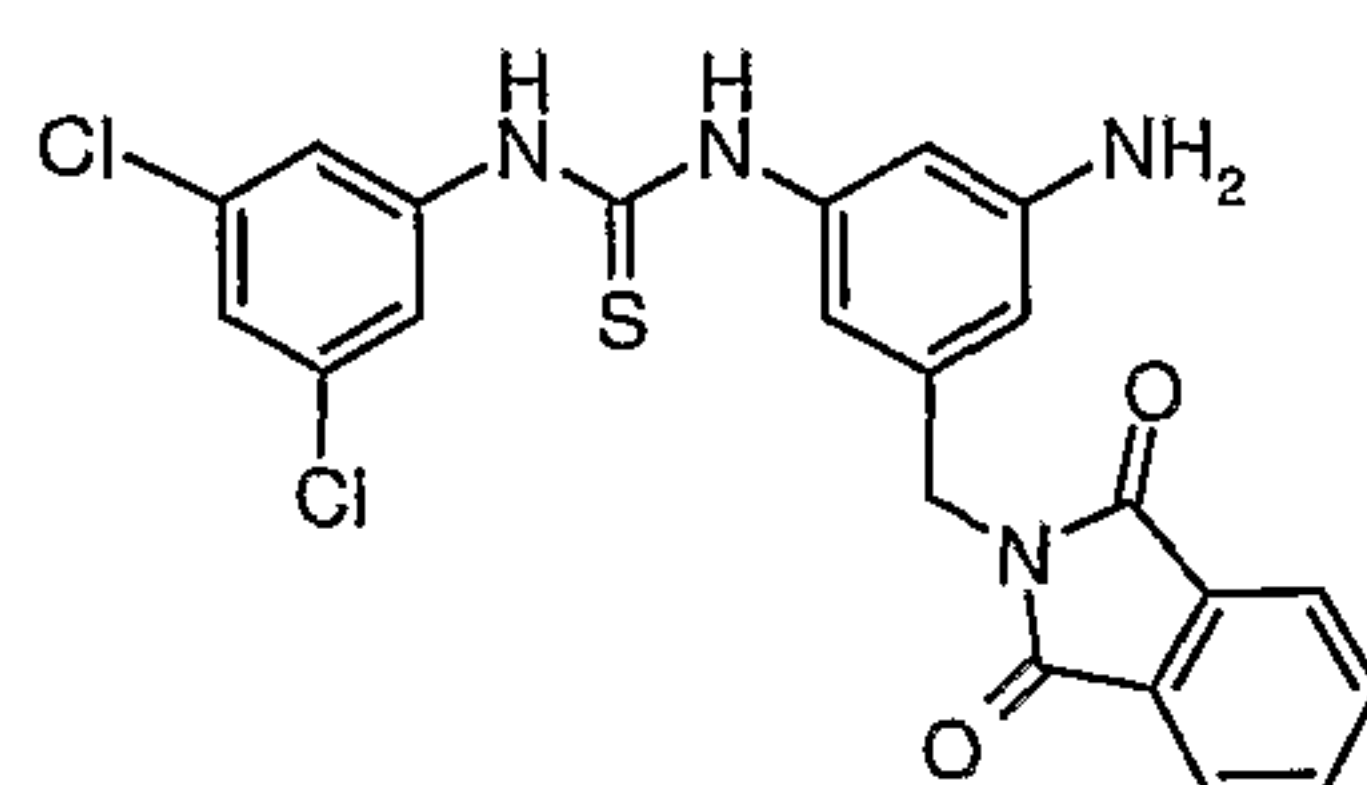
Compound # 31
