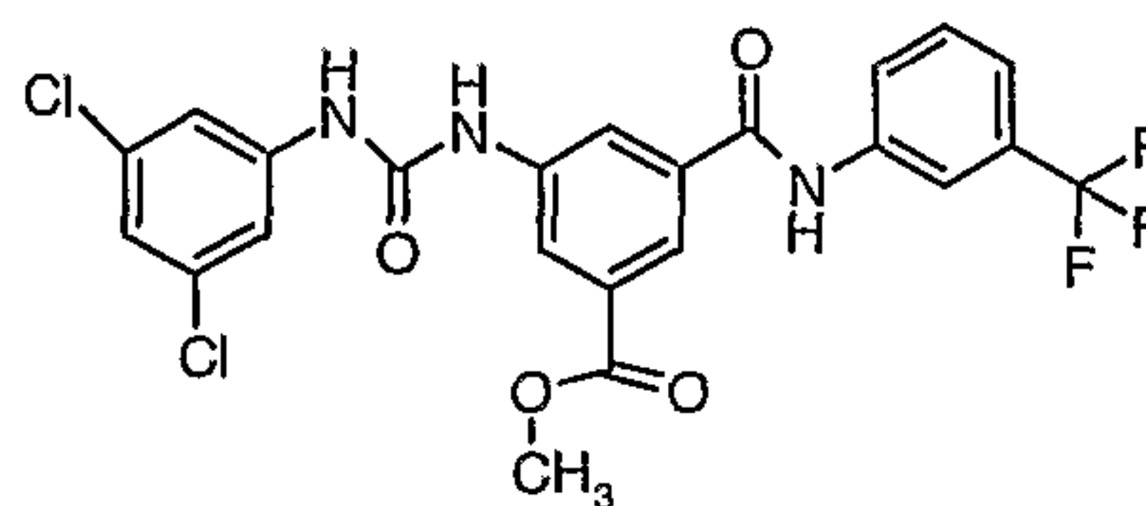
Compound # 6
