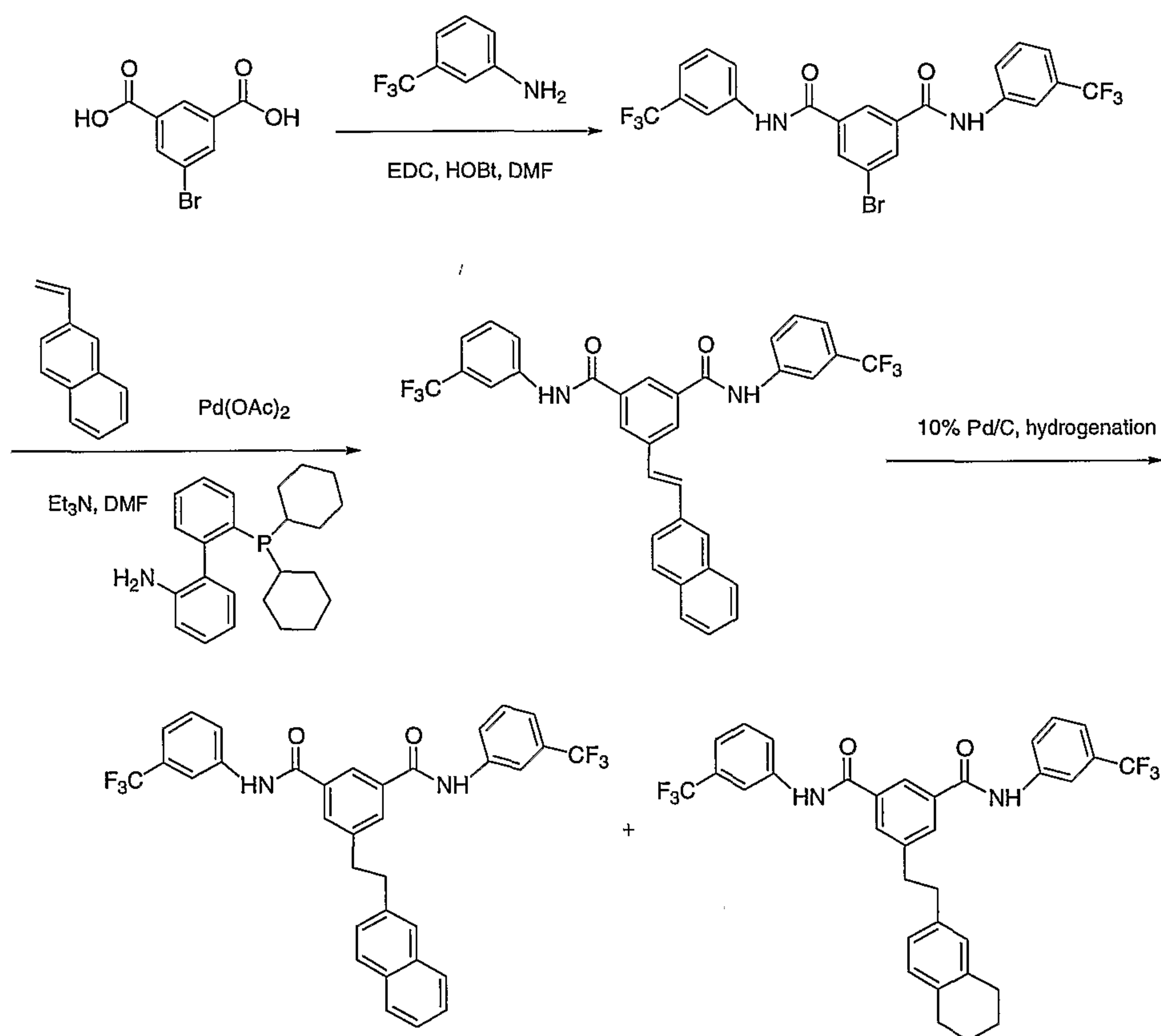
Scheme I-F
