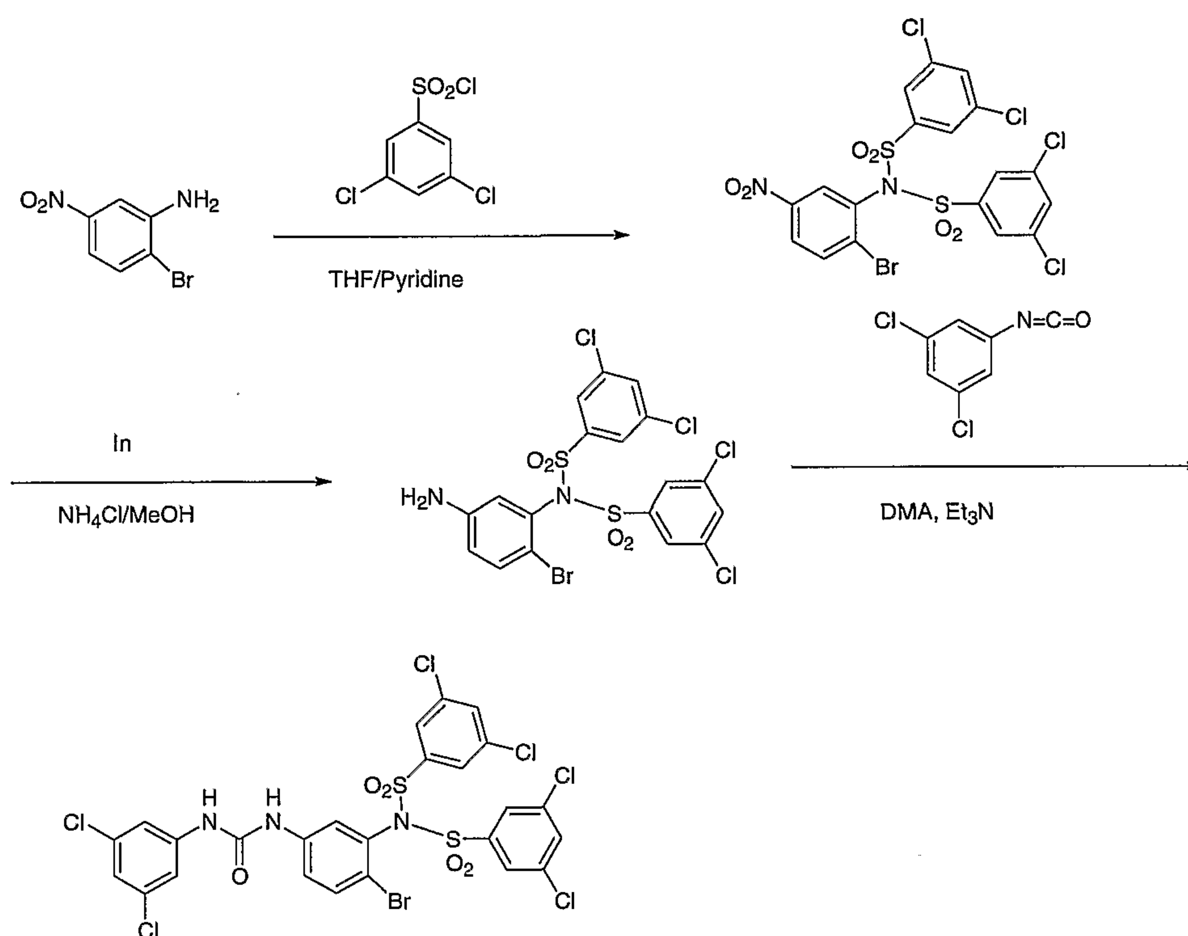
Scheme IV-C
