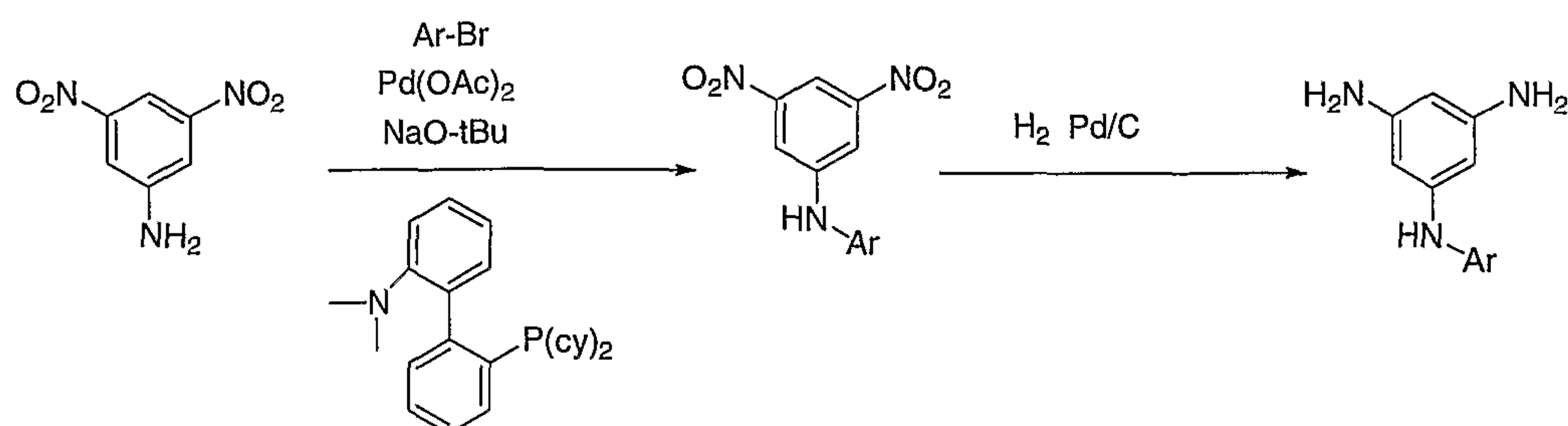
Scheme II-B
