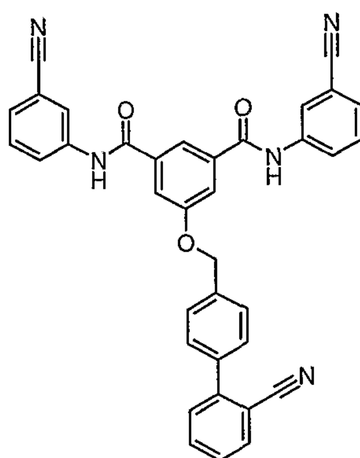
Compound # 22
