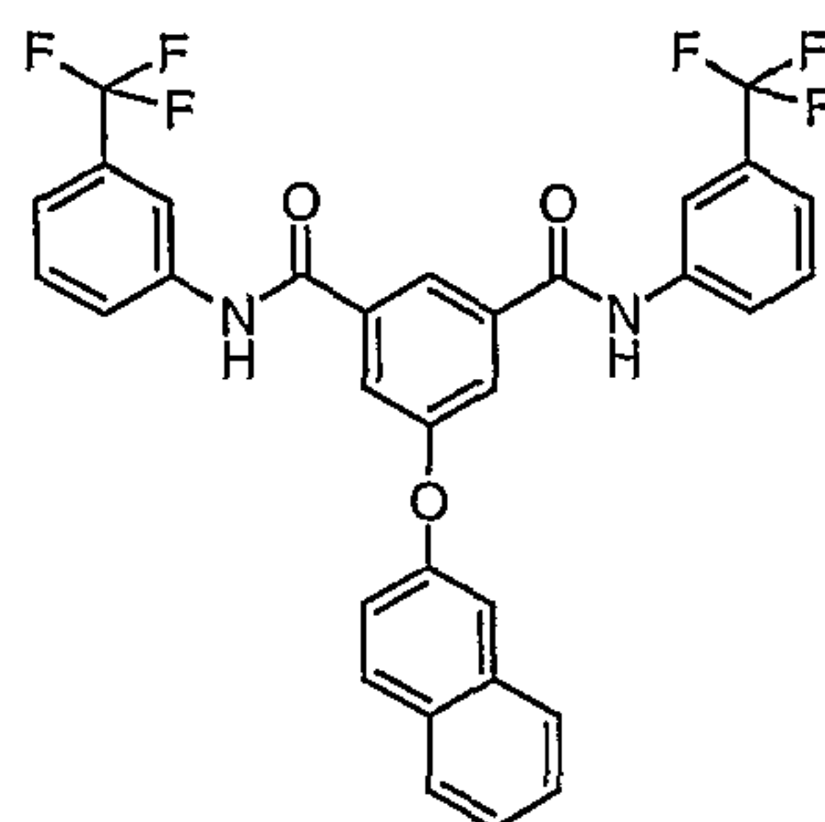
Compound # 17
