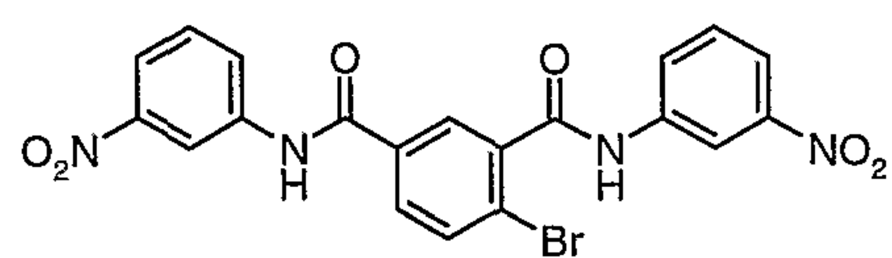
Compound # 41
