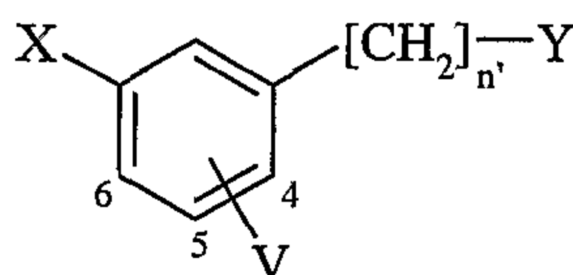
Formula 1
