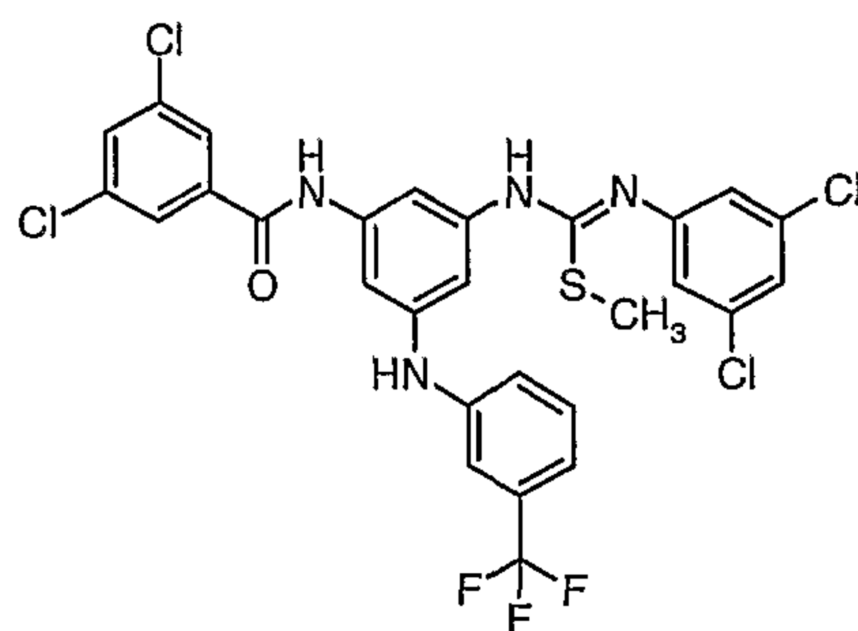
Compound # 9
