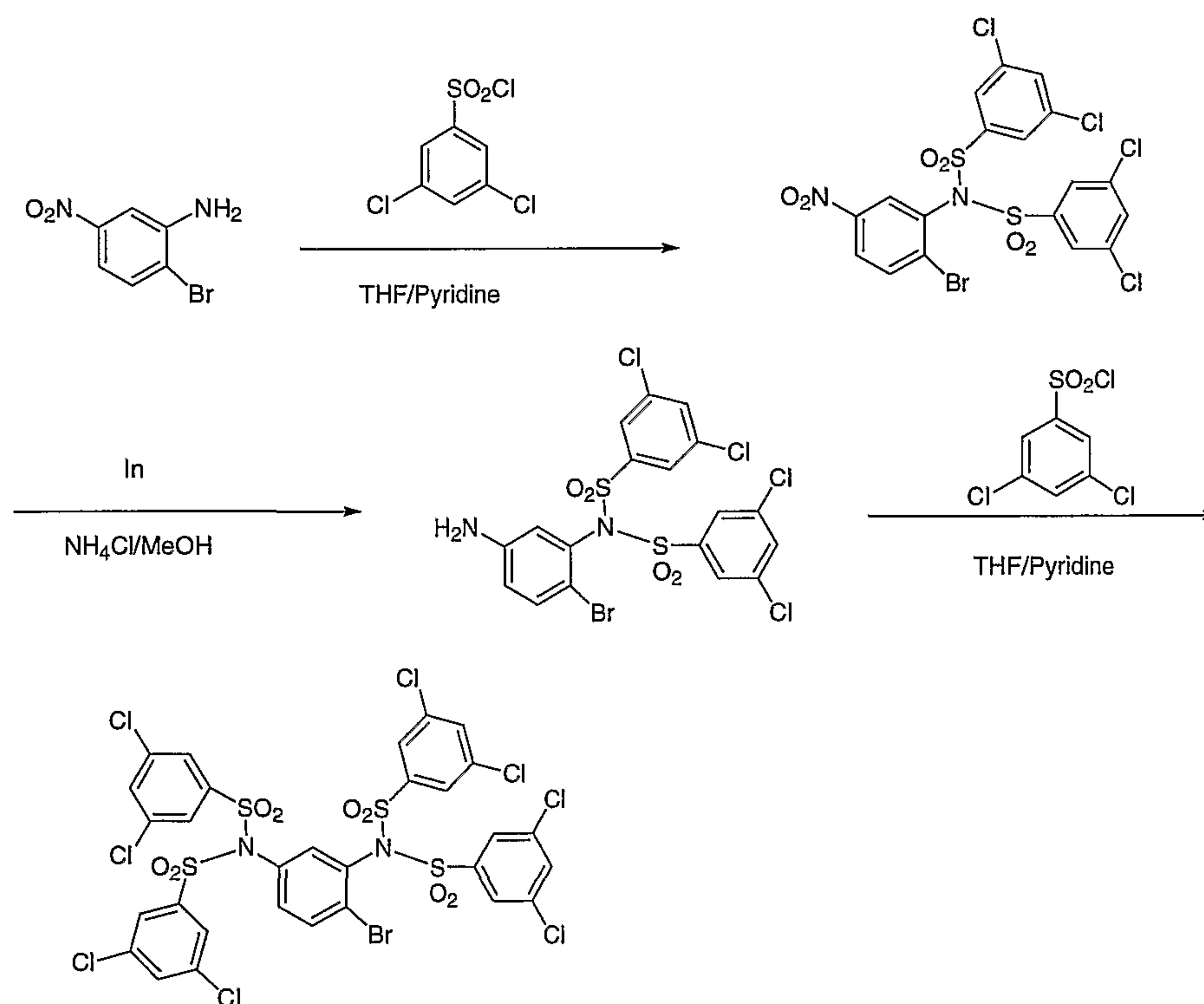
Scheme IV-B
