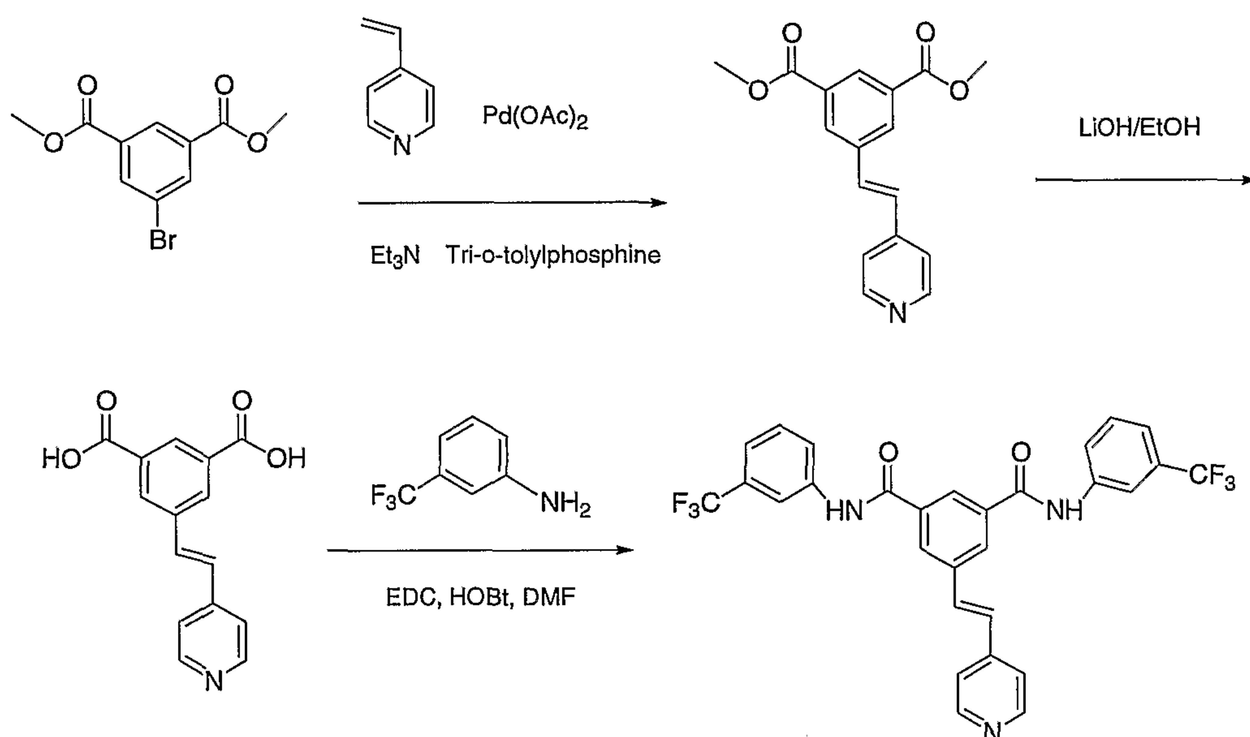
Scheme I-C
