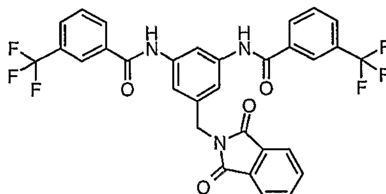
Compound # 12
