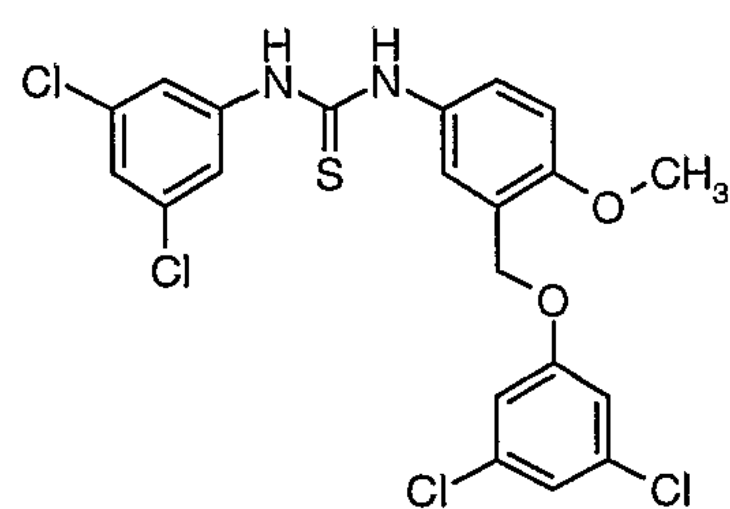
Compound # 45
