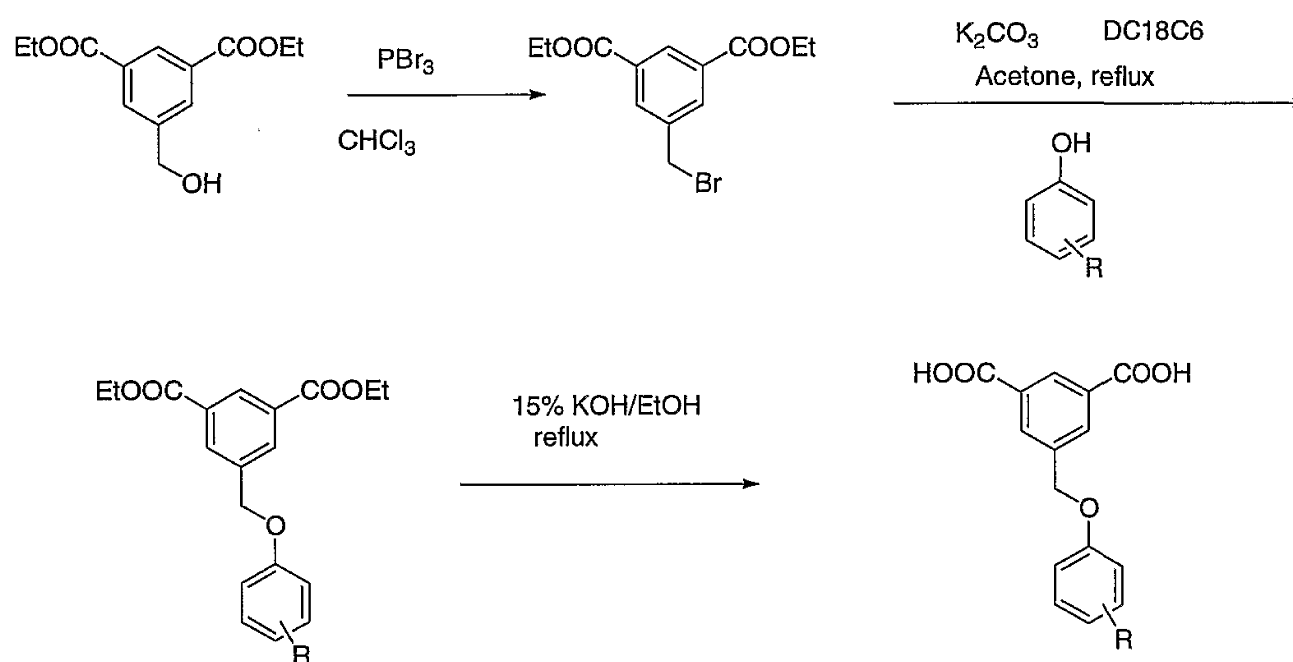
Scheme I-B
