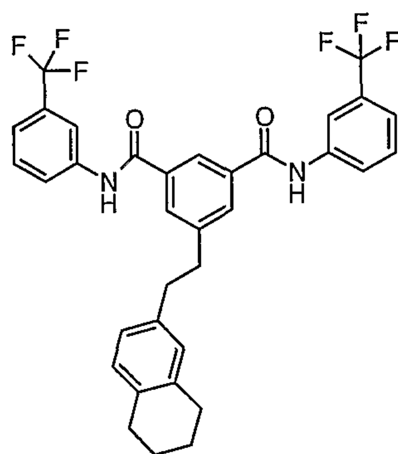
Compound # 23
