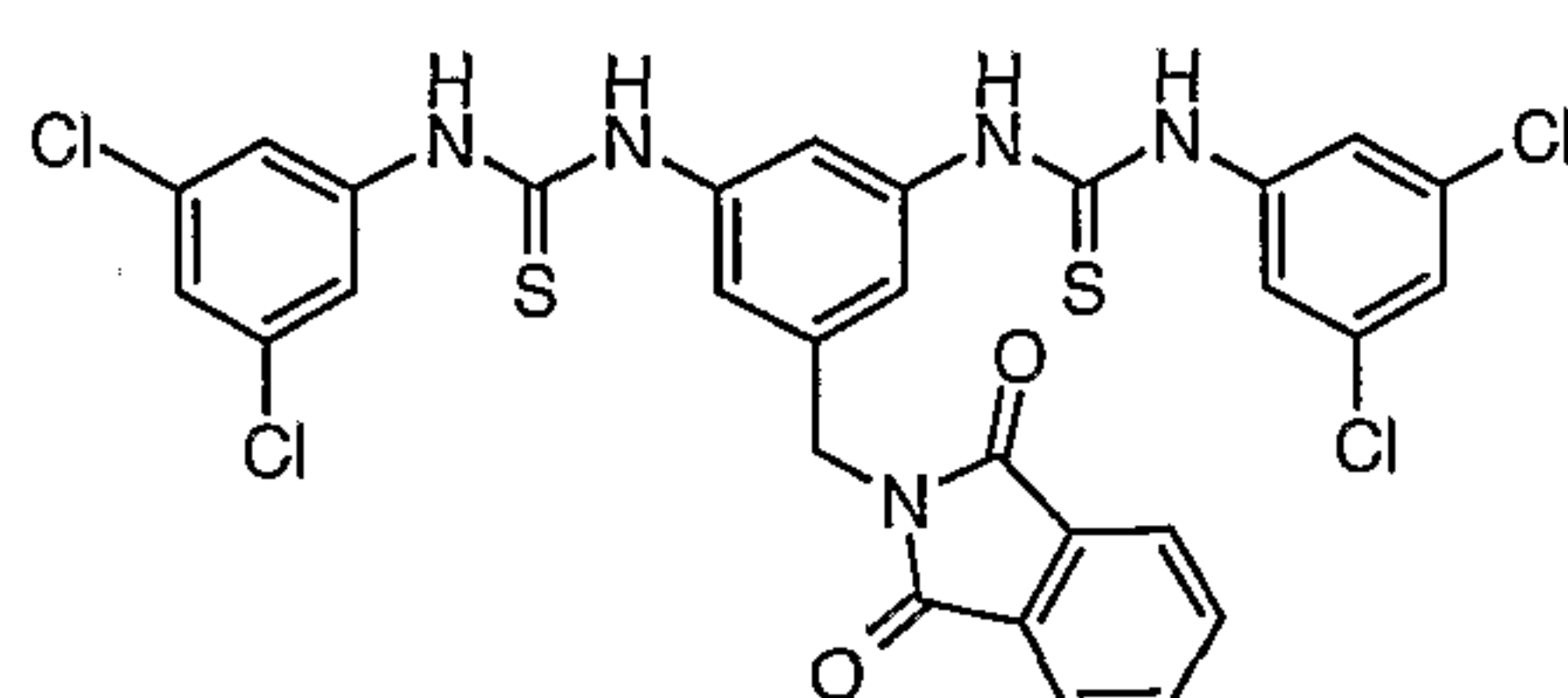
Compound # 27
