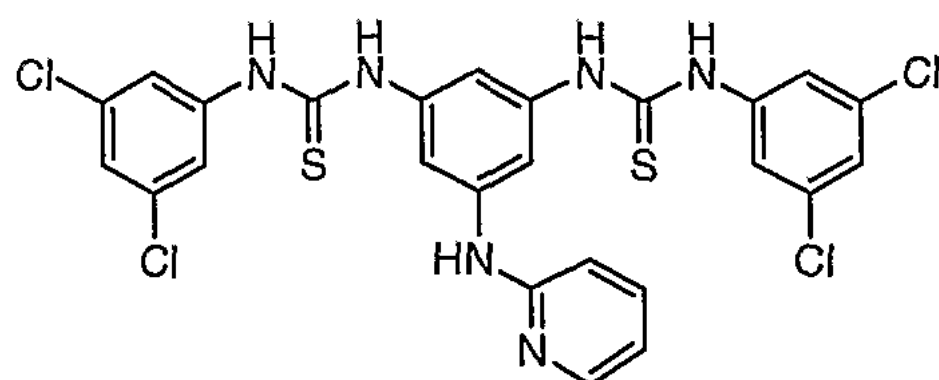
Compound # 13
