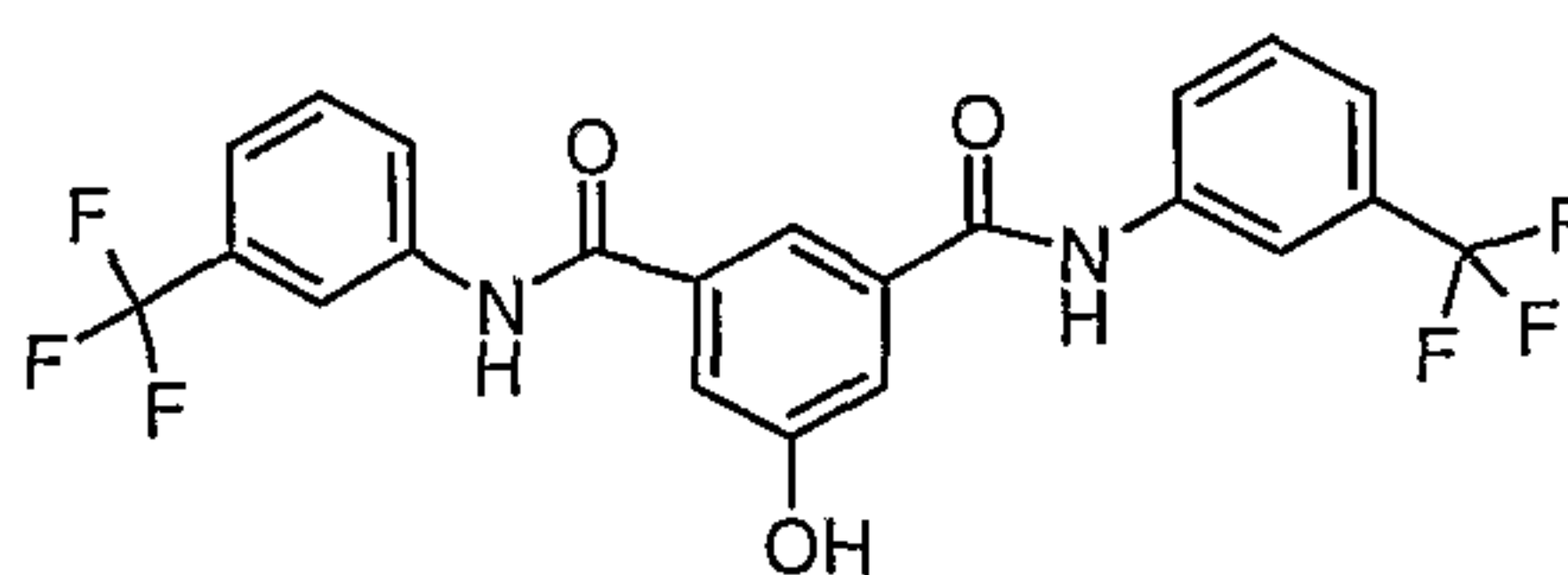
Compound # 2
