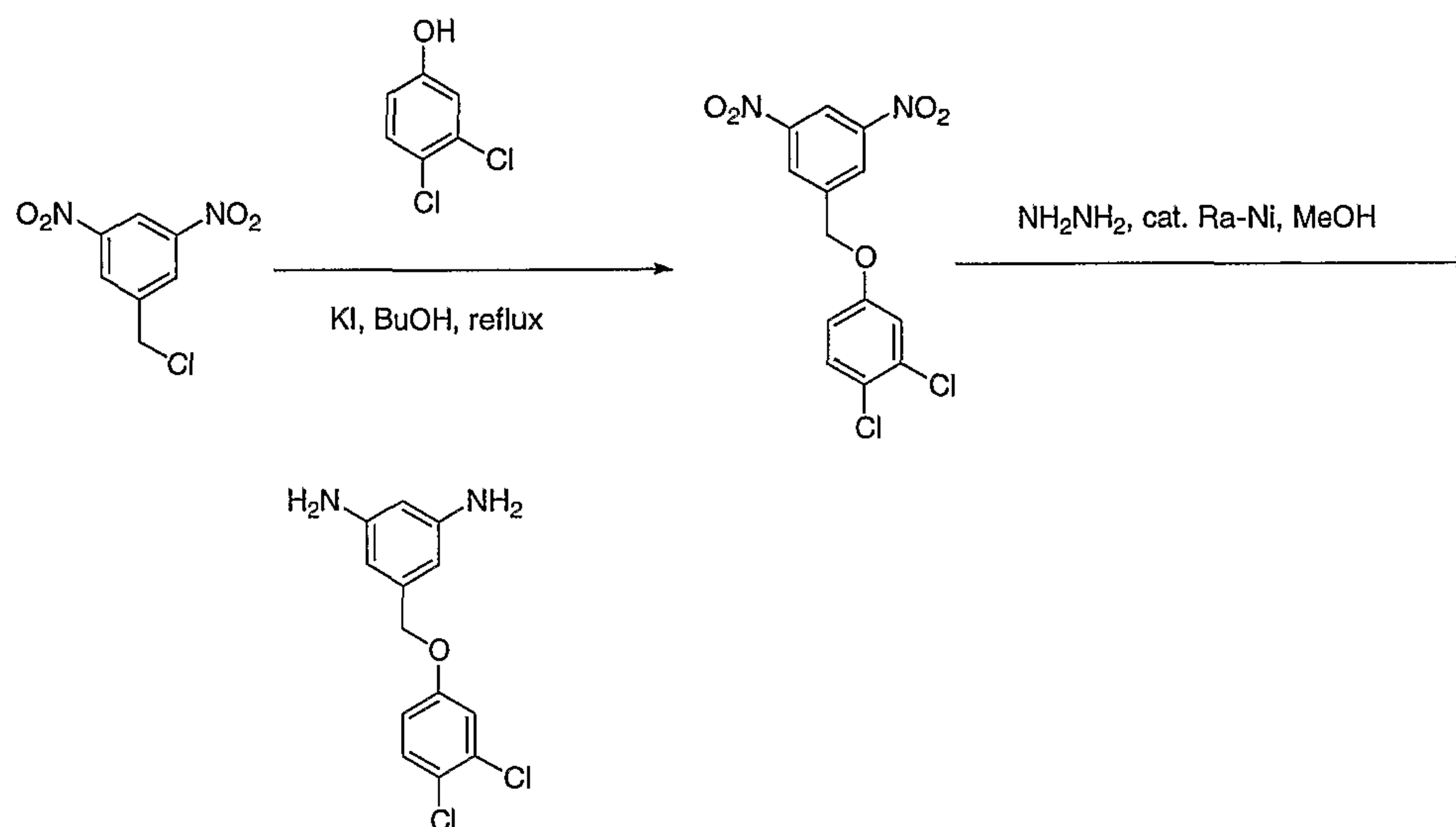
Scheme II-E
