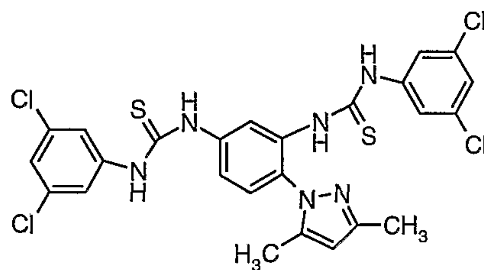
Compound # 39
