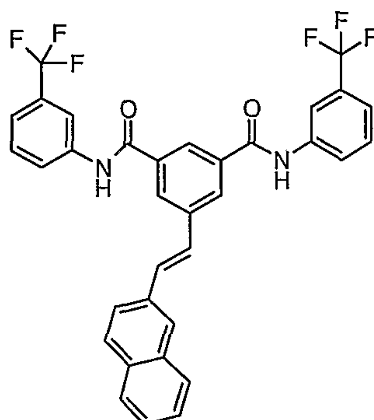
Compound # 25
