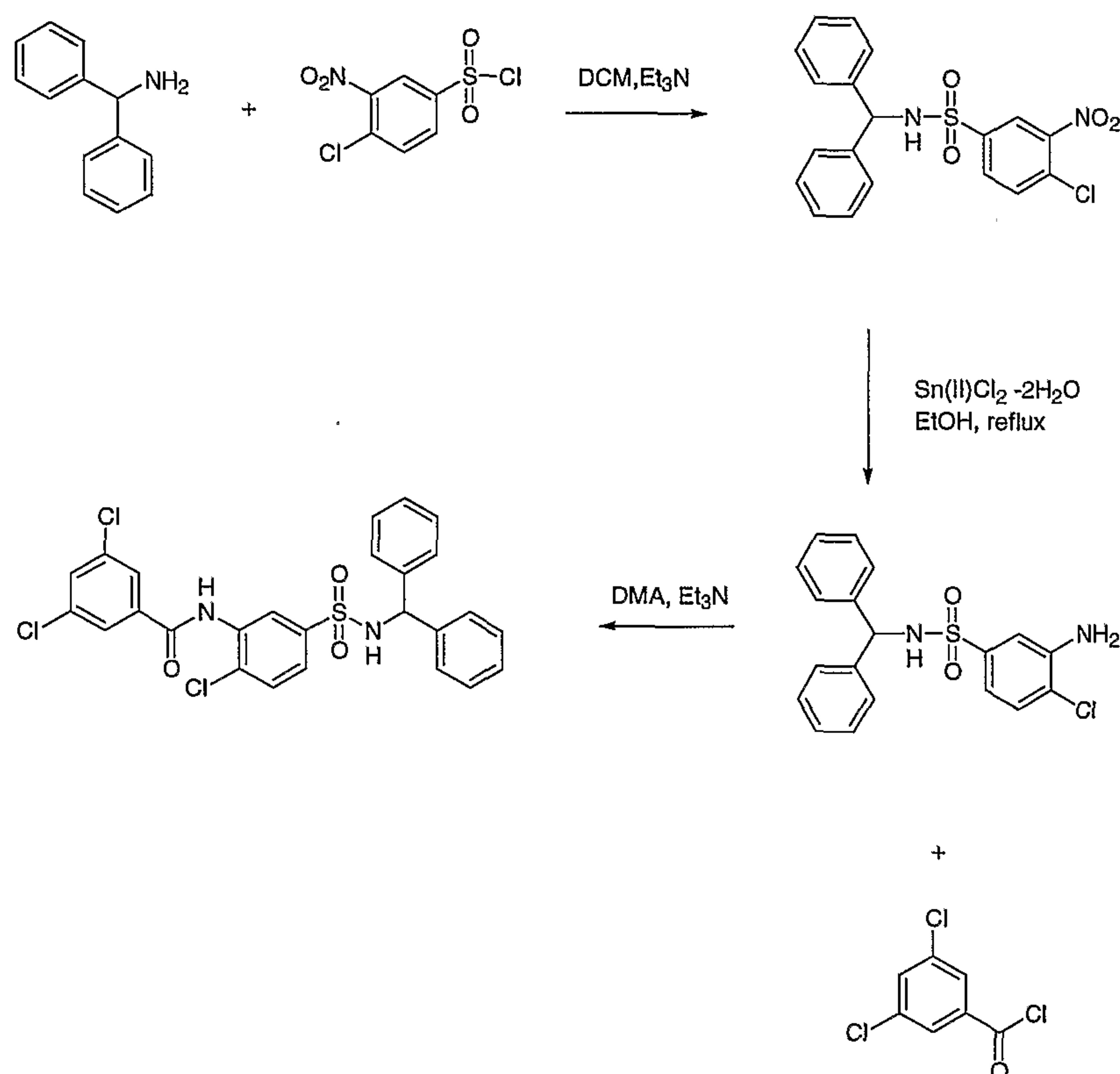
Scheme X
