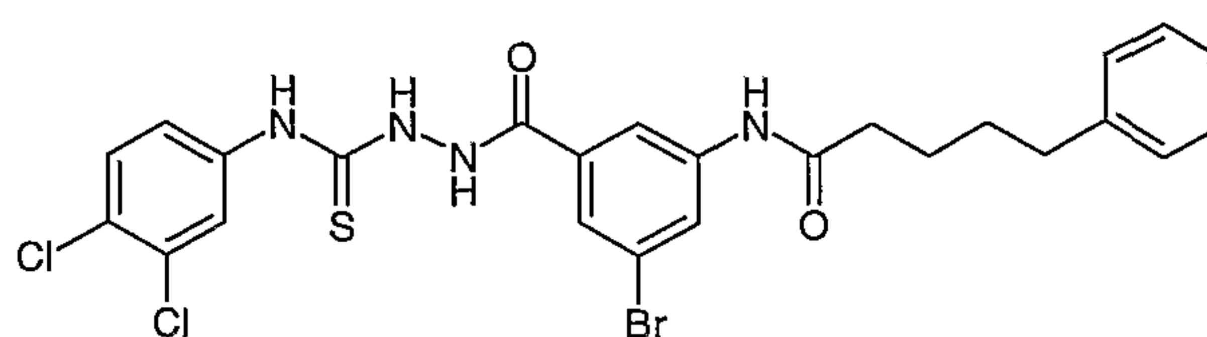
Compound # 53
