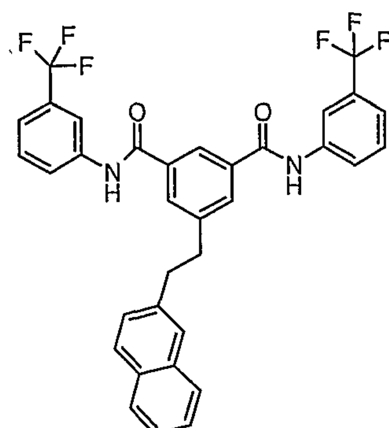
Compound # 24
