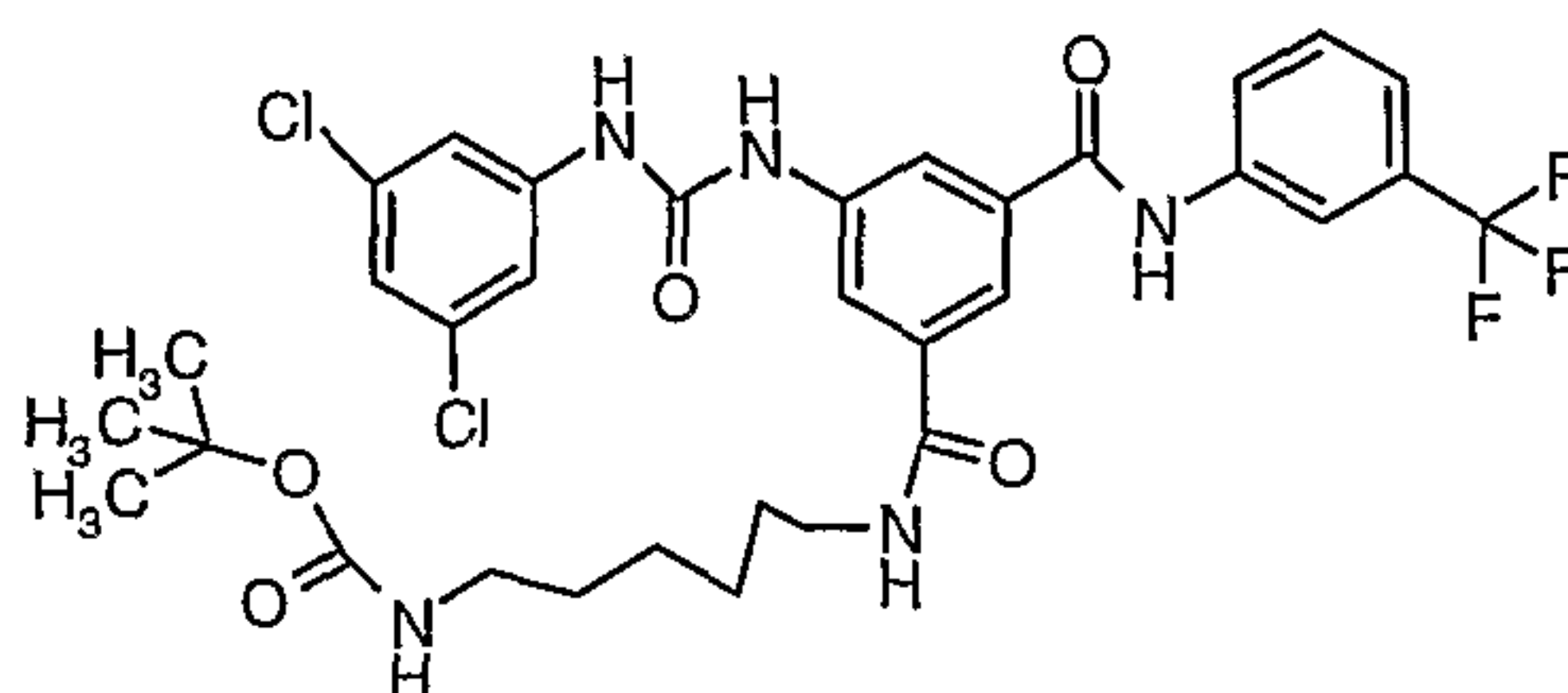
Compound # 4
