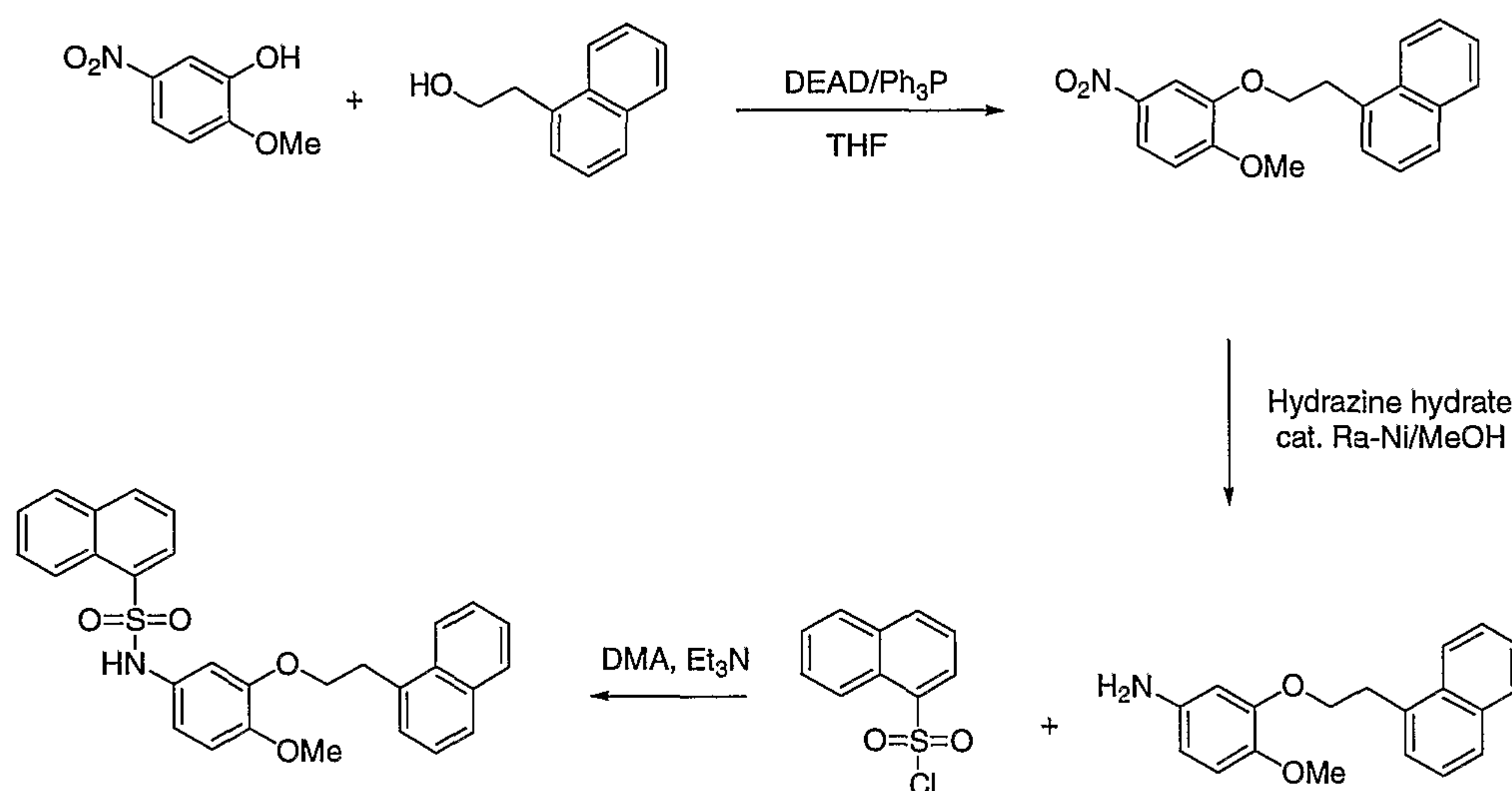
Scheme XII
