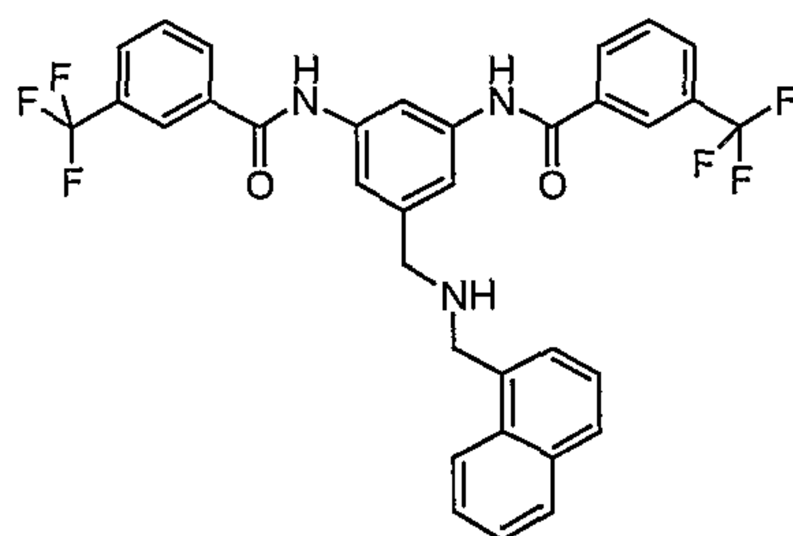
Compound # 14
