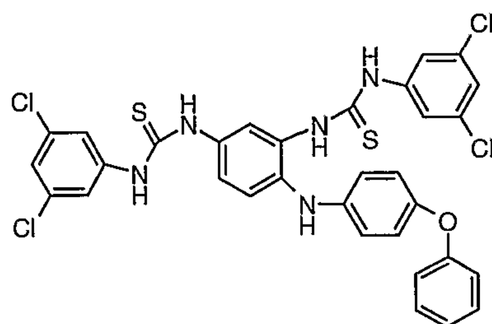
Compound # 40
