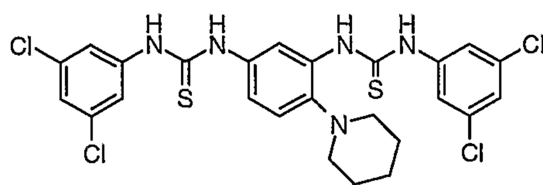
Compound # 44
