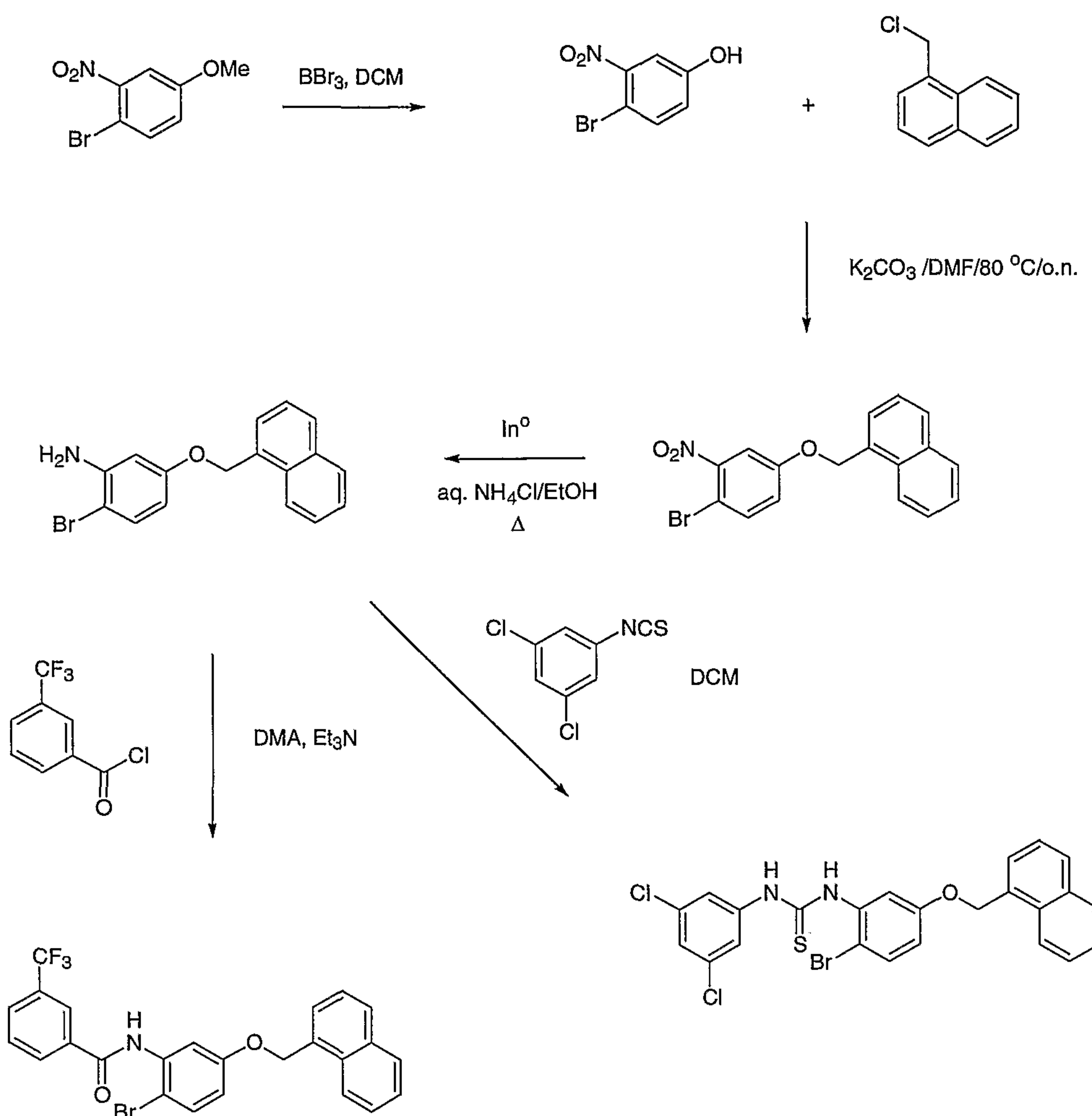
Scheme VII
