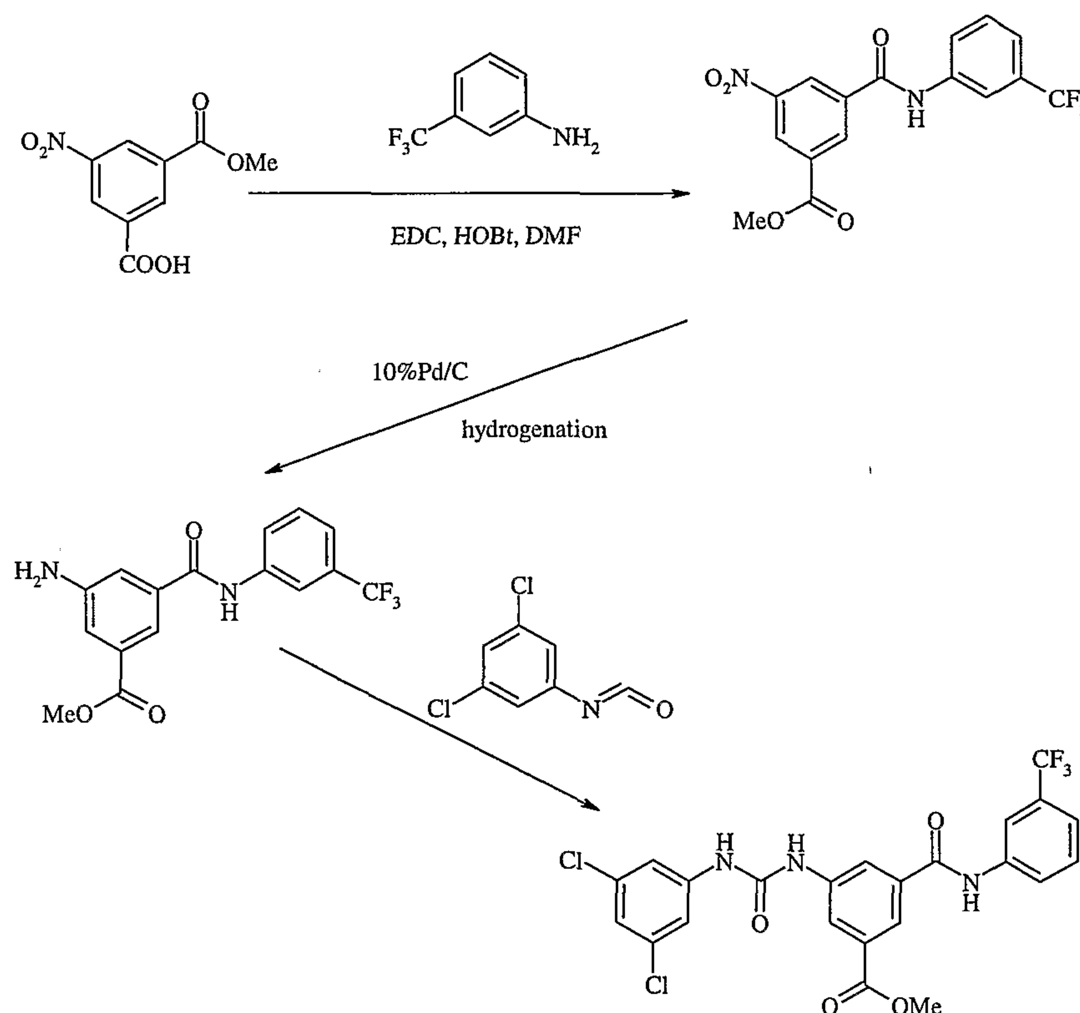
Scheme III-B
