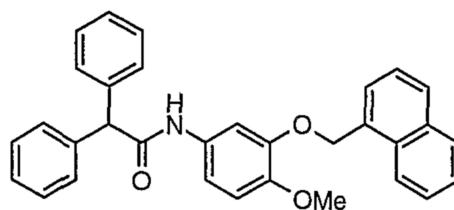
Compound # 49
