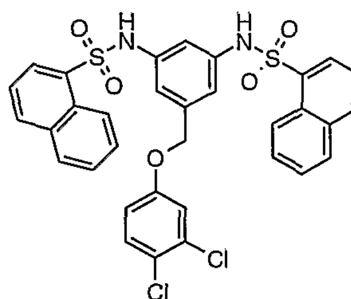
Compound # 7
