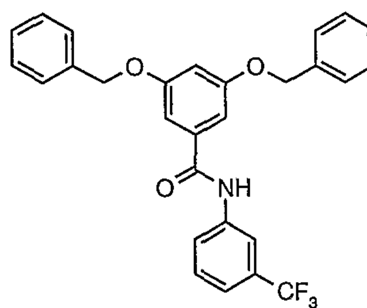
Compound # 8
