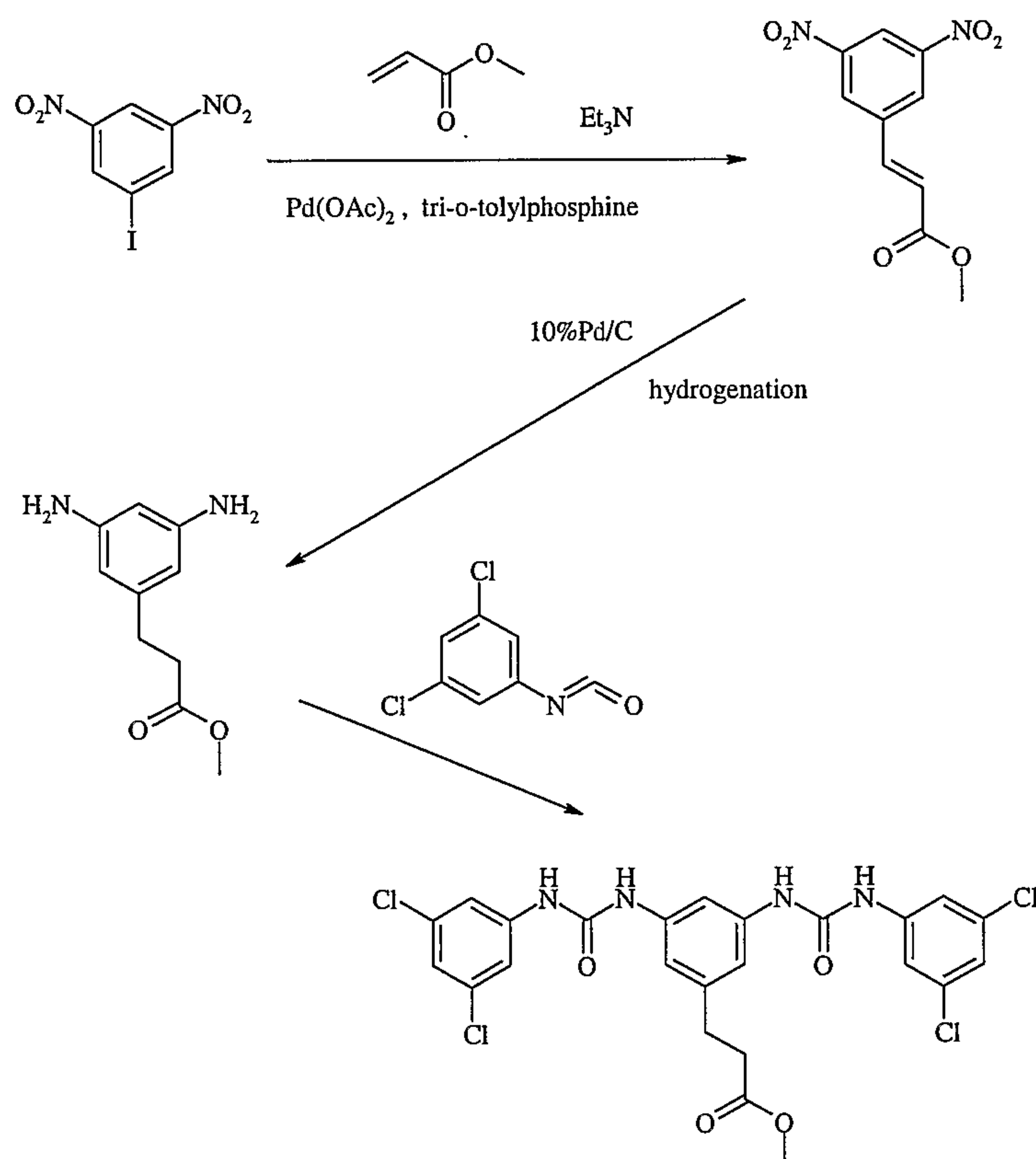
Scheme III-A
