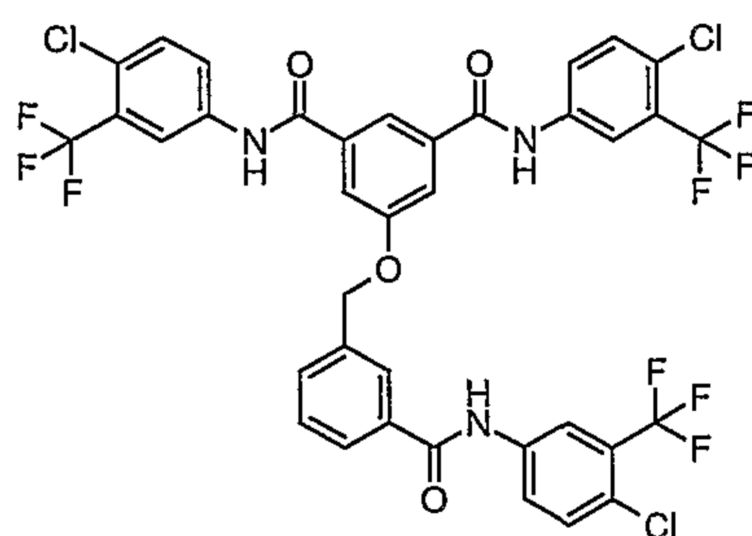
Compound # 37
