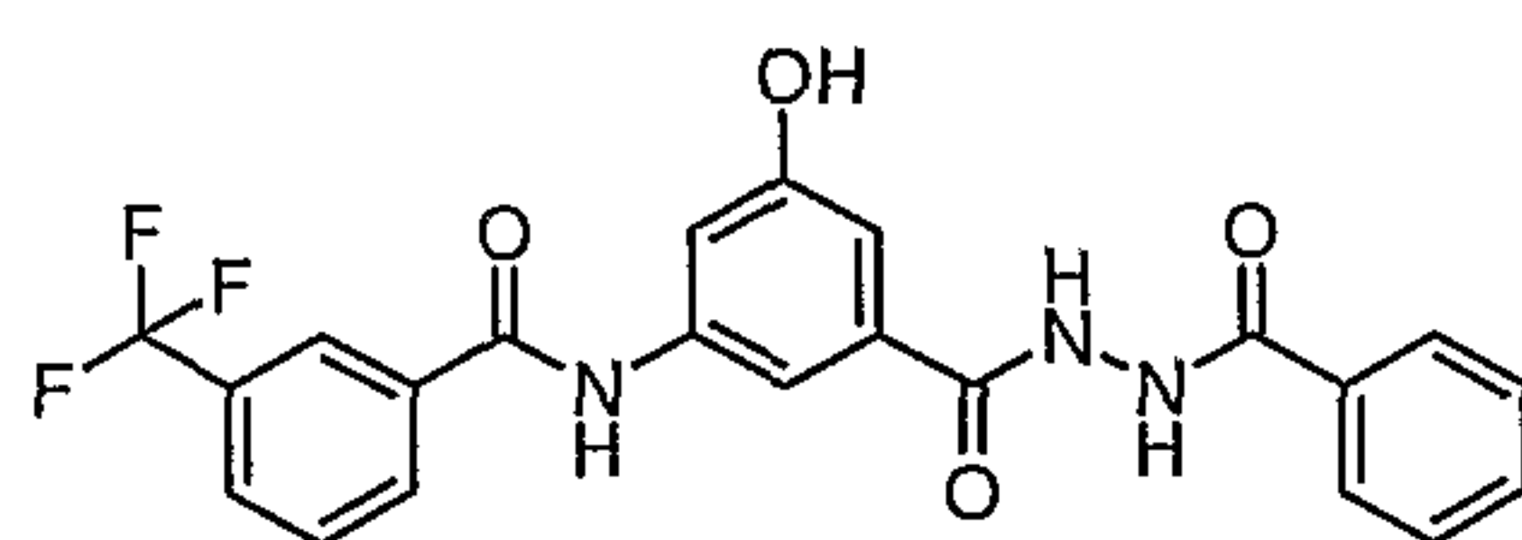
Compound # 15
