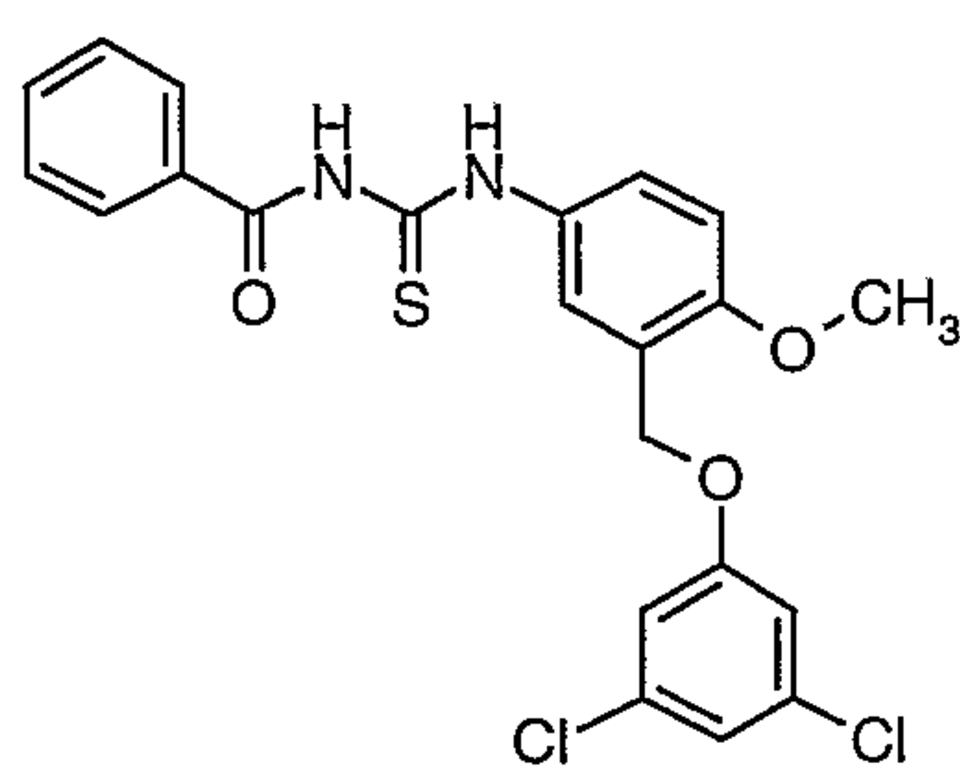
Compound # 46
