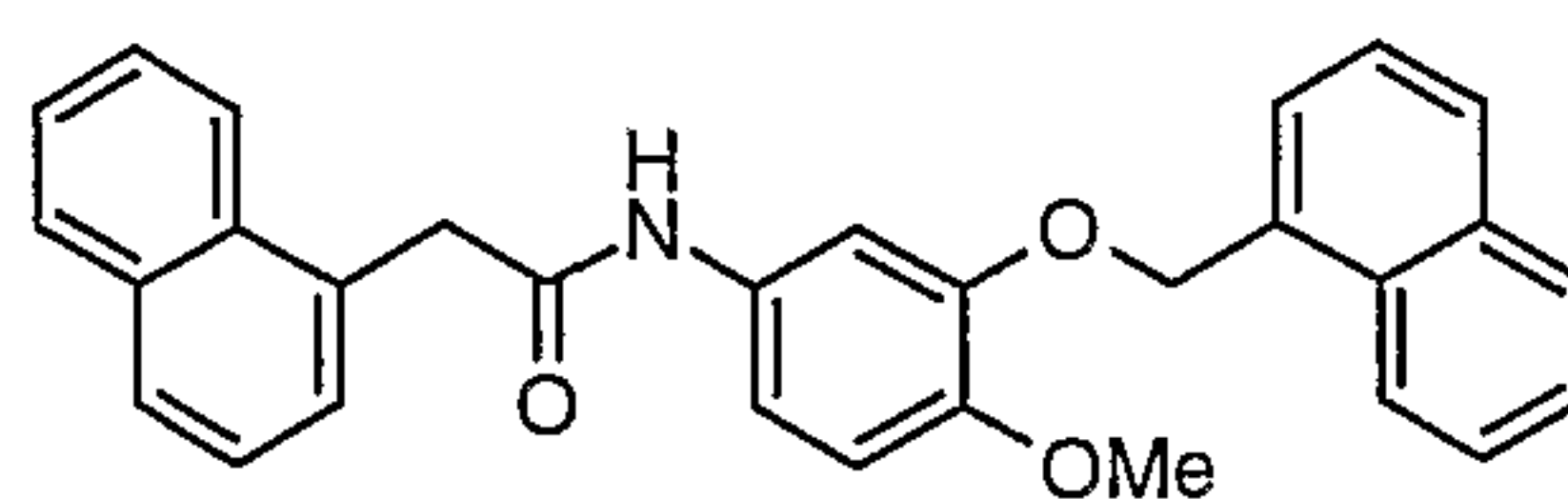
Compound # 48
