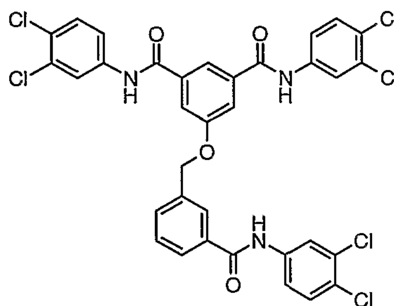
Compound # 38
