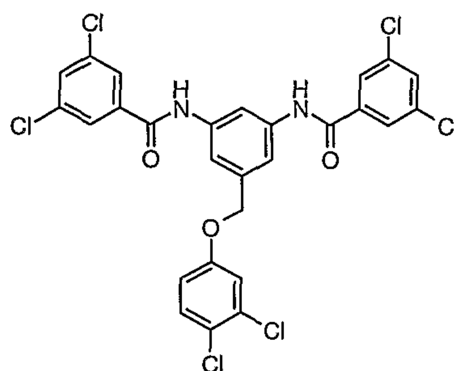
Compound # 6
