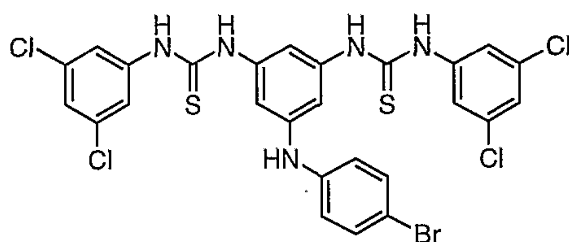
Compound # 11
