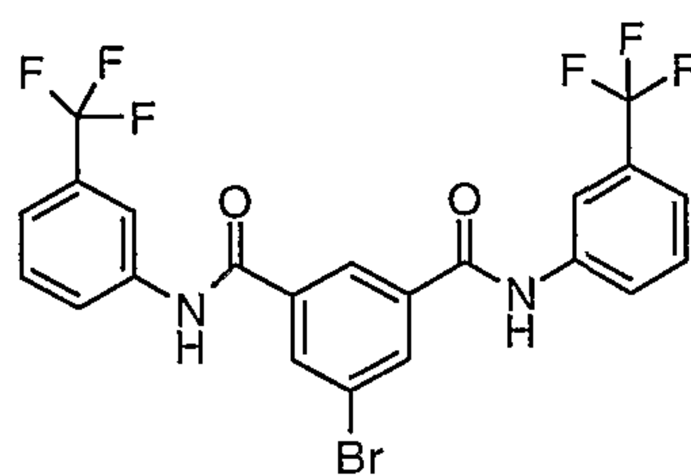
Compound # 26
