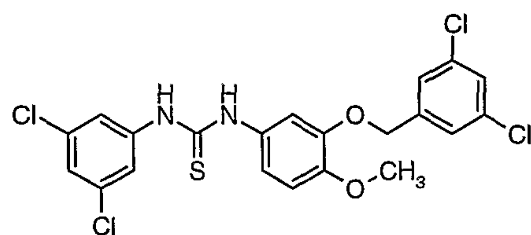
Compound # 28
