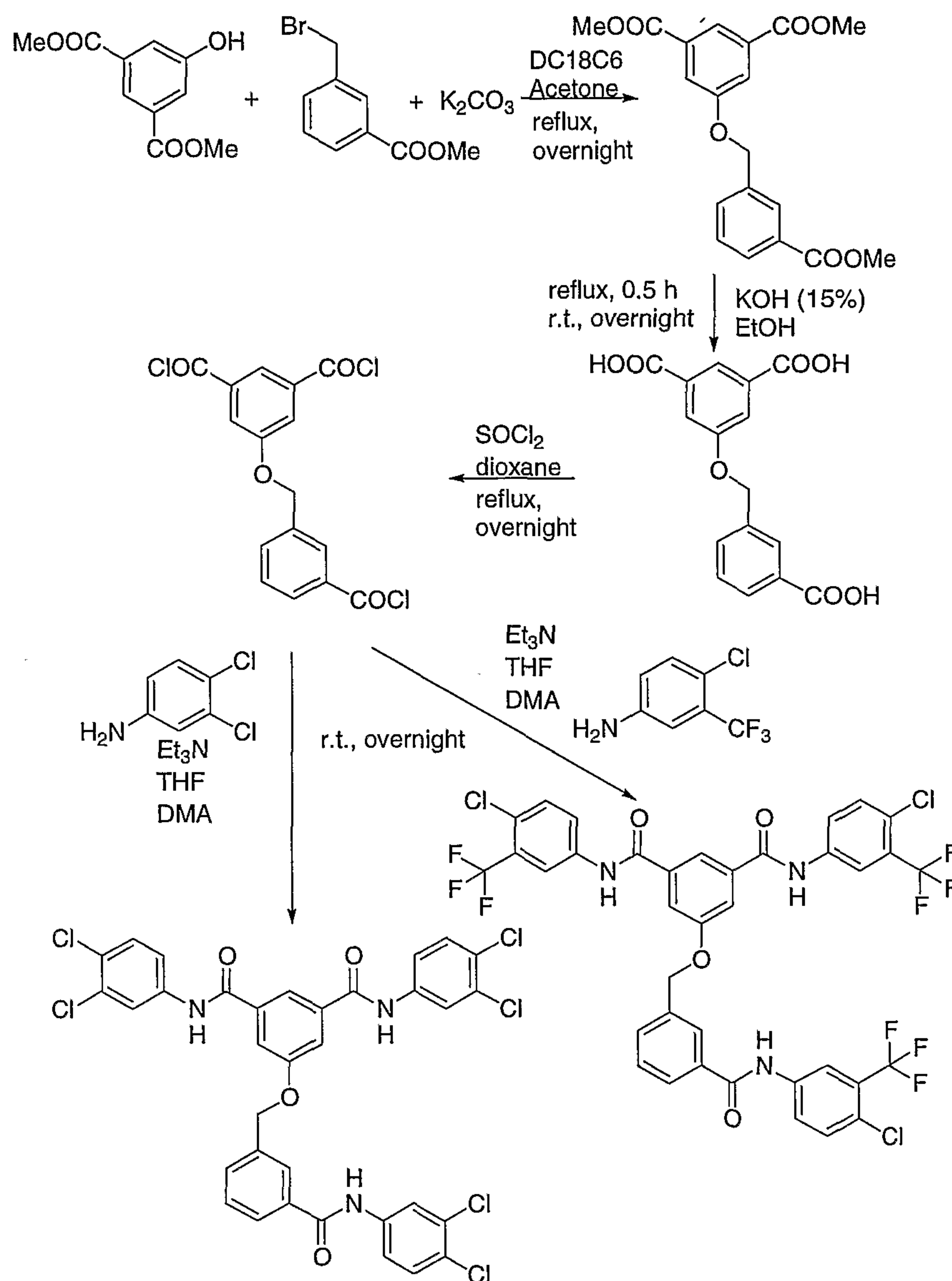
Scheme I-G
