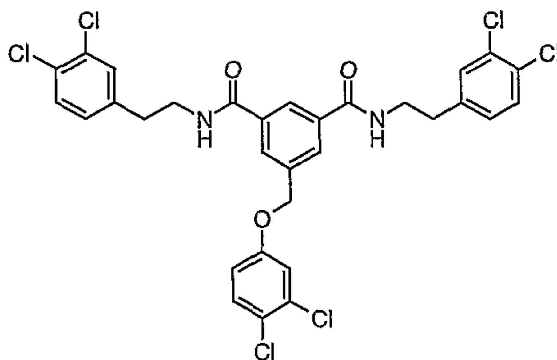
Compound # 19
