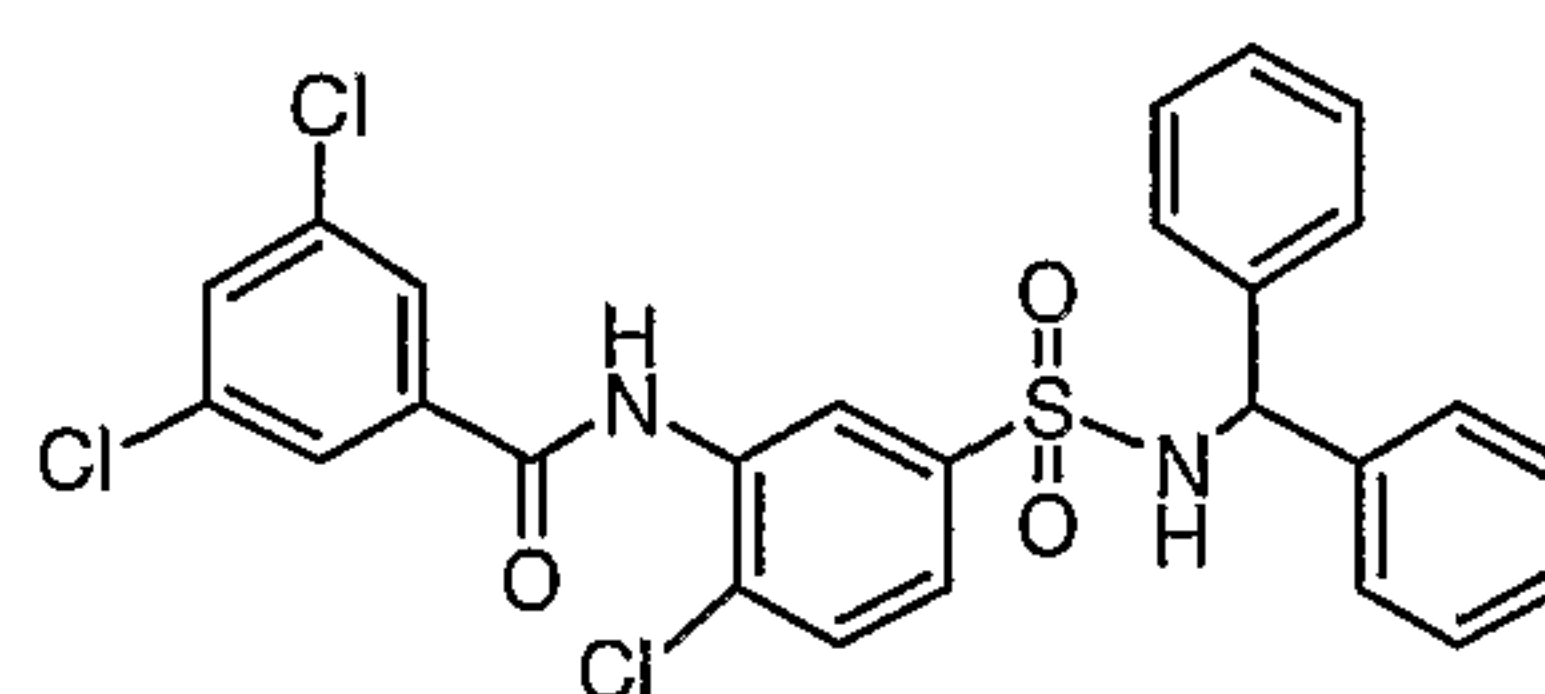
Compound # 52
