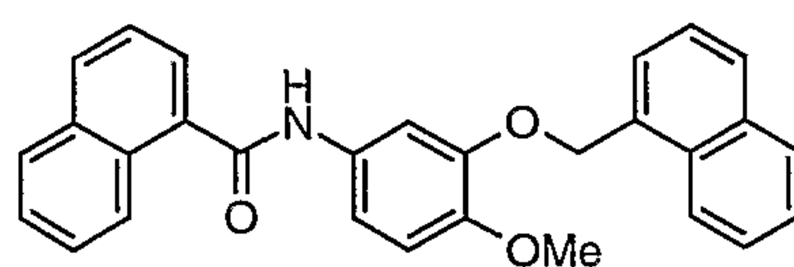
Compound # 47
