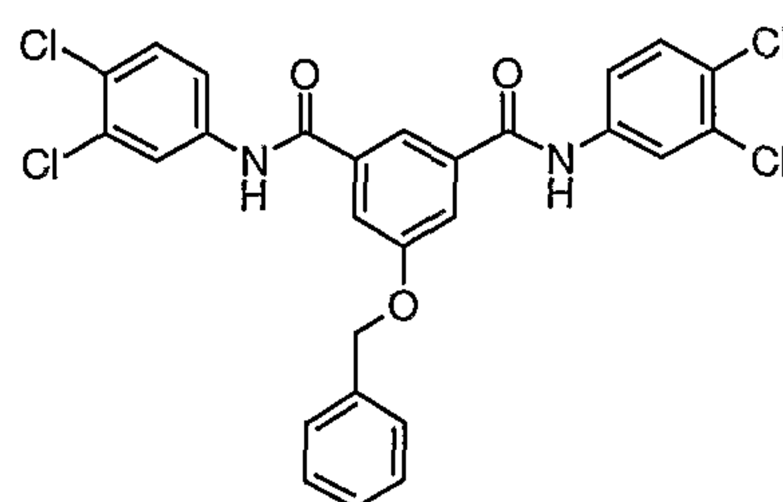
Compound # 43
