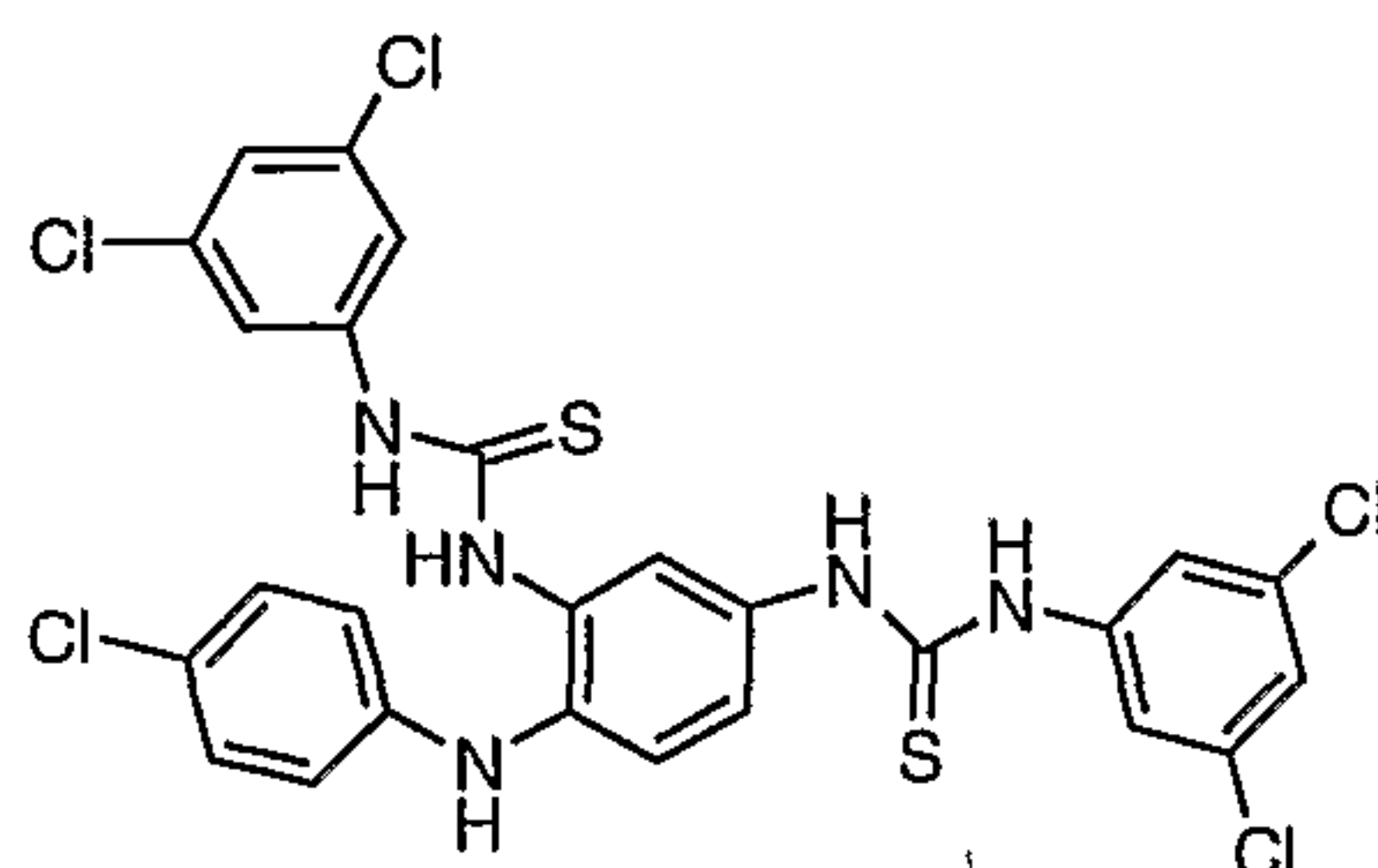
Compound # 36
