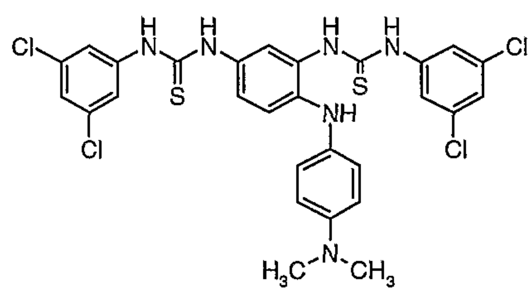
Compound # 35
