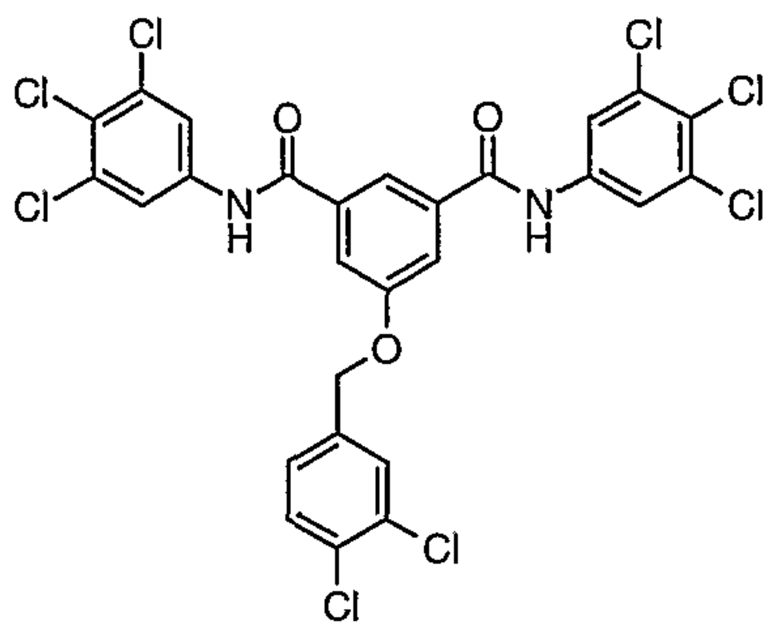
Compound # 32
