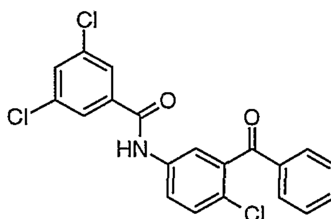
Compound # 51
