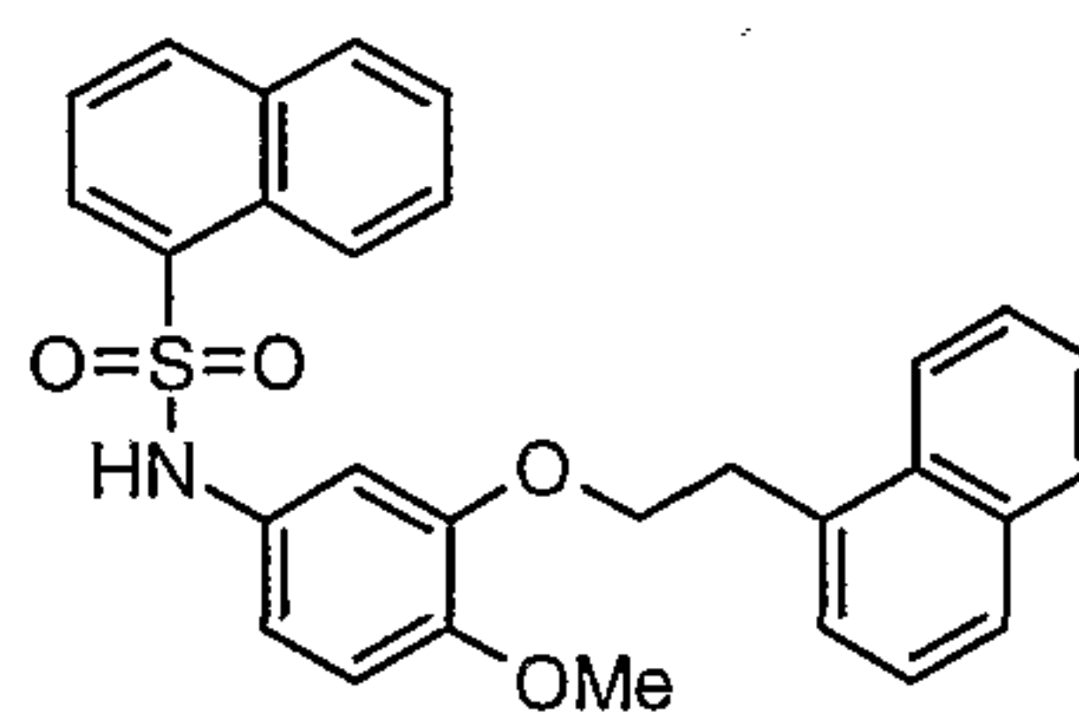
Compound # 50
