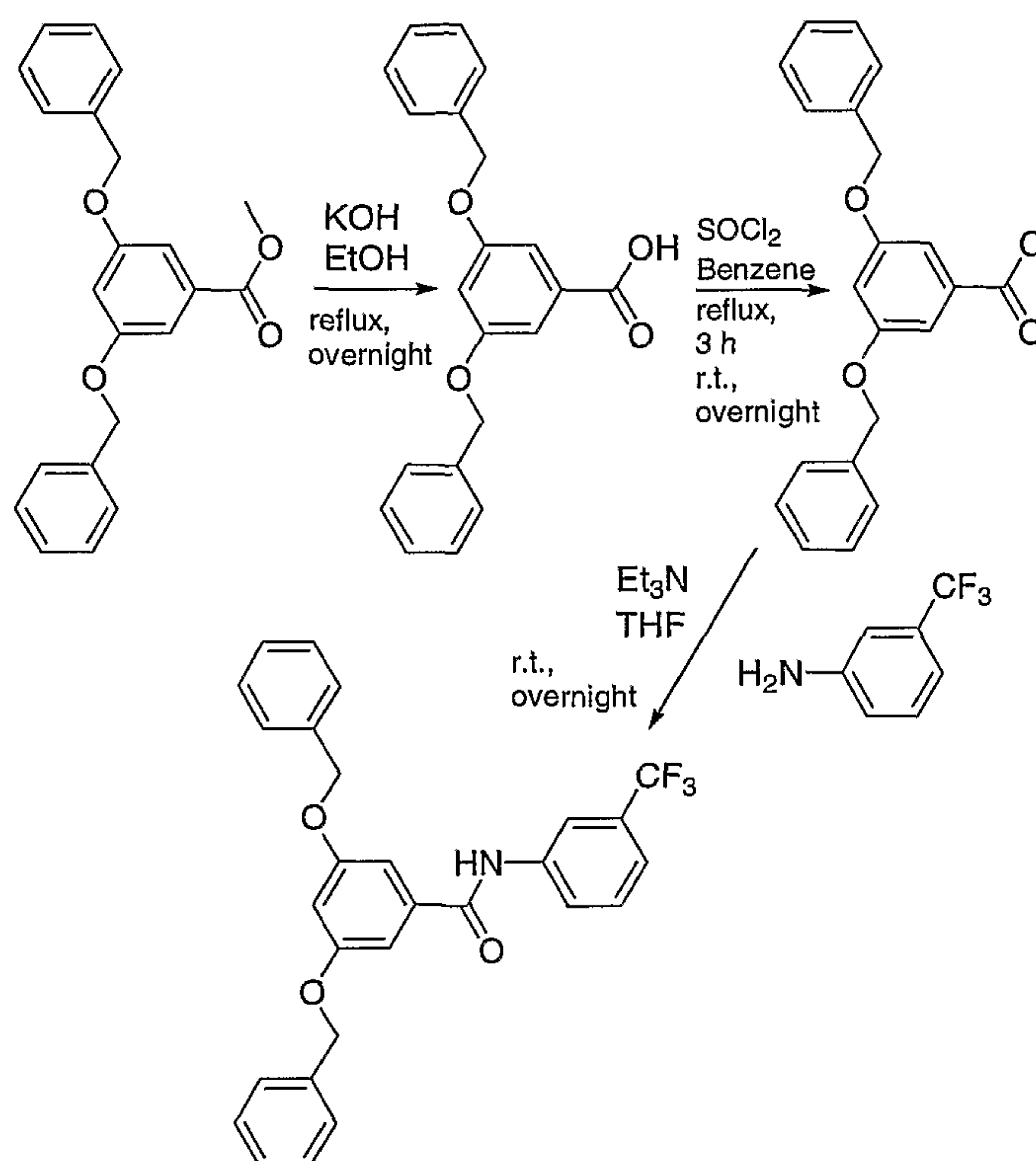
Scheme V
