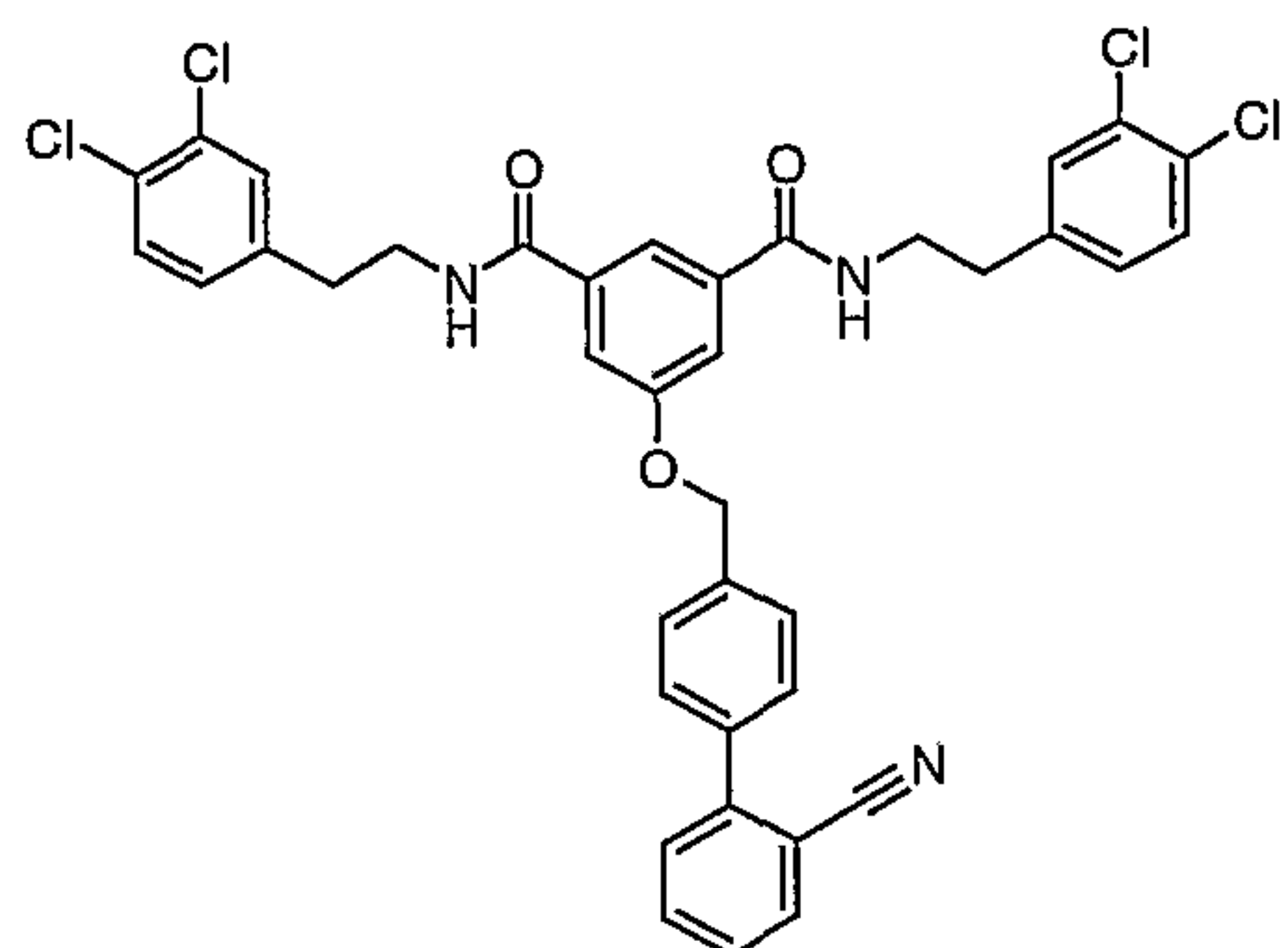
Compound # 21
