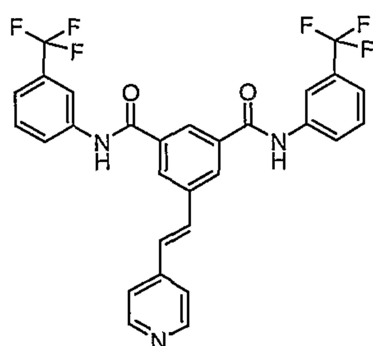
Compound # 16
