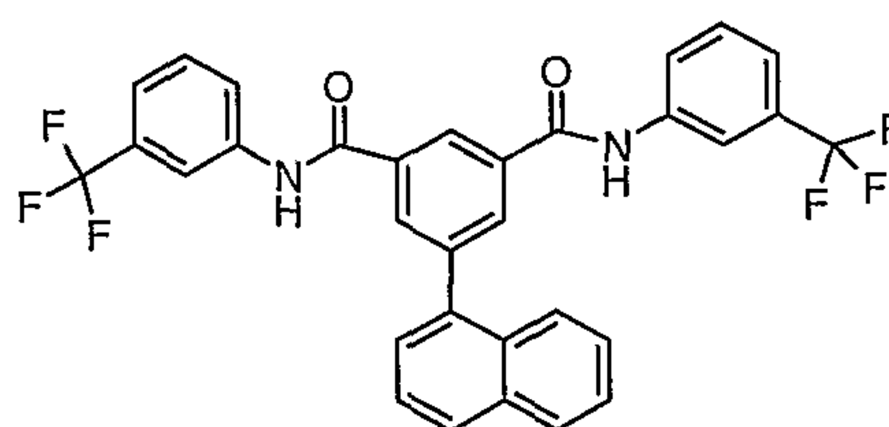
Compound # 3
