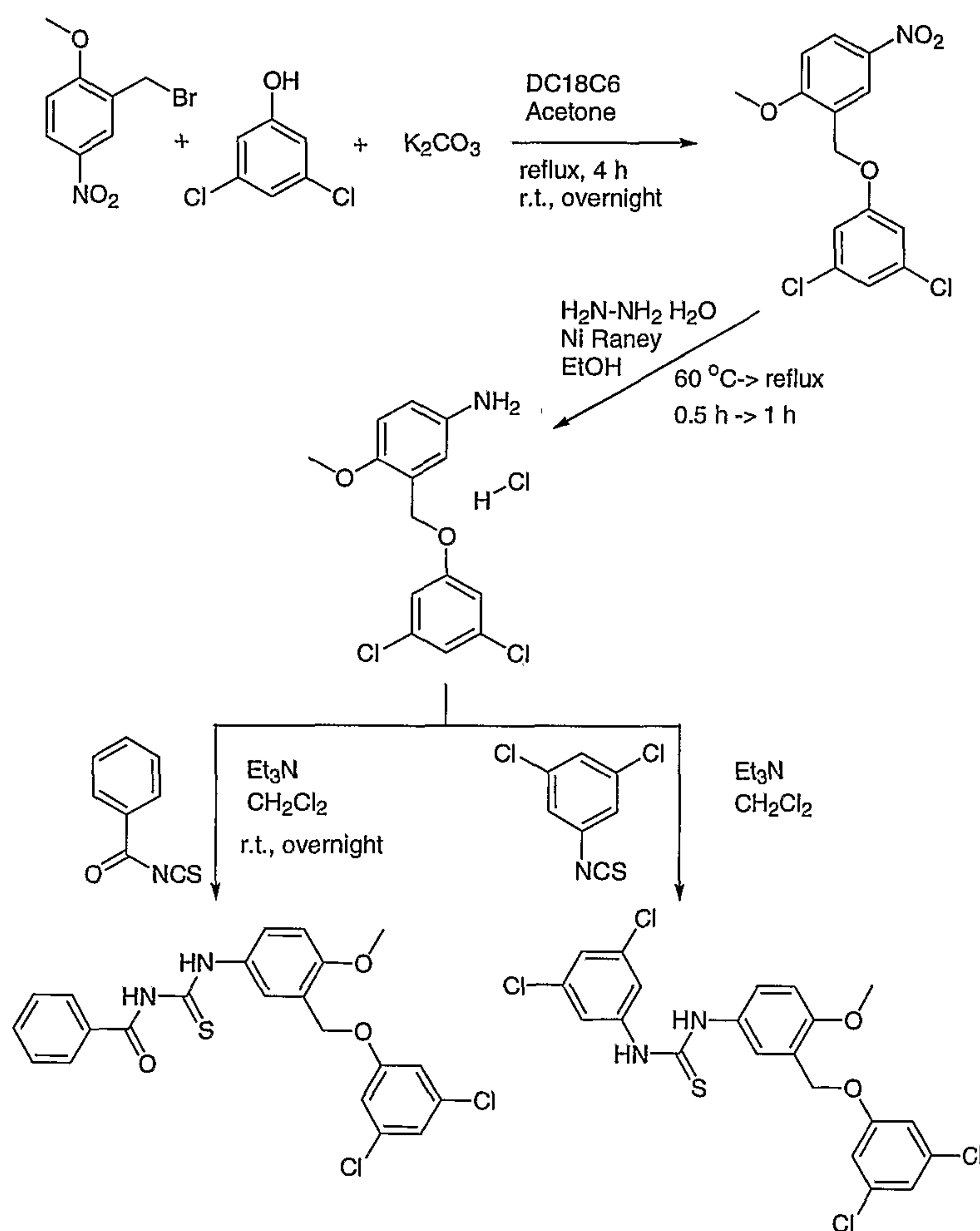
Scheme VIII
