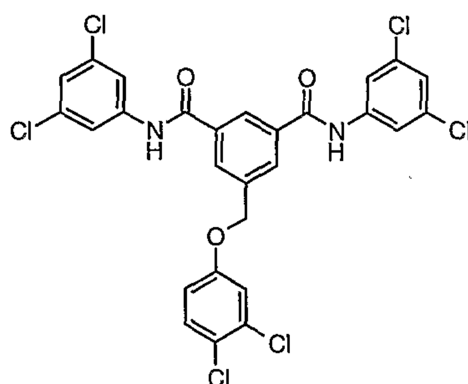
Compound # 20
