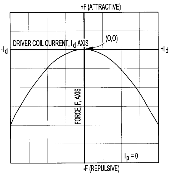
FORCE vs. I_d FOR "PUSH" HTS DRIVER
