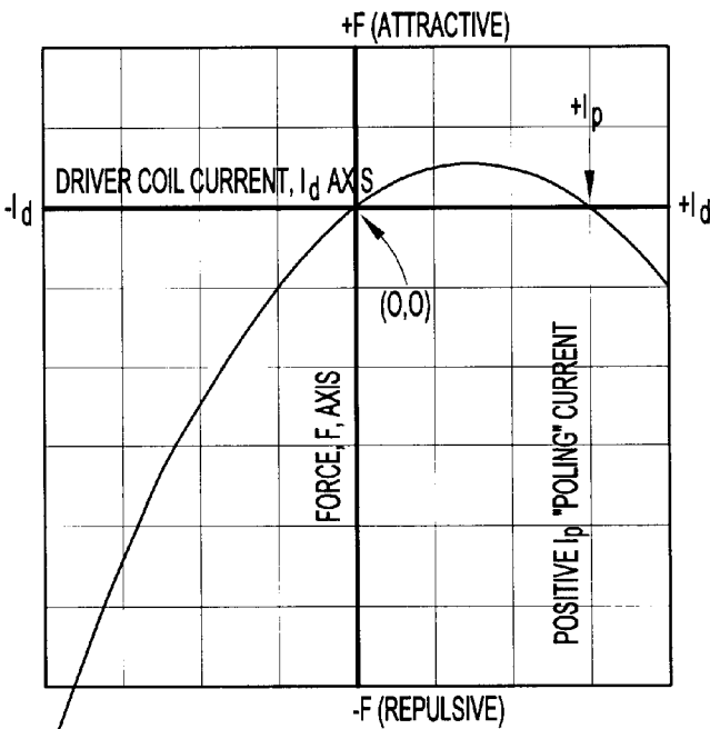
FORCE vs. I_d FOR "PUSH-PULL" HTS DRIVER
