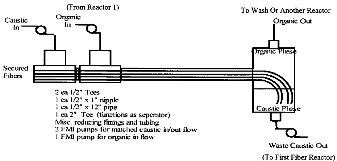
Reactor 2
