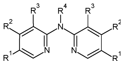
Formula H-III
