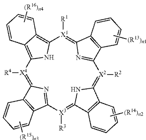
Formula Y-II
