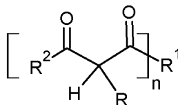
Formula D-II
