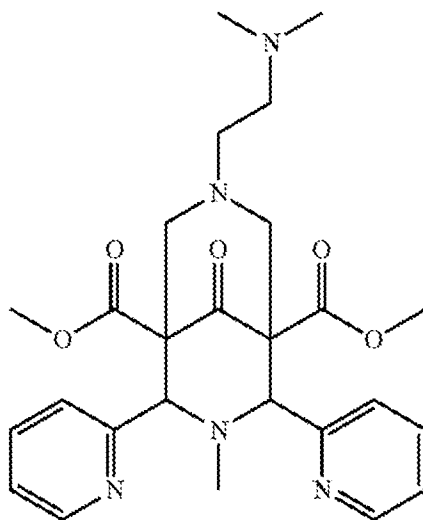
Formula N-Ib
