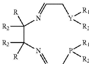
Formula P-IV
