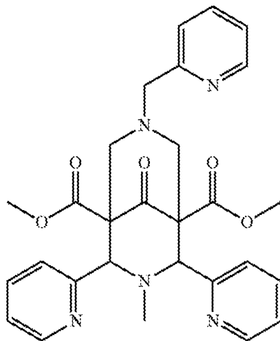
Formula N-Ia
