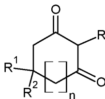
Formula D-IV
