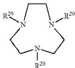
Formula N-III
