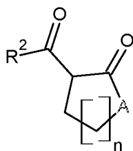
Formula D-III
