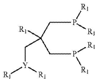
Formula P-III
