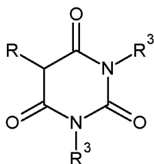
Formula D-V
