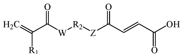
Formula C-II
