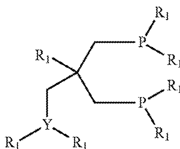
Formula P-III
