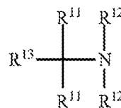
Formula N-II
