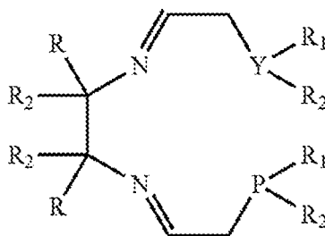
Formula P-IV
