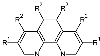
Formula H-II
