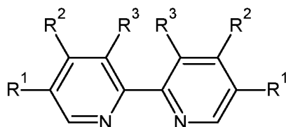
Formula H-I
