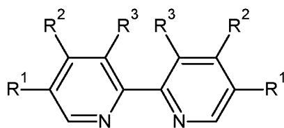
Formula H-I
