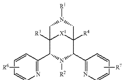
Formula N-I
