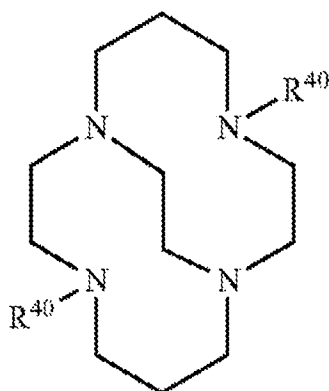
Formula N-V
