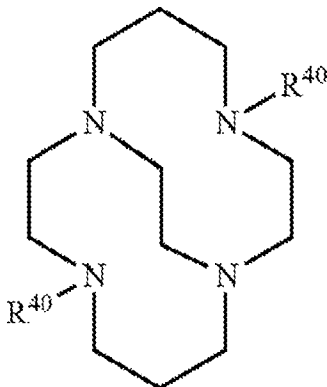
Formula N-V
