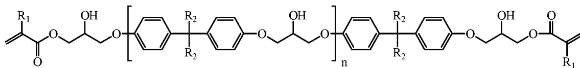
Formula E-I
