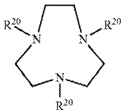
Formula N-III
