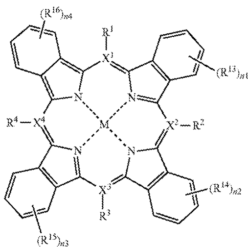
Formula Y-IIa
