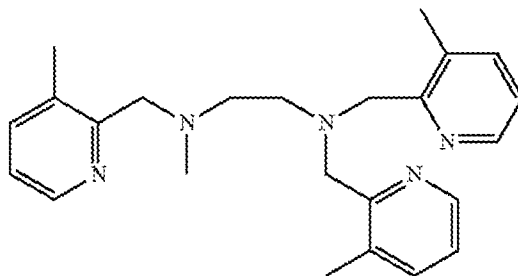
Formula N-XIV
