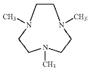
Formula N-XV
