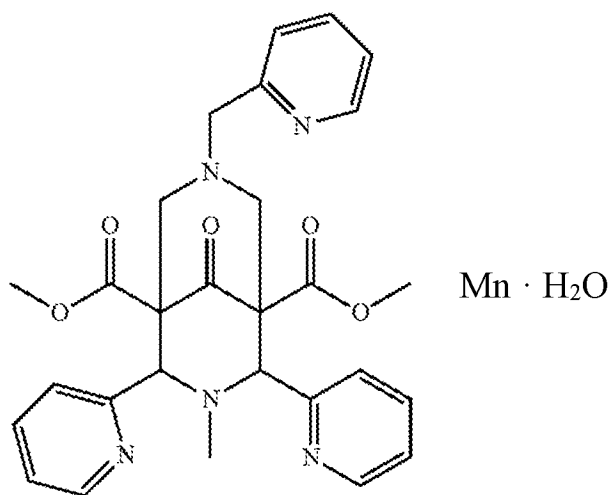
Formula N-XX
