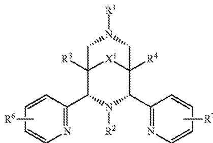
Formula N-I
