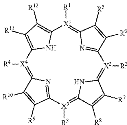
Formula Y-I
