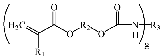
Formula C-I
