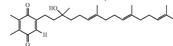
Gamma-tocotrienol quinone
