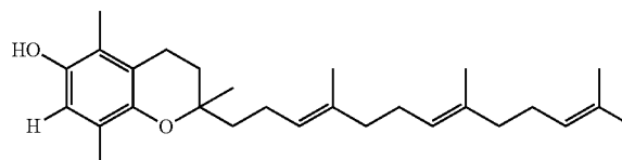
Beta-tocotrienol
