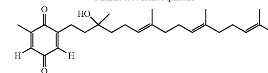
Delta-tocotrienol quinone
