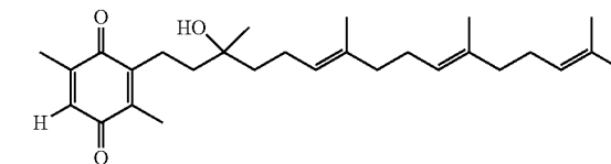
Beta-tocotrienol quinone
