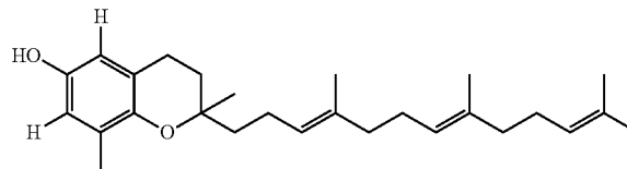
Delta-tocotrienol
