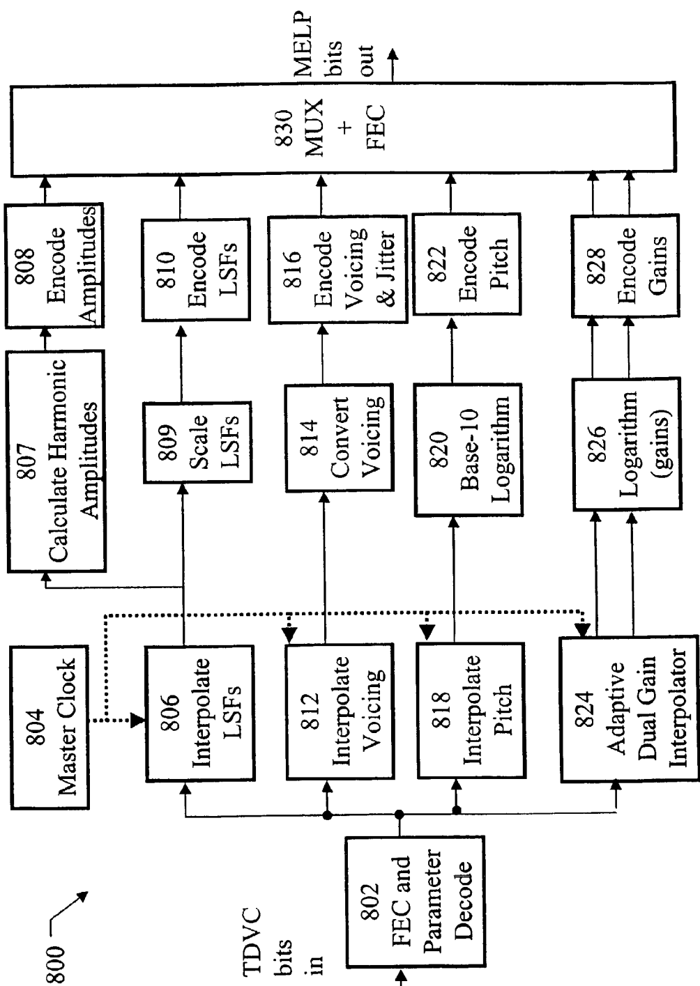
Figure 8: TDVC to MELP Transcoder
