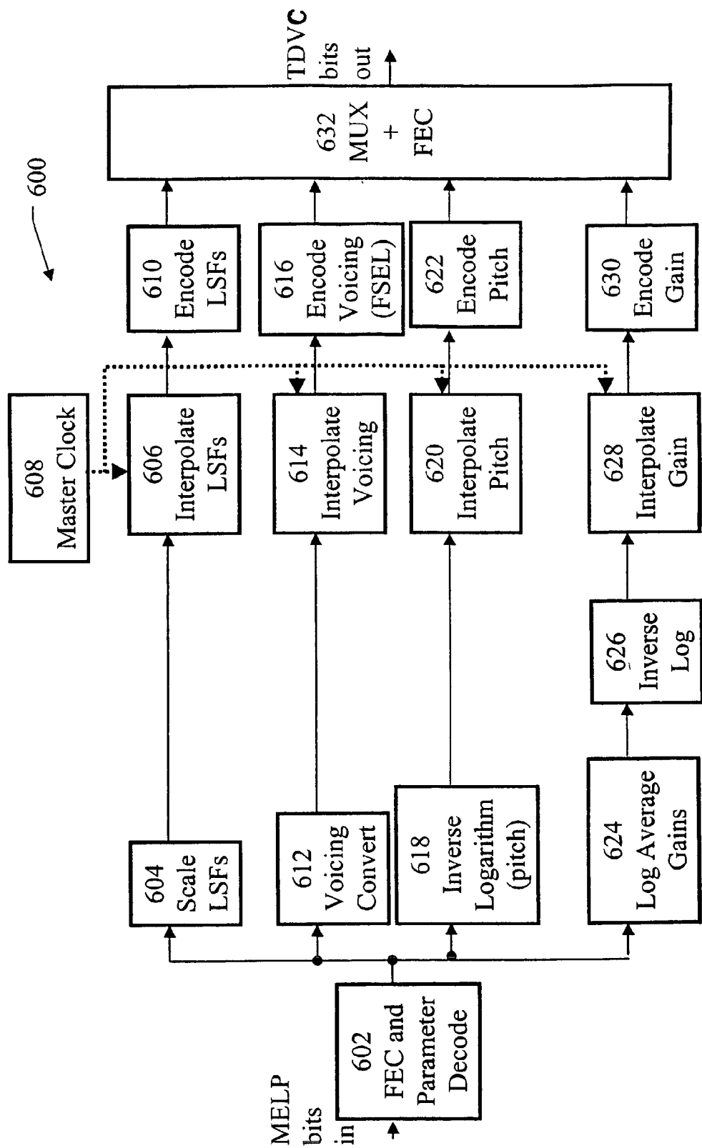
Figure 6: MELP to TDVC Transcoder
