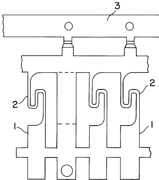
FIG. 11 PRIOR ART
