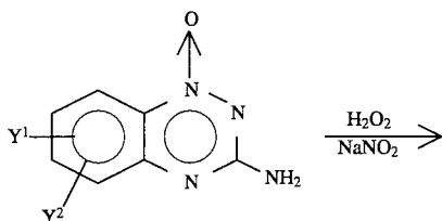
Scheme IV
