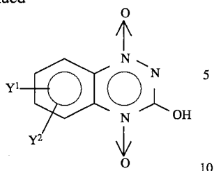
Scheme IV
