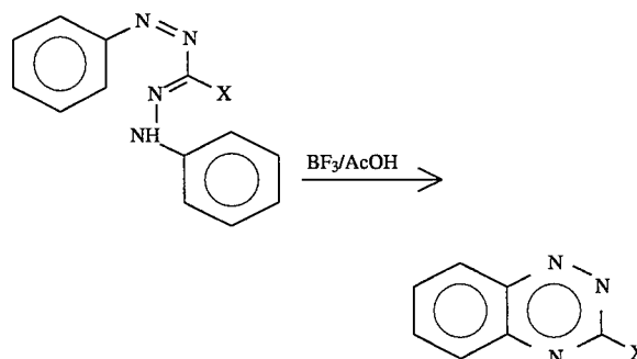
Scheme III
