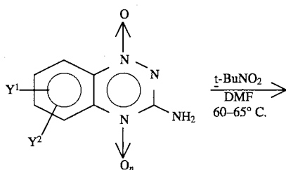
Scheme V
