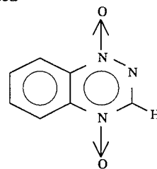
9 1,2,4-benzotriazine 1,4-dioxide
