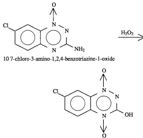
11 7-chloro-3-hydroxy-1,2,4-benzotriazine 1,4-dioxide
