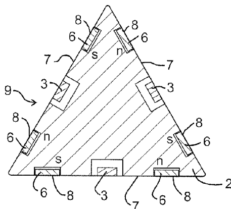
FIG. 5 SECTION C-C
