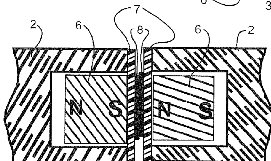
FIG. 10 SECTION B-B
