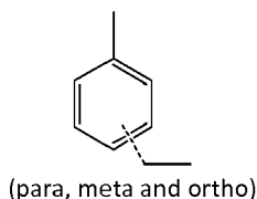
MEB isomers
