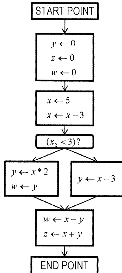
FIG. 4 CONTROL FLOW GRAPH REPRESENTATION
