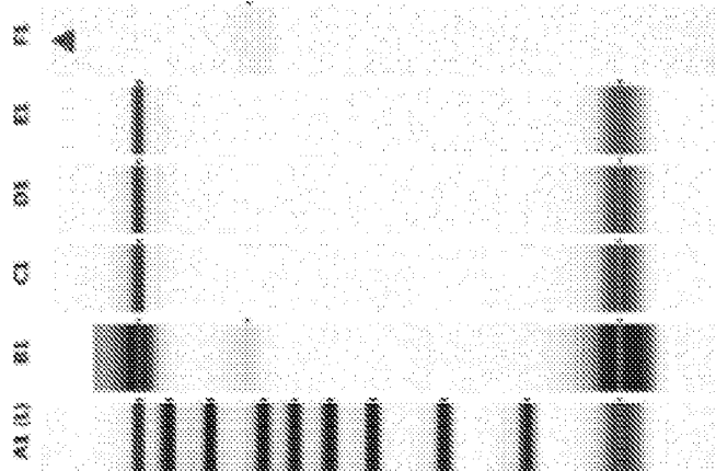
Gel Image
