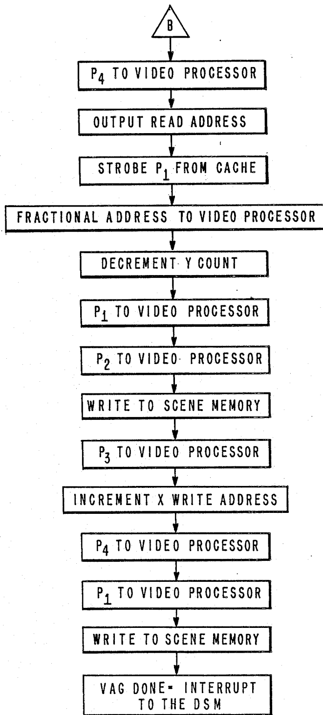
VAG CONTROL FLOW BILINEAR INTERPOLATION MODE
