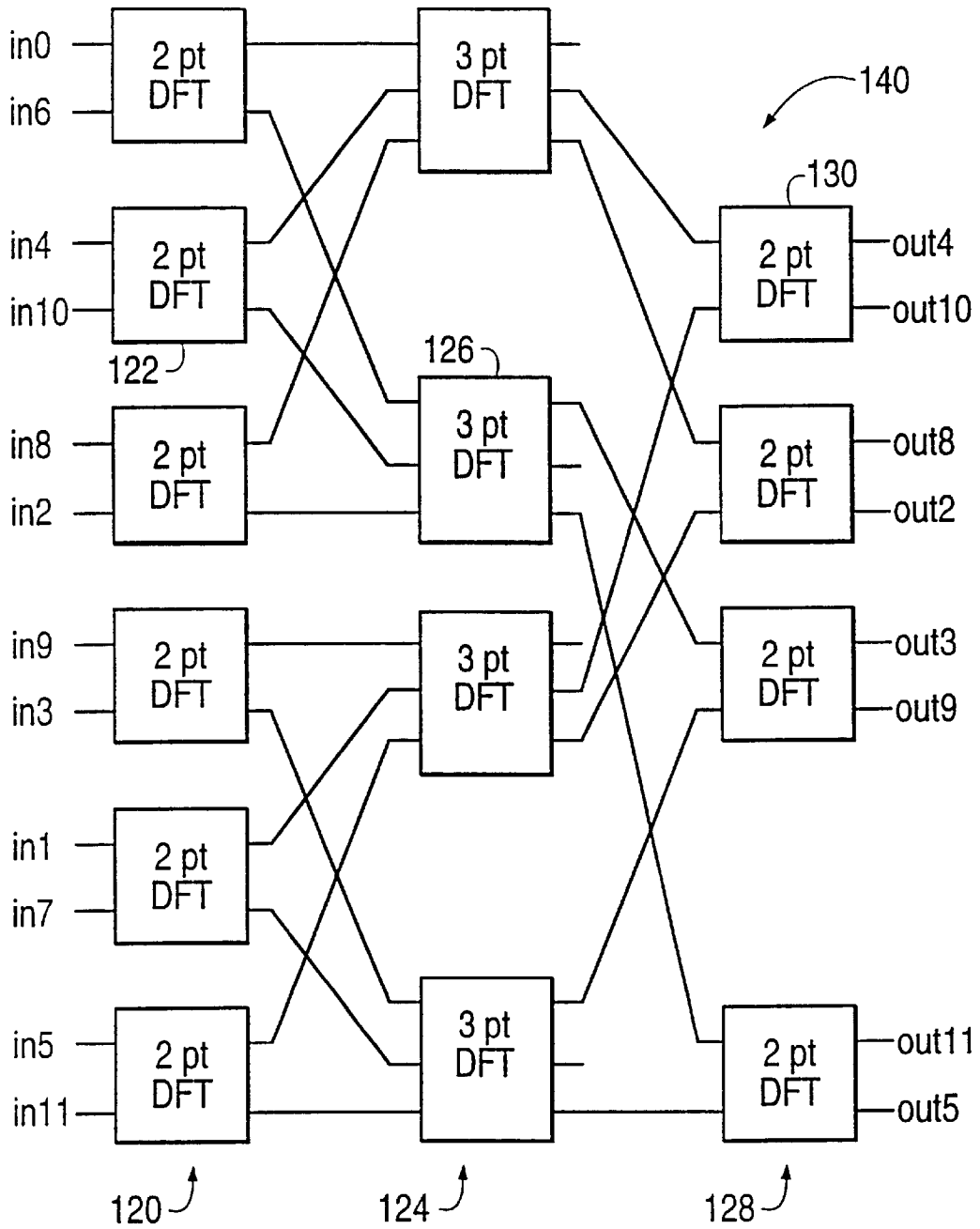
FIG. 9 (PRIOR ART)
