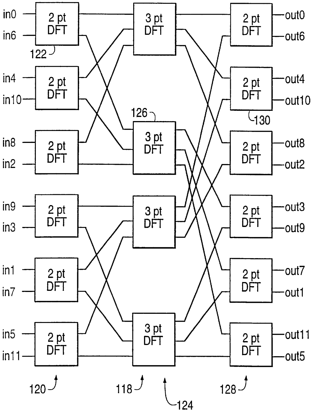
FIG. 8 (PRIOR ART)
