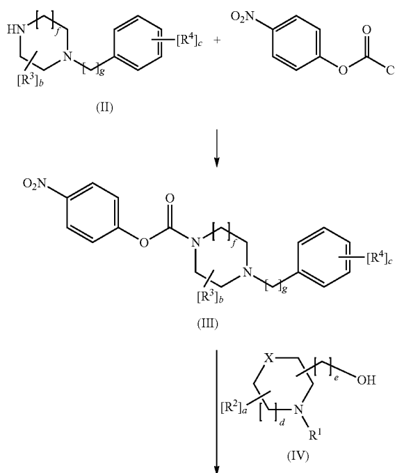
Scheme 1. Preparation by activation of the piperazine moiety
