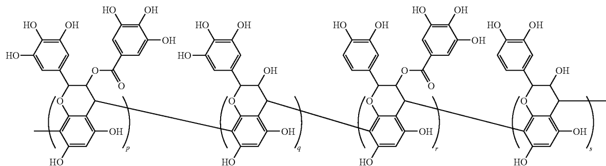
Probable Structural Formula of Persimmon Condensed Tannin
