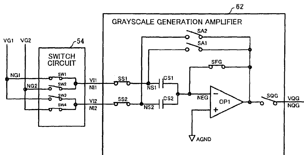
FIG. 11A SAMPLING PERIOD
