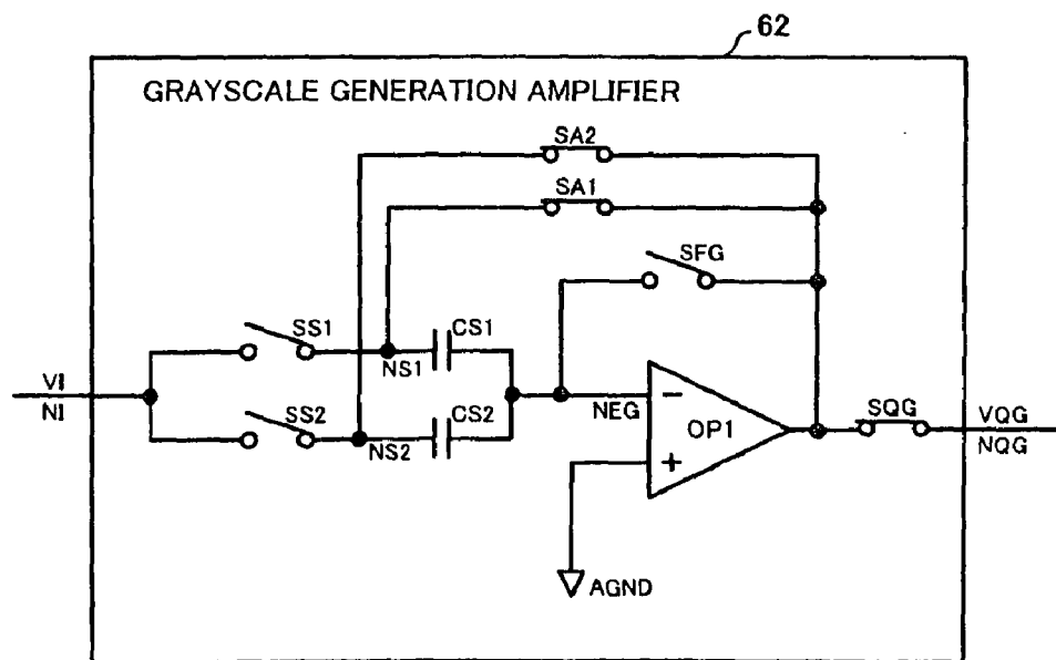
FIG. 13B HOLDING PERIOD
