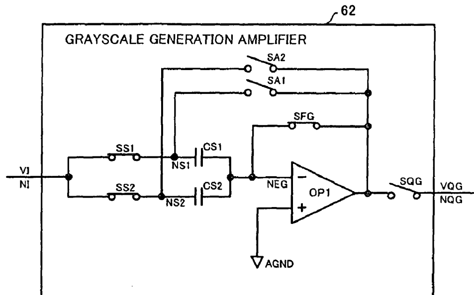
FIG. 13A SAMPLING PERIOD
