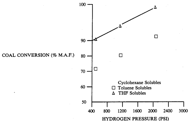
FIG. 3 Effect of Pressure on Present Process
