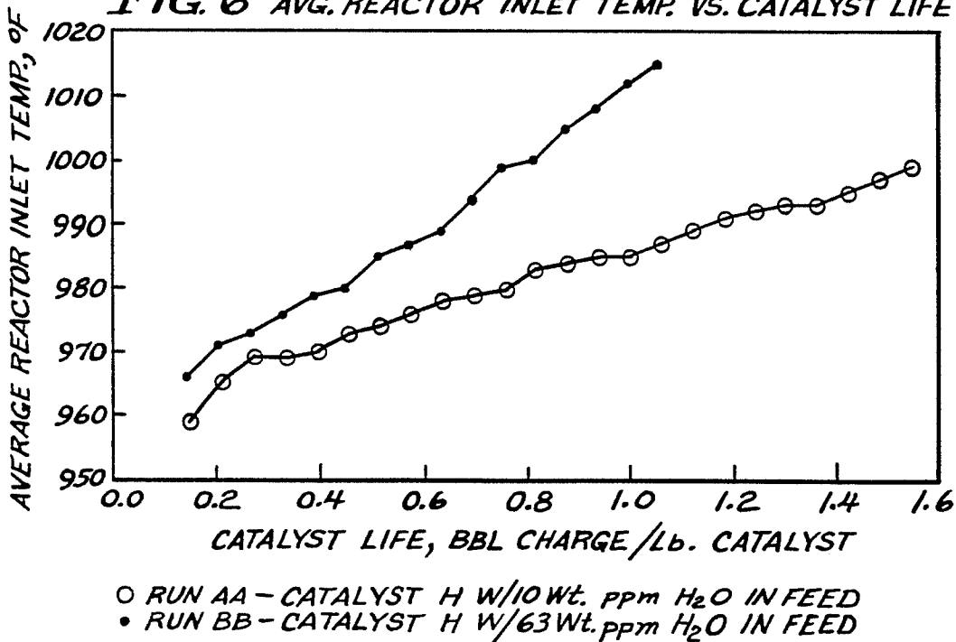
FIG. 6 AVG. REACTOR INLET TEMP. VS. CATALYST LIFE
