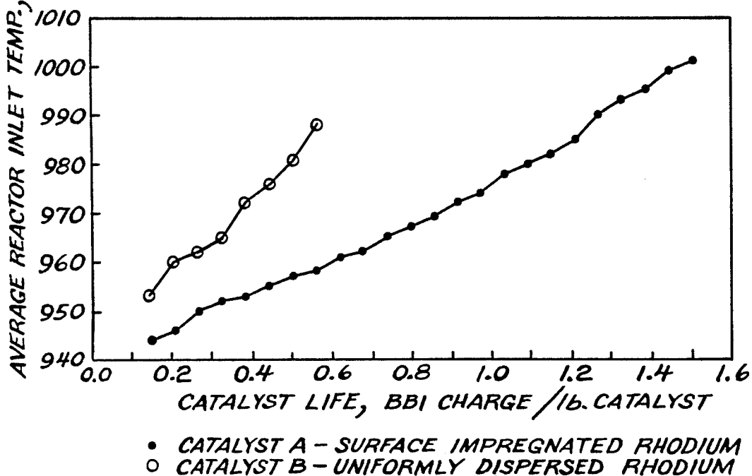
FIG. 4 AVE. REACTOR INLET TEMP. VS CATALYST LIFE
