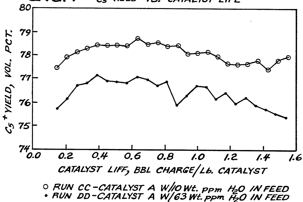
FIG. 7 C_5^+ YIELD VS. CATALYST LIFE
