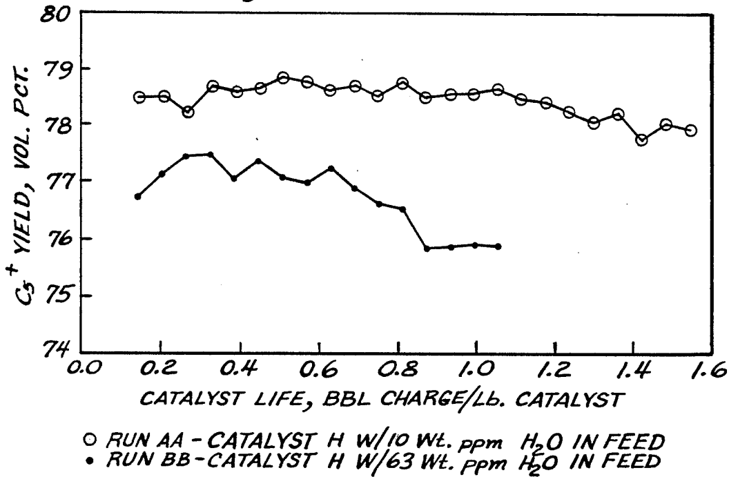
FIG. 5 C 5 + YIELD VS. CATALYST LIFE
