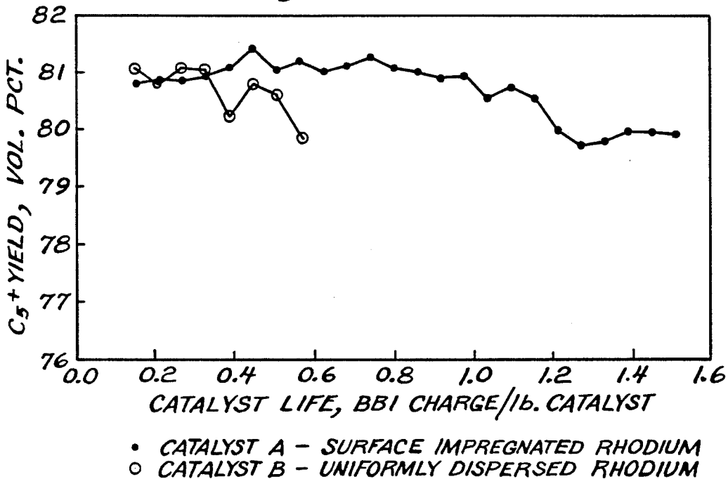
FIG. 3 C_5^+ YIELD VS. CATALYST LIFE
