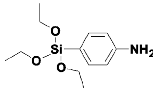
p-aminophenyl triethoxysilane
