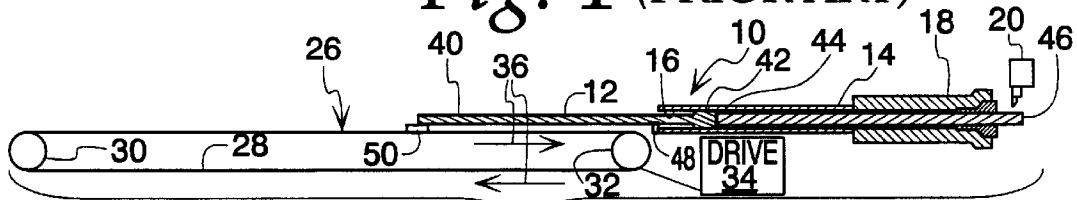
Fig. 2 (PRIOR ART)
