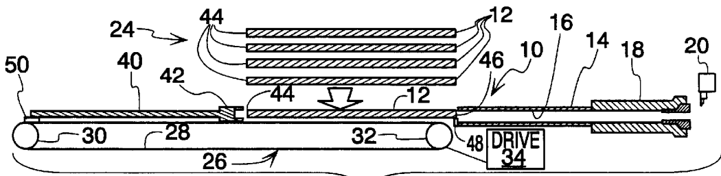
Fig. 1 (PRIOR ART)
