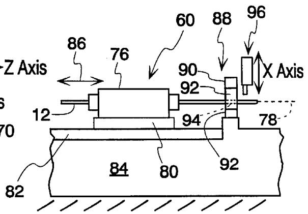
Fig. 13 (PRIOR ART)
