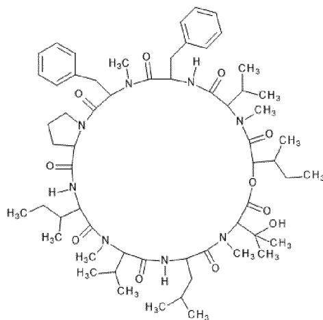
(I-A1); and
