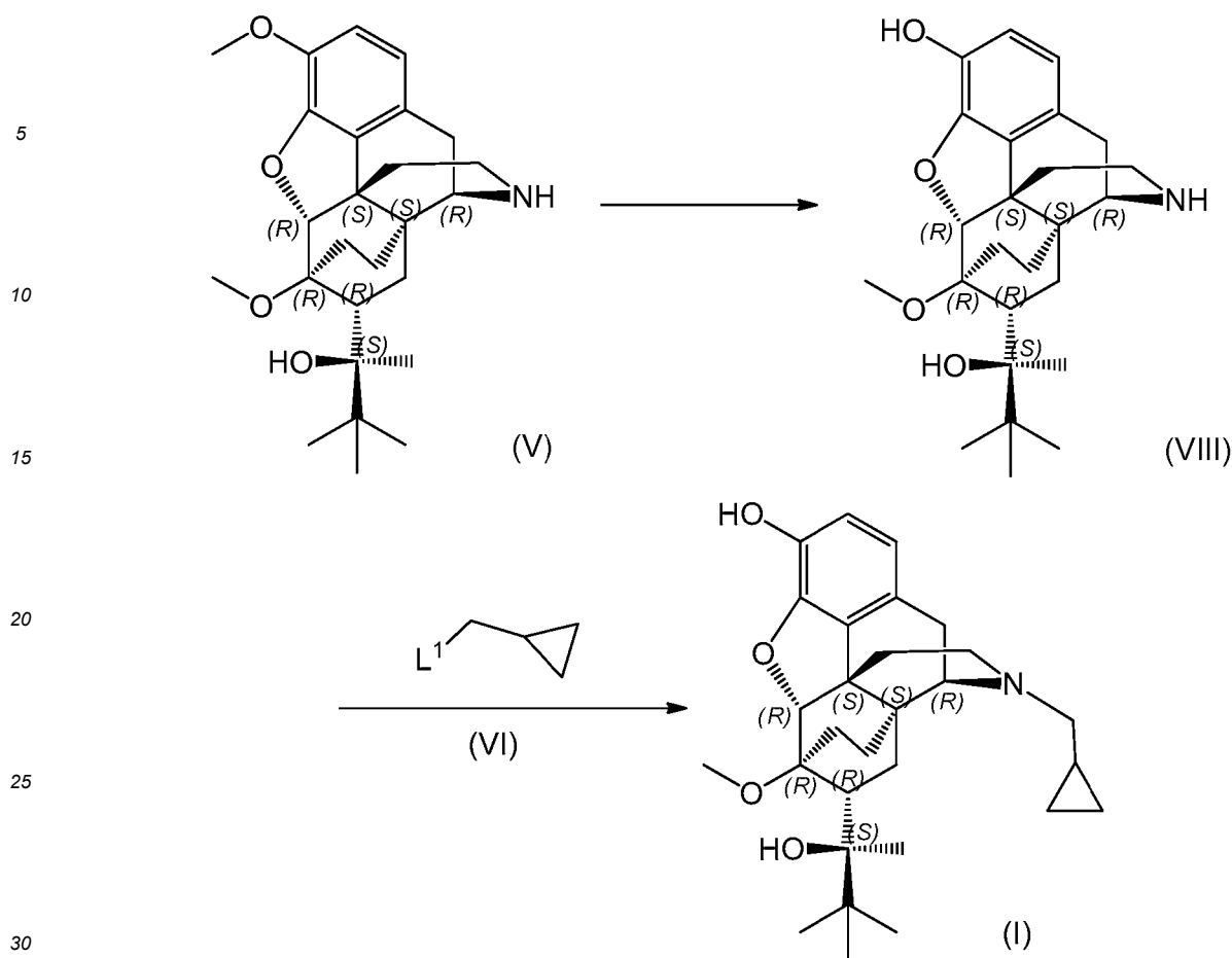
Scheme 2
