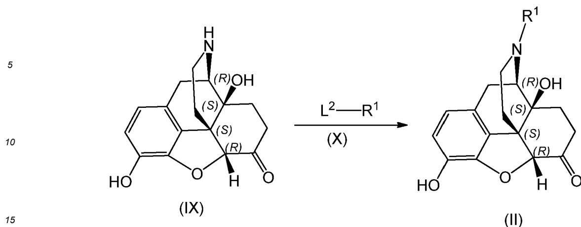
Scheme 3
