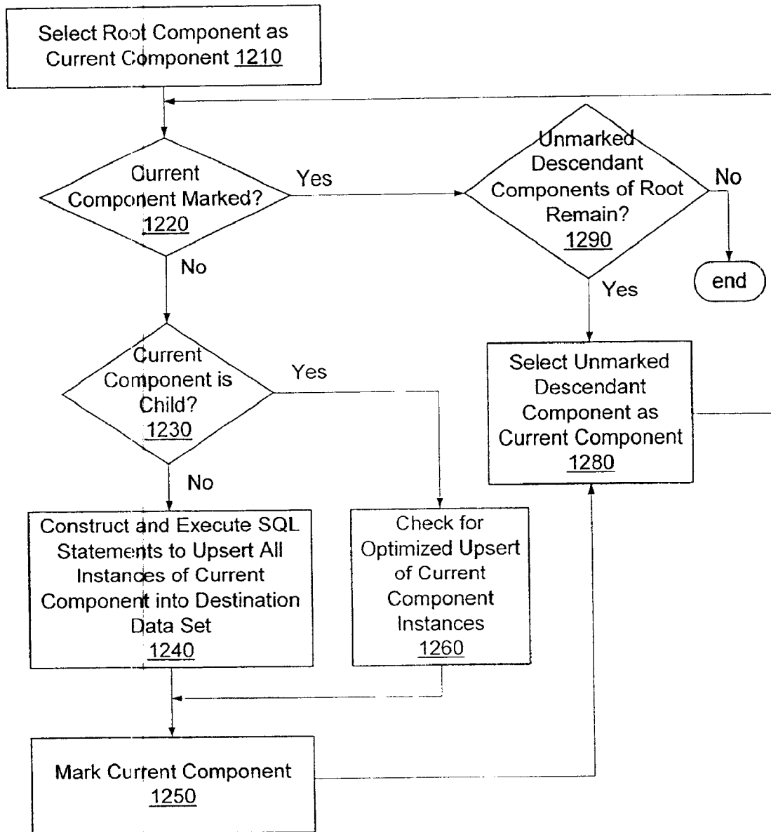
FIG. 12 Upsert Data Set
