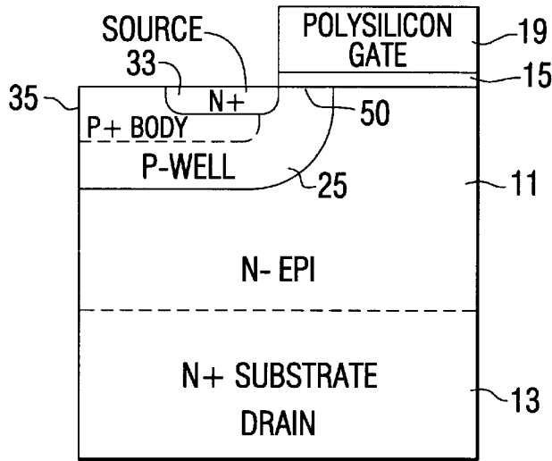
FIG. 7 PRIOR ART
