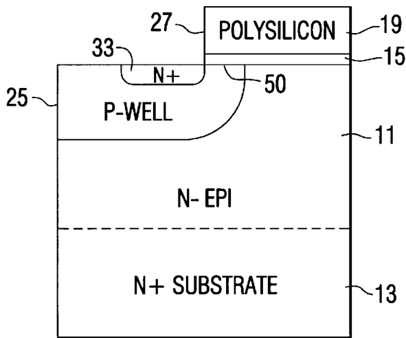
FIG. 6 PRIOR ART
