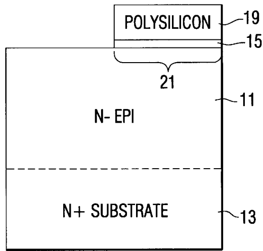
FIG. 4 PRIOR ART
