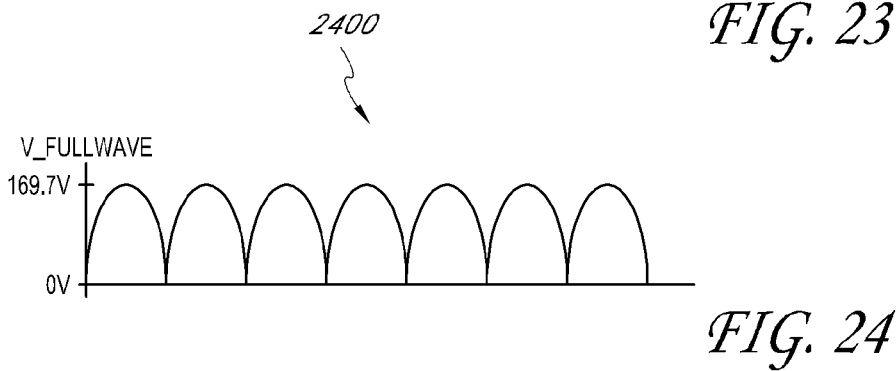
MOSFET Full Wave Rectifier Waveforms
