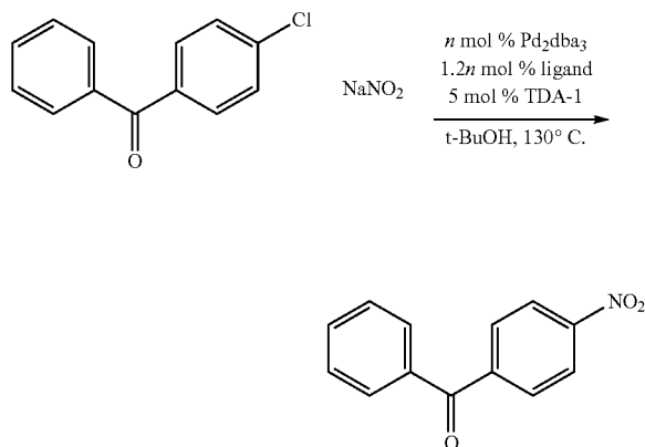
4-Nitrobenzophenone
