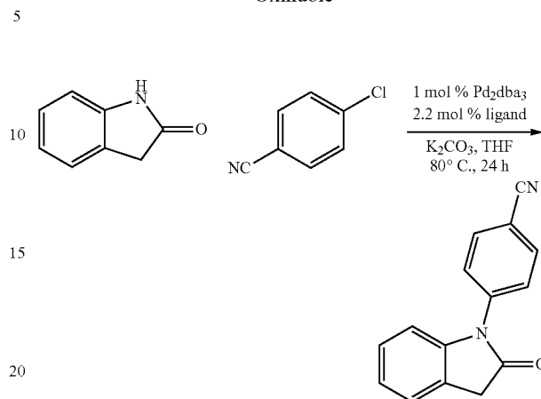
4-(2-Oxoindolin-1-yl)benzonitrile
