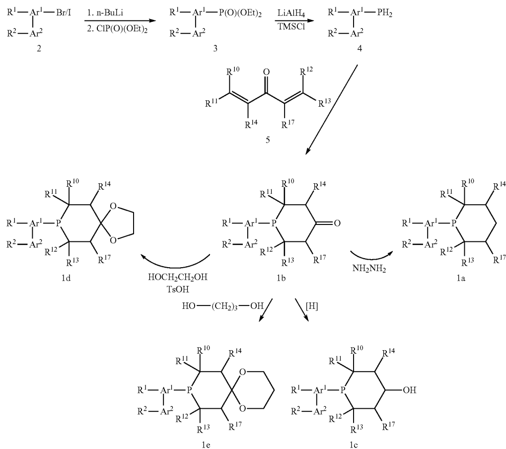
Scheme A
