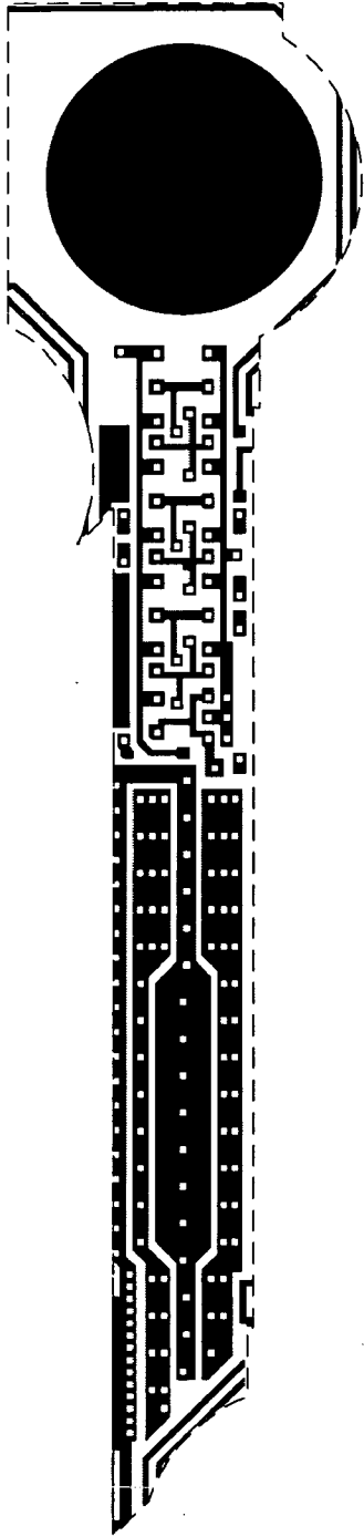
Metal 1 mask
