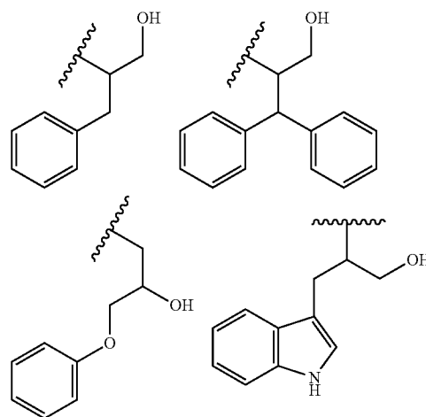
[Chemical formula 37]
