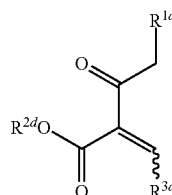
[Chemical formula 8]
