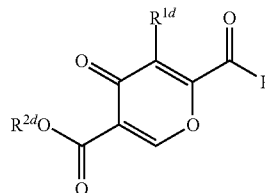
[Chemical formula 39]
