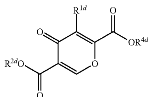
[Chemical formula 12]
