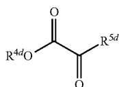
[Chemical formula 3]
