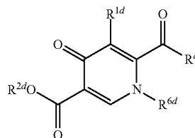
[Chemical formula 10]
