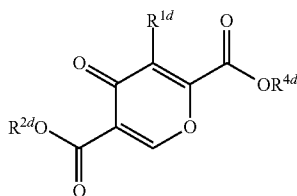
[Chemical formula 4]
