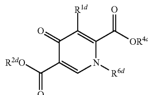
[Chemical formula 6]
