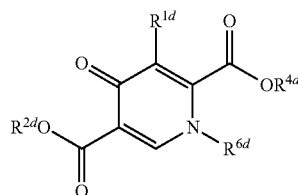
[Chemical formula 15]
