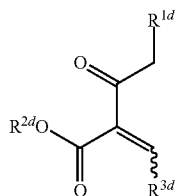
[Chemical formula 10]
