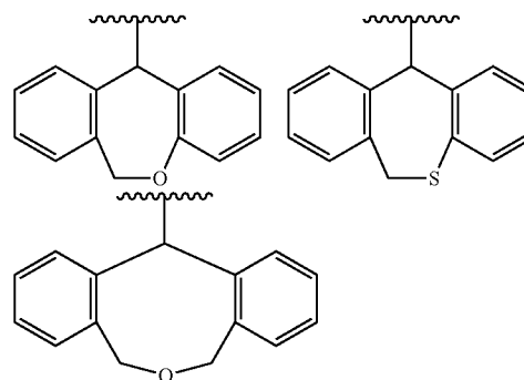
[Chemical formula 36]
