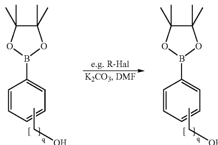
Scheme 3: Synthesis of building blocks for Suzuki couplings
