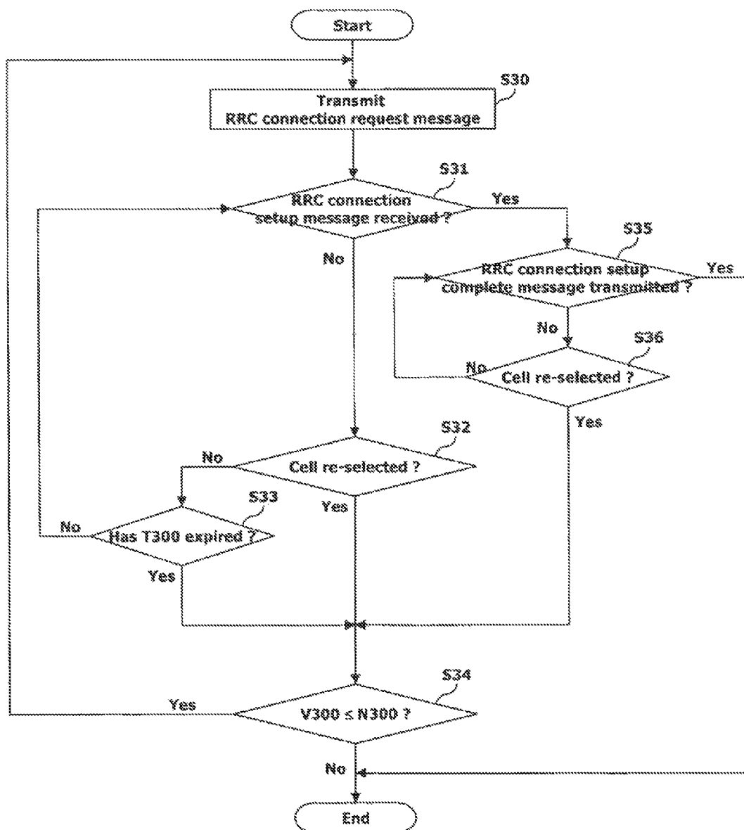
FIG. 5 Related Art
