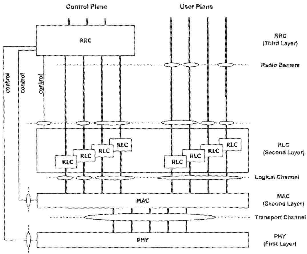
FIG. 2 Related Art
