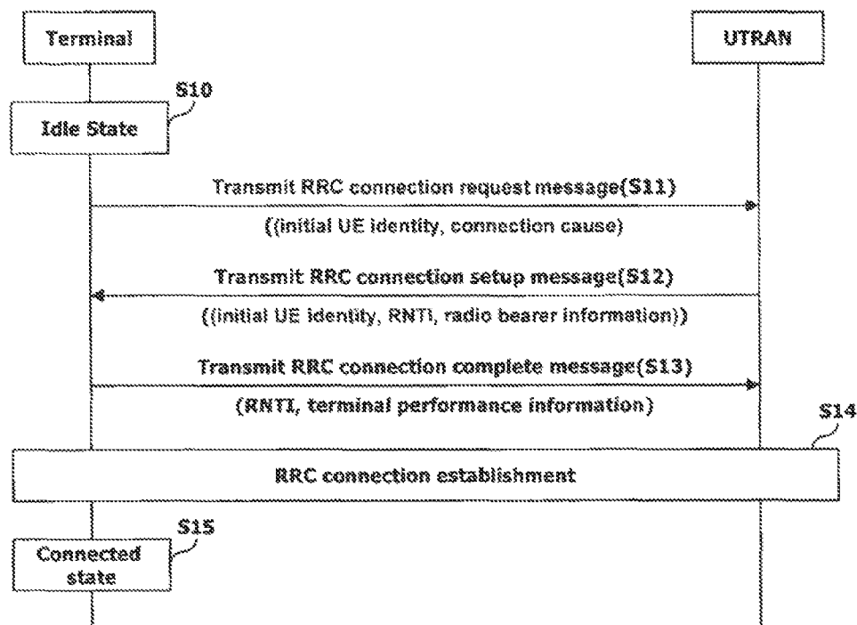
FIG.4 Related Art
