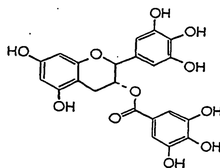
(-)-Gallocatechin gallate ((-)-GCg),
