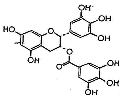
(-)-Epigallocatechin gallate ((-)-EGCg),
