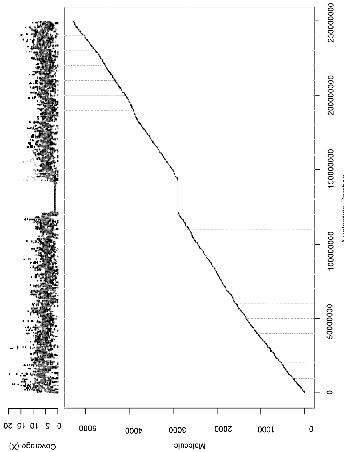
Figure 7A Coverage Distribution for Chromosome 1
