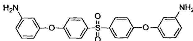
bis(4-(3-aminophenoxy)phenyl)sulfone, and
