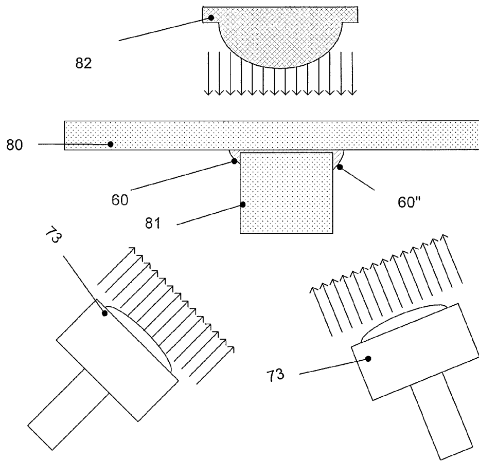
FIG. 32. Additional UV energy added to cure fillets
