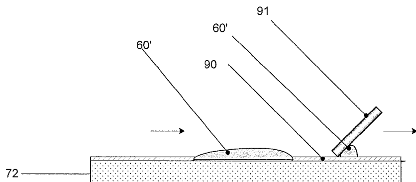
FIG. 30B- Position of the blade post screen printing
