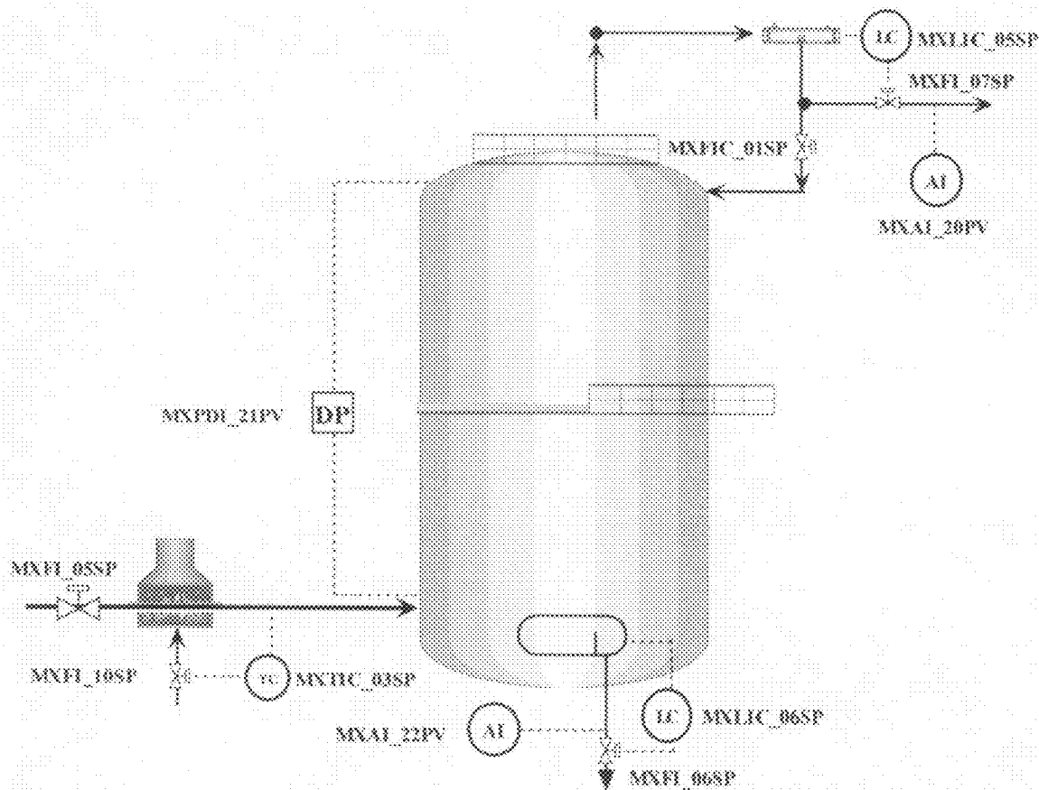
DeEthanizer Schematic Process Flow Diagram
