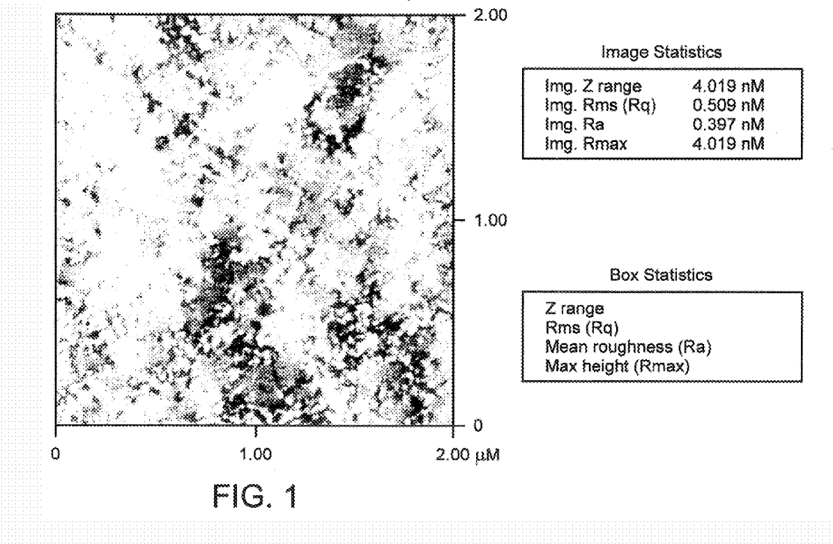
Photograph of atomic force microscope of Example 1-16
