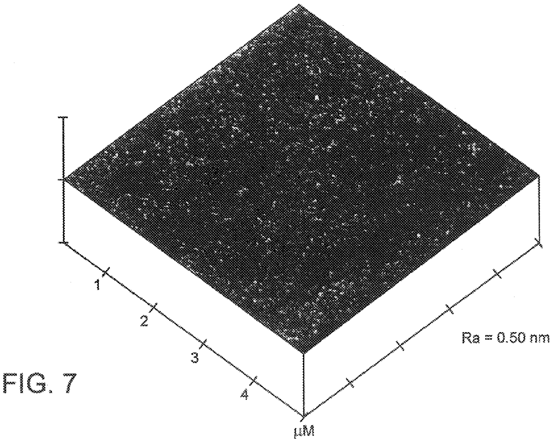
Photograph of atomic force microscope of Example 4 - 4
