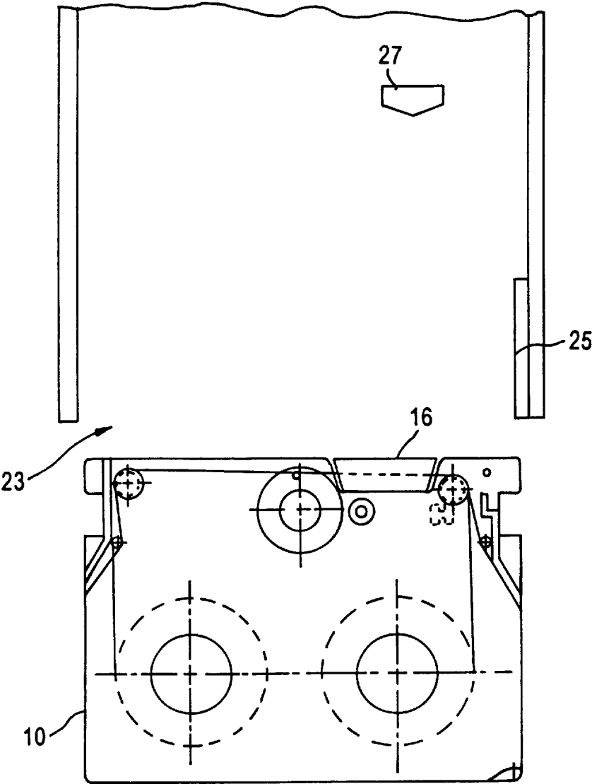
Figure 3 (PRIOR ART)
