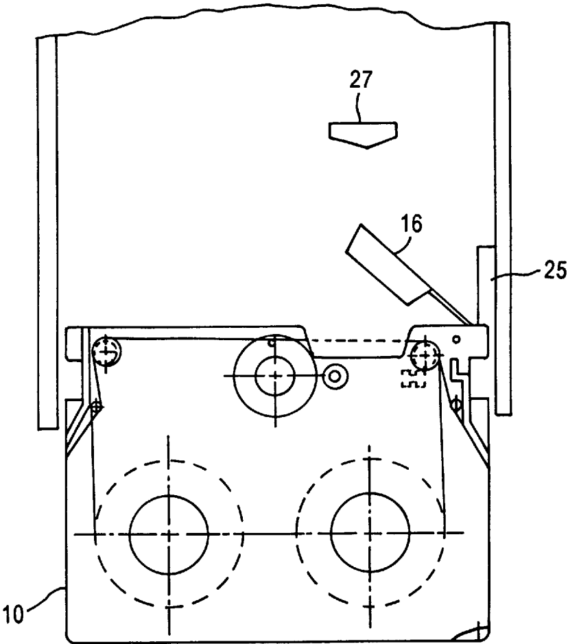
Figure 4 (PRIOR ART)
