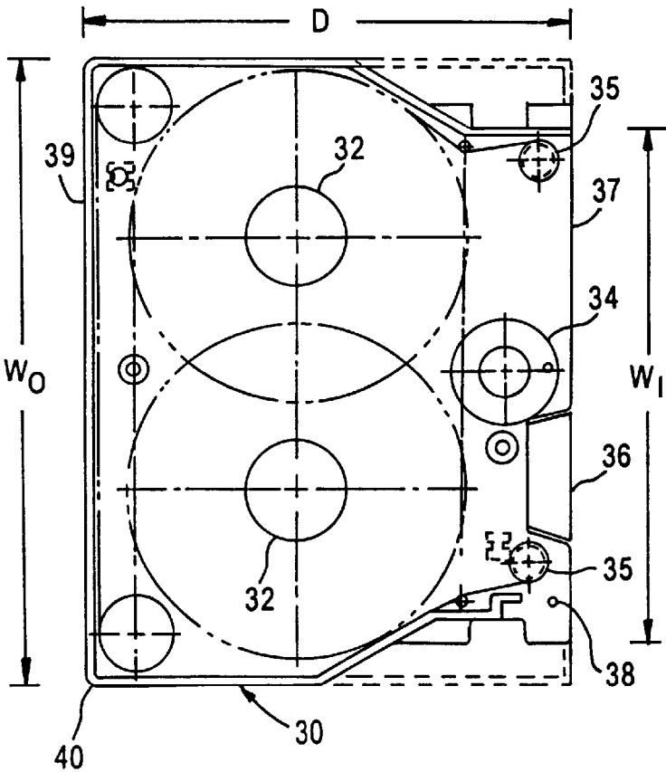
Figure 2 (PRIOR ART)
