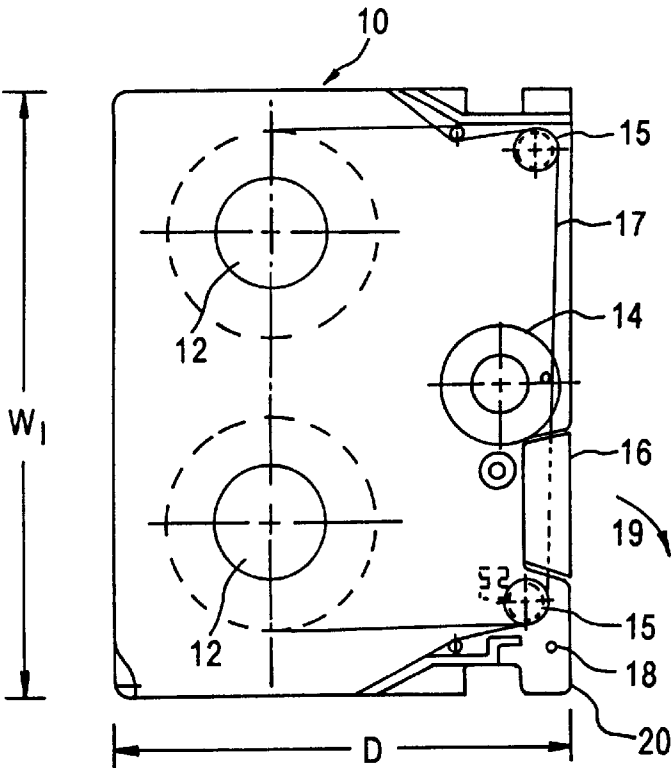
Figure 1 (PRIOR ART)
