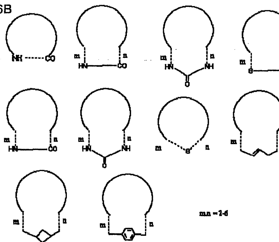
Scheme 2. Cyclization strategies:
