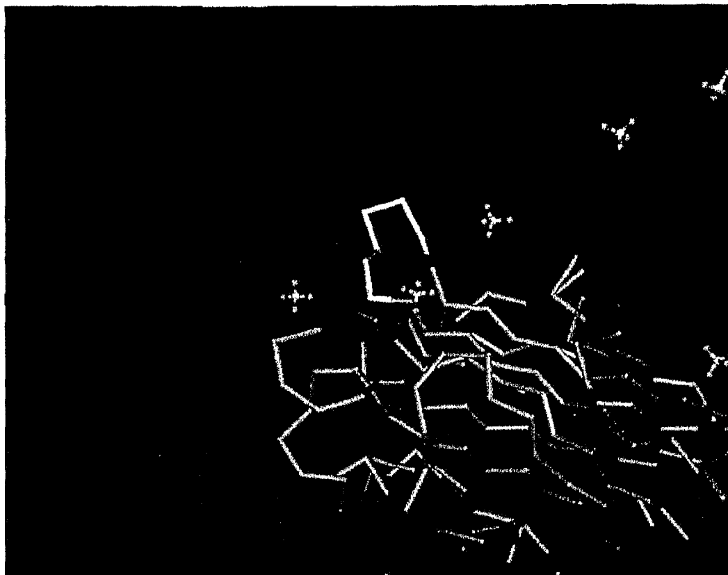
Figure 1: 1GWY Chain A, Crystal Structure Of The Water-Soluble Pore-Forming Cytotoxin Stictholysin II
