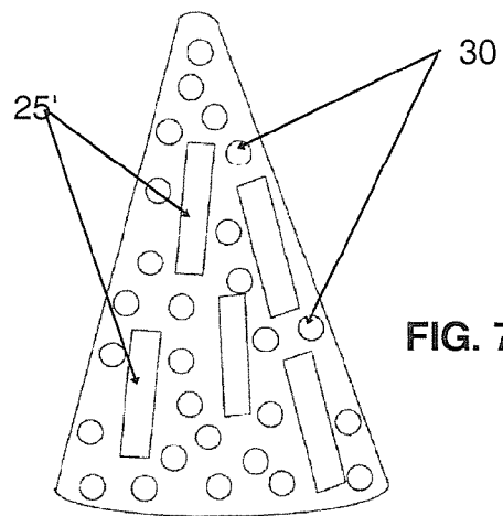
Curved Cone
