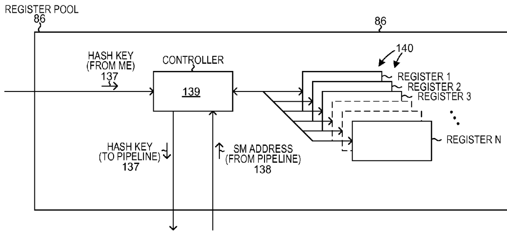
REGISTER POOL FIG. 17
