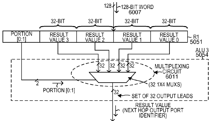
DIRECT 32-BIT LOOKUP STAGE FIG. 42
