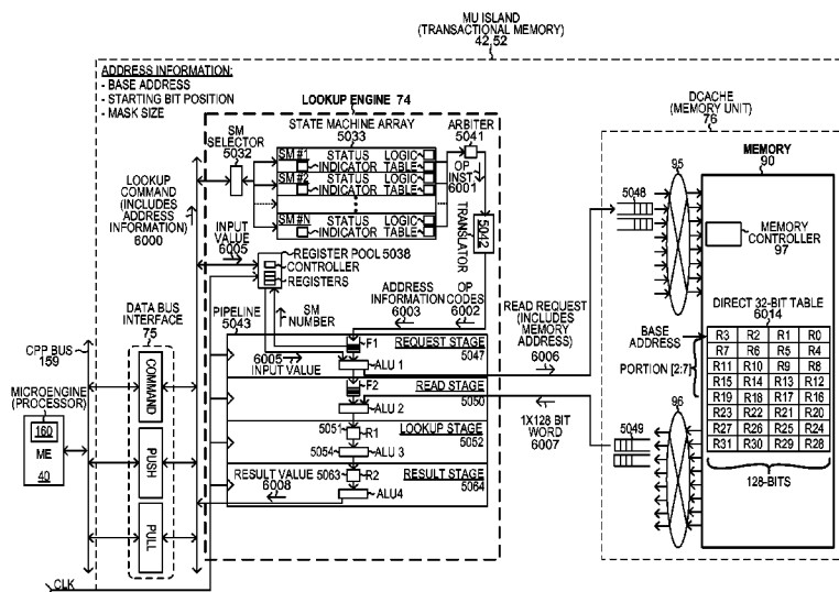
MU ISLAND SHOWING LOOKUP ENGINE PERFORMING DIRECT 32-BIT LOOKUP IN DETAIL
