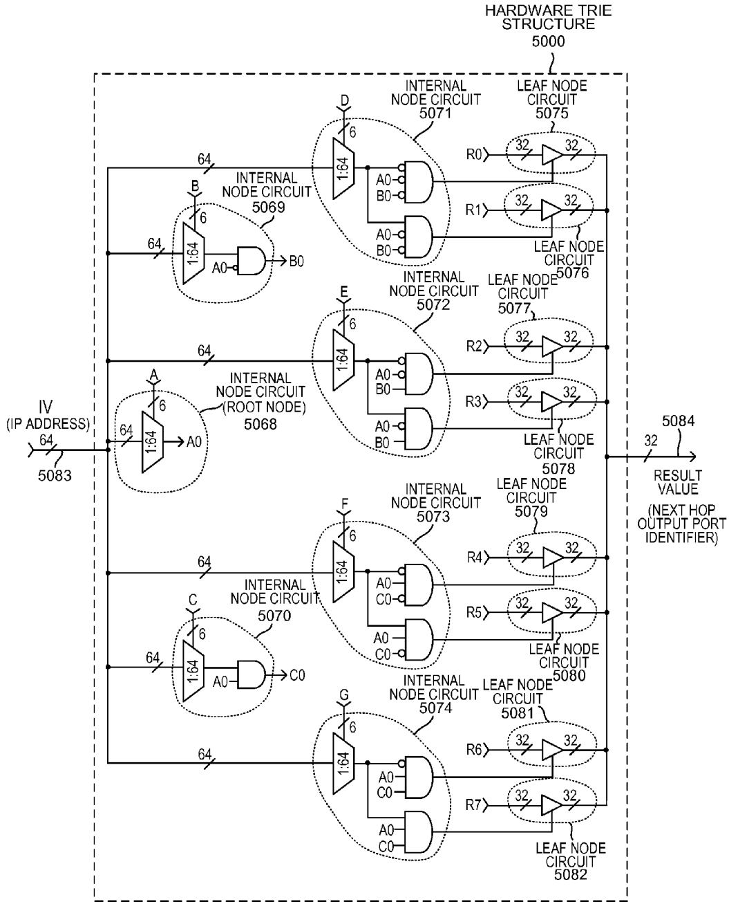
HARDWARE TRIE STRUCTURE FIG. 36
