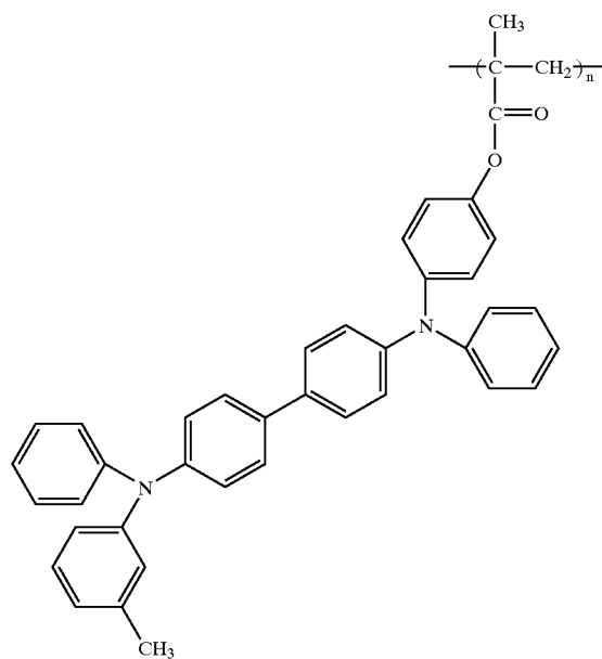
TPD-PMMA
