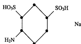
4-aminobenzene-1,3-disulphonic acid sodium salt (M-3)
