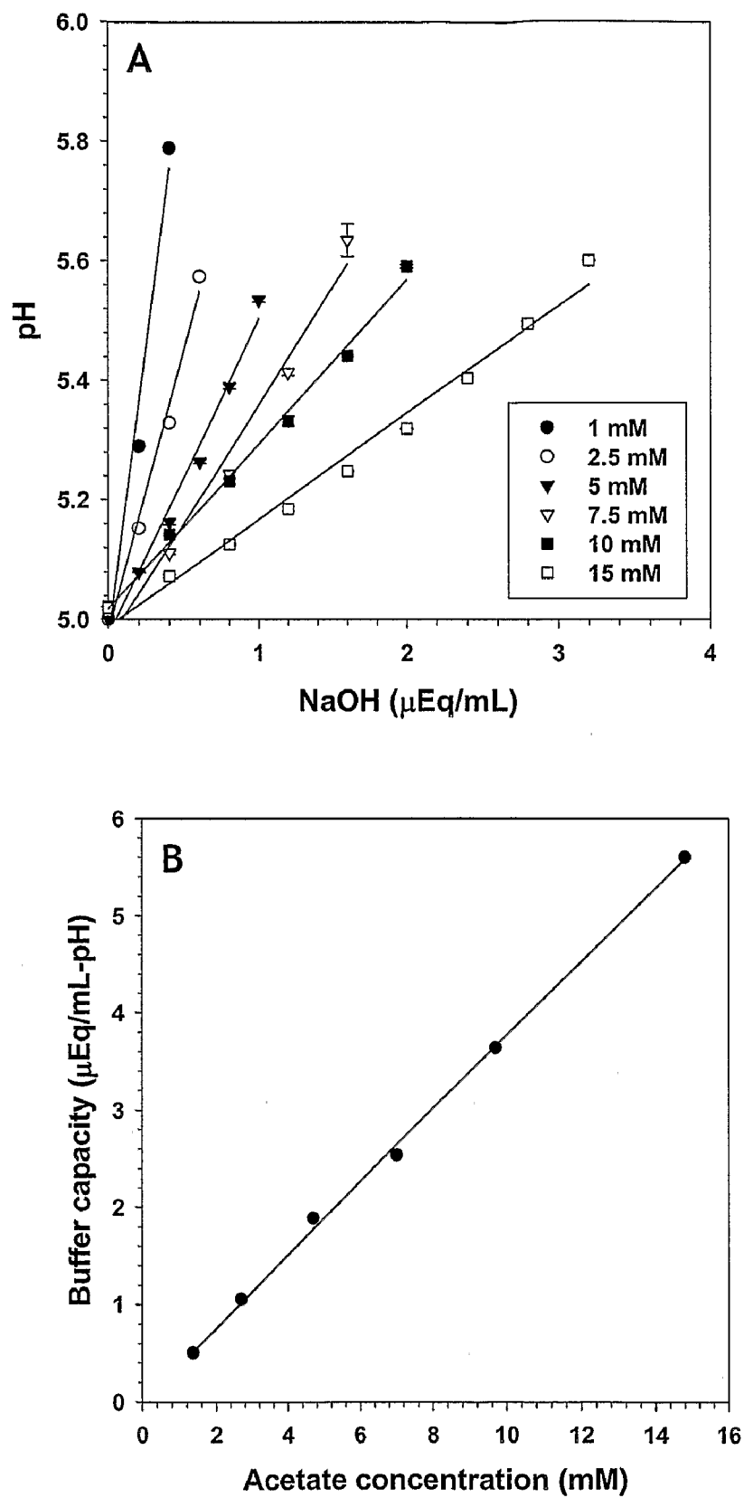
Figure 2. Buffer Capacity of Acetate in the pH 5.0 – 5.5 Range
