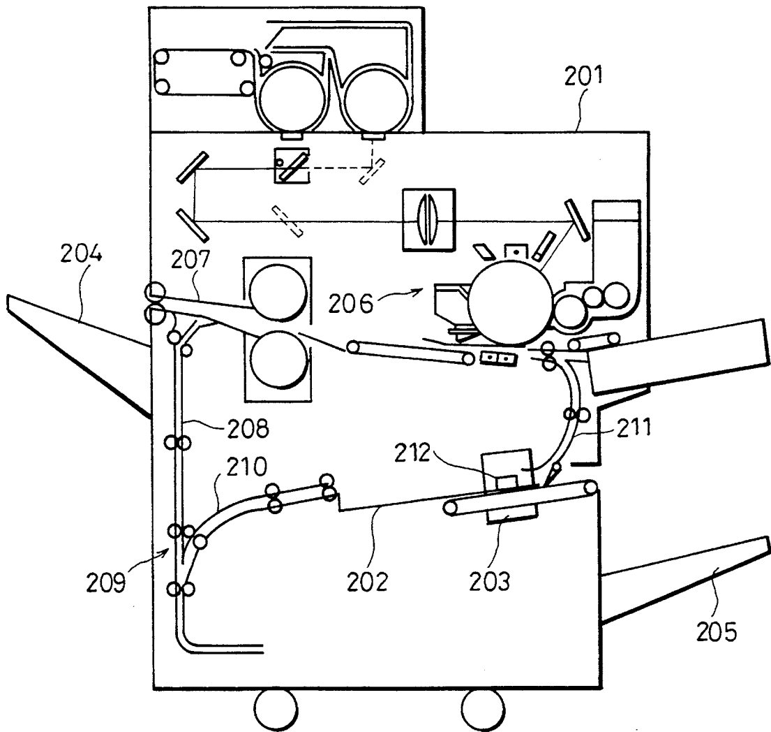
FIG. 19 (PRIOR ART)
