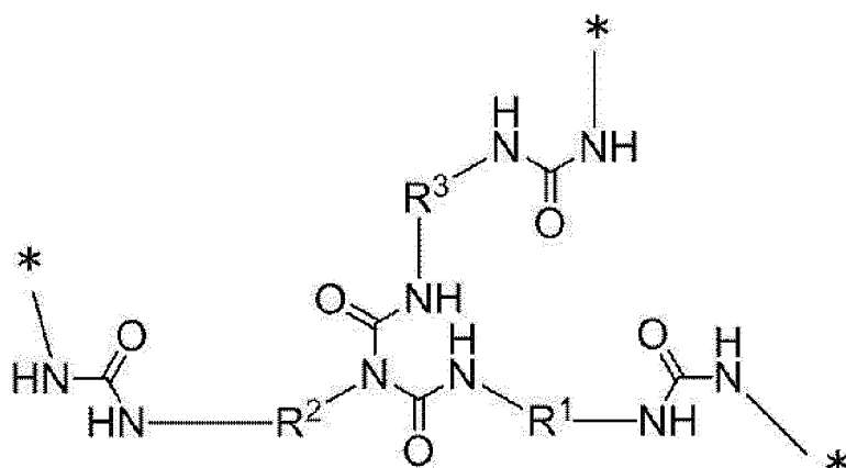
Structure (4)
