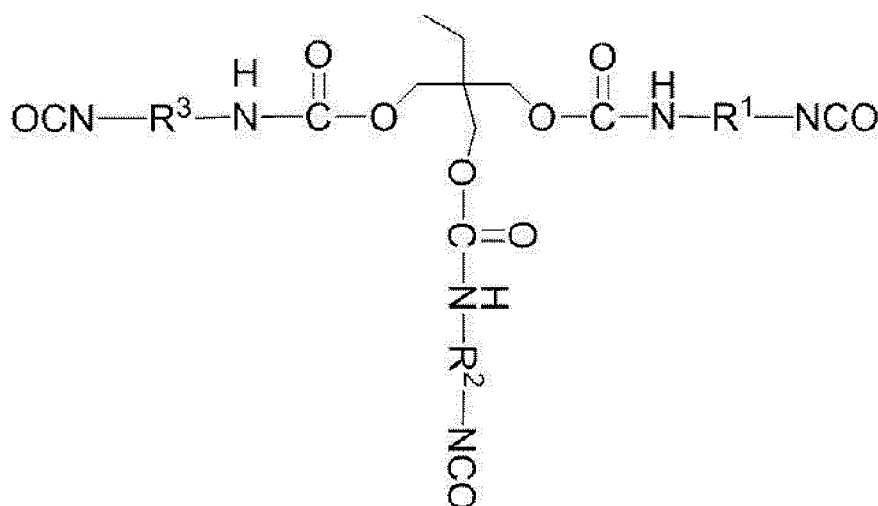
Formula (11A-1)
