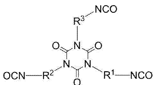
Formula (11C)
