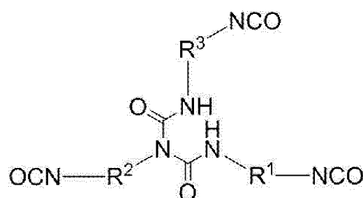
Formula (11D)
