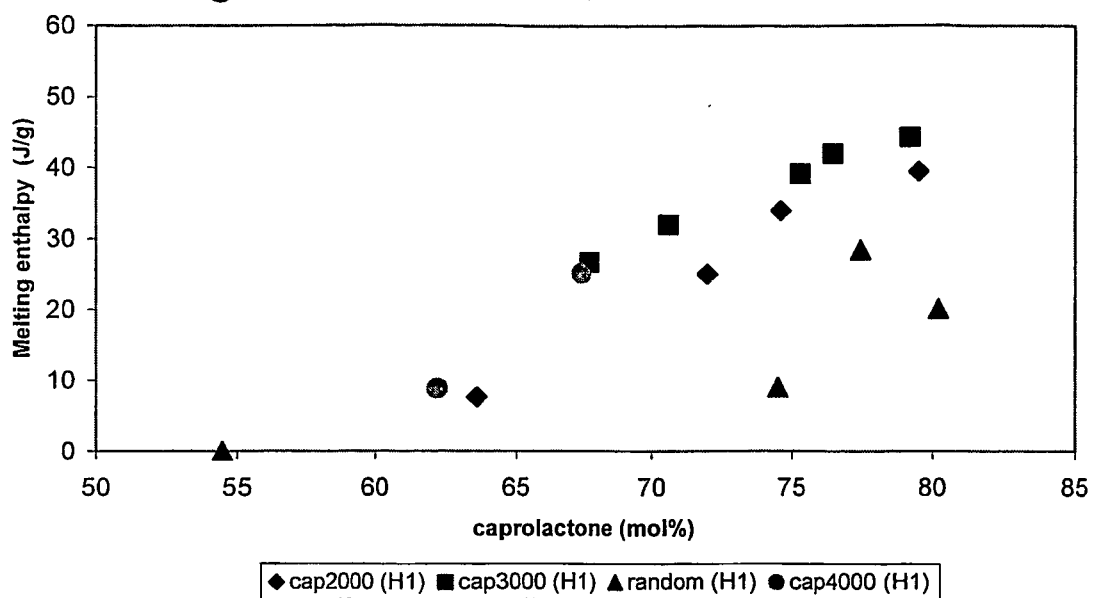
Figure 4: Melting enthalpy vs caprolactone content
