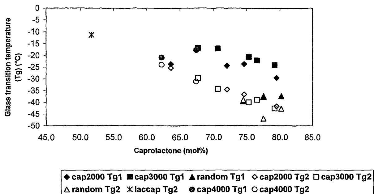
Figure 2: Glass transition temperature vs caprolactone content
