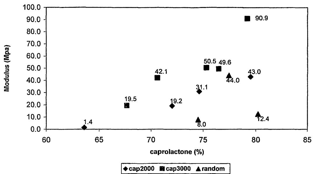
Figure 8: Modulus vs caprolactone content
