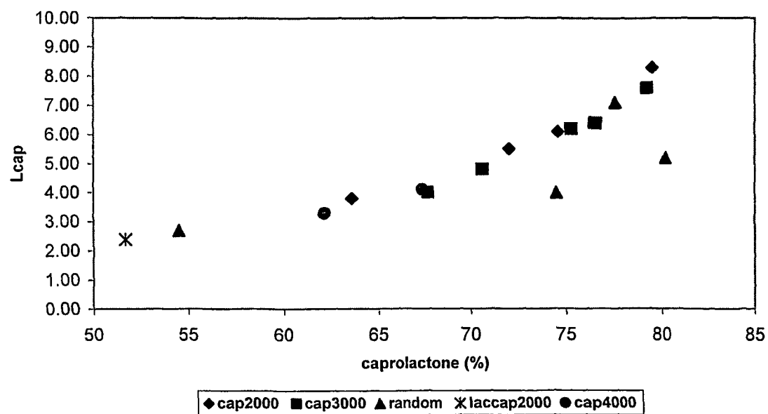
Figure 6: Average caprolactone sequence length vs caprolactone content
