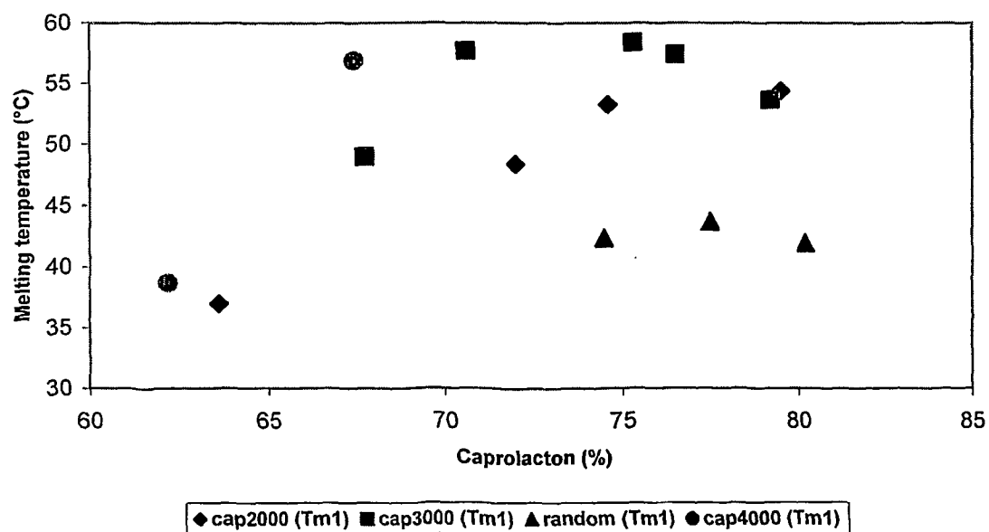
Figure 3: Melting temperature vs caprolactone content
