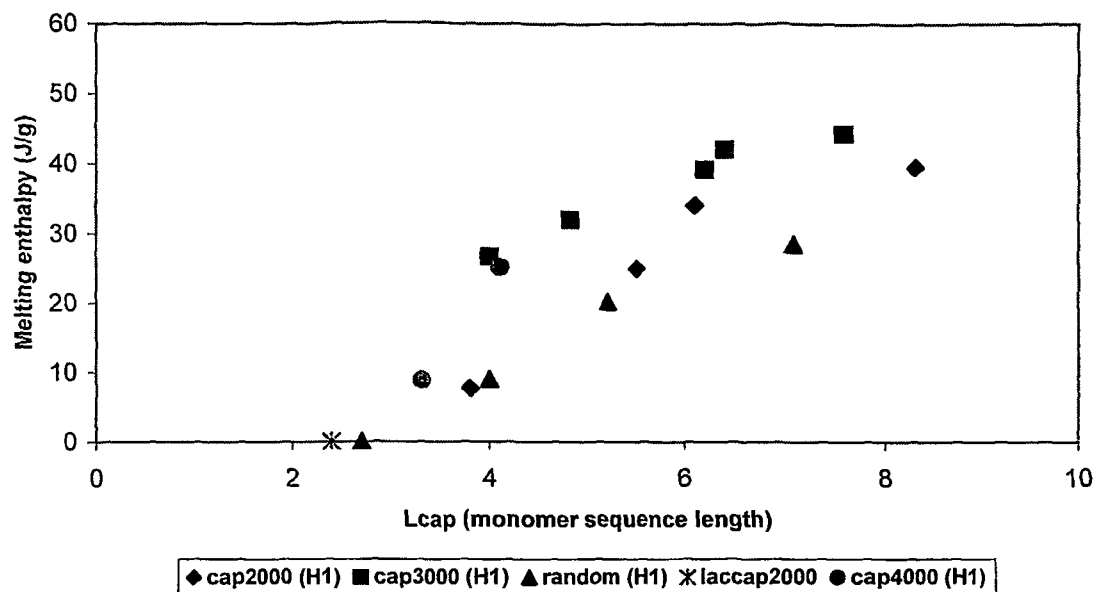
Figure 5: Melting enthalpy vs average caprolactone sequence length
