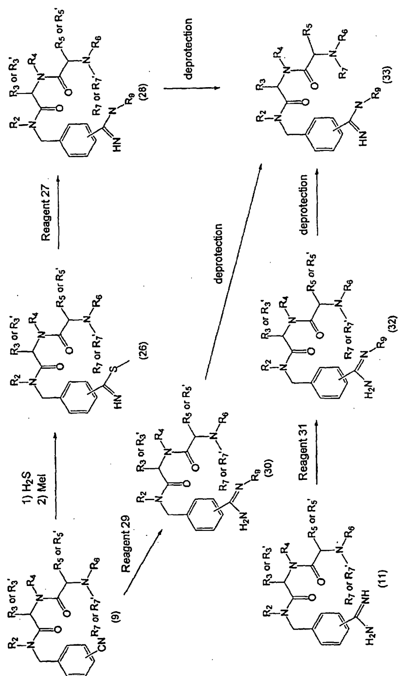
Reaction Scheme 4
