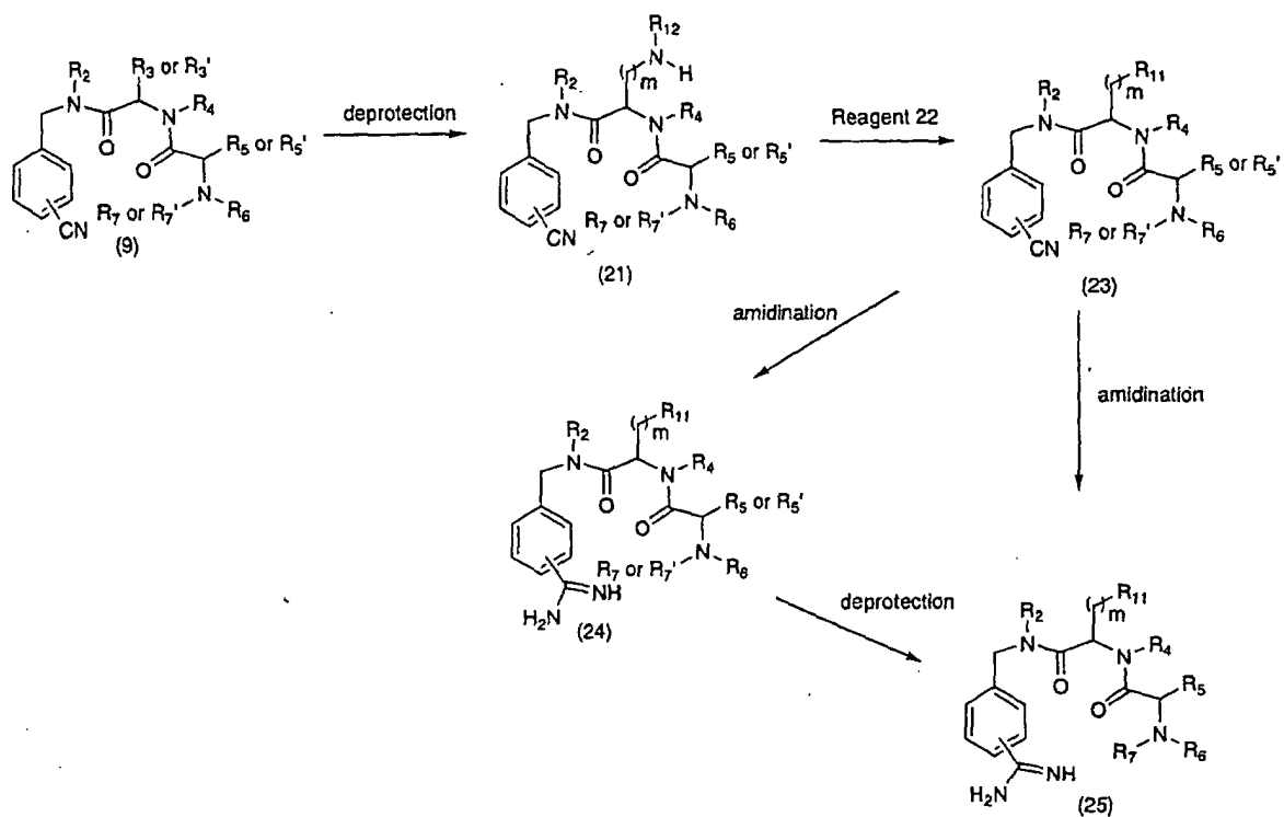
Reaction Scheme 3
