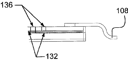
FIGURE 3C. DETAIL F
