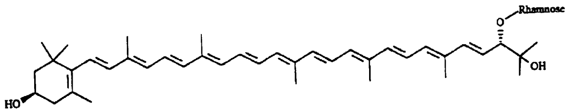
Myxoxanthophyll
