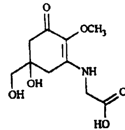
Mycosporine - Gly
