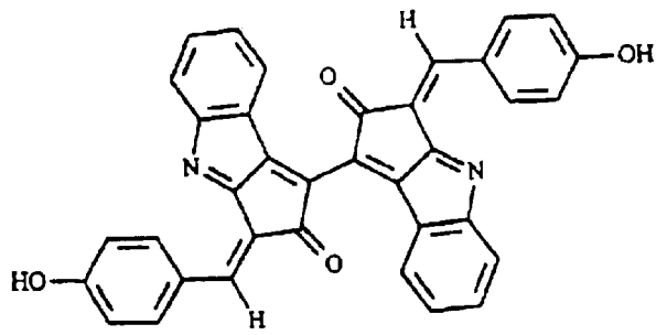
Scytonemin
